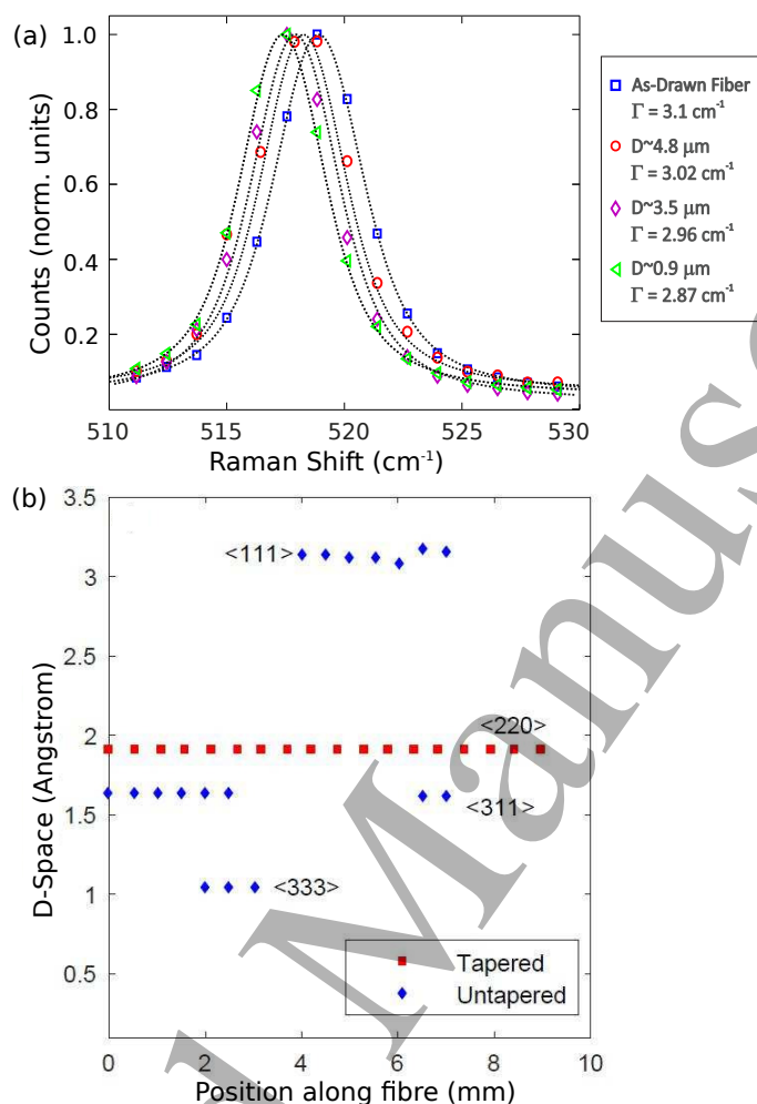
Figure 5. (a) Raman spectra for the silicon-core material taken for the as-drawn fibre and at the tapered waist sizes given in the legend. The dash curves are Voigt fits and the corresponding Lorentzian linewidths are given in the legend. (b) Lattice spacing of diffraction spots measured via XRD as a function of position along a section of the as-drawn fibre (blue) and tapered waist (red). Different d-spacings correspond to different crystallographic planes, as labelled.
