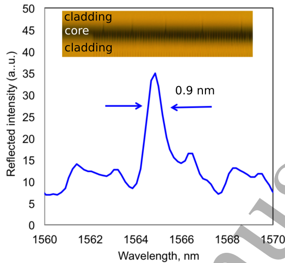
Figure 9. The reflected spectrum from a Bragg grating produced in a silicon optical fibre with a 517 nm femtosecond laser. Inset is on optical microscope image of the inscribed section of fibre.
