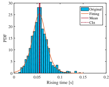
(c) Rising time T_r
