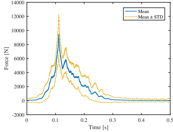
Figure 17: Representative mean wave slamming force time series and its standard deviation.
