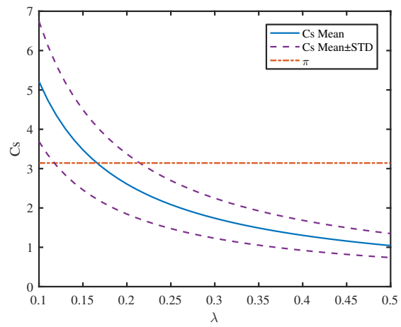
Figure 19: C_s under different \lambda values.
