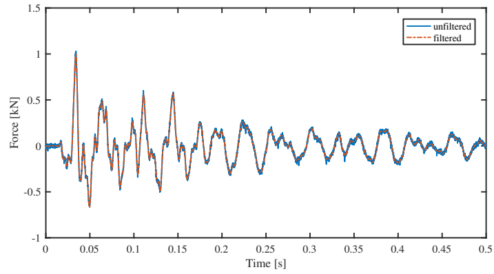
Figure 3: Comparison of unfiltered and filtered forces measured by one transducer.
