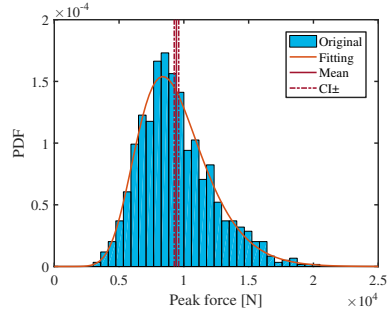
(a) Peak force F_p
