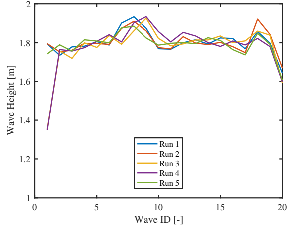
Figure 9: Wave height variation over different runs and waves.
