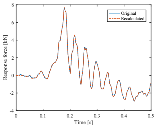
Figure 7: Comparison of original and recalculated response forces.
