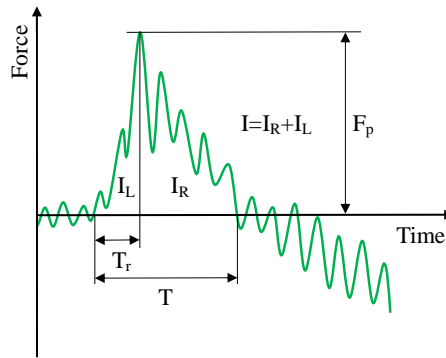
Figure 11: Parameters to describe one wave slamming force time series. The variation of the time series has been exaggerated for visualization purposes.
