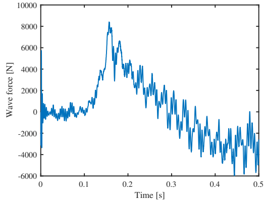
Figure 8: Estimated wave slamming force.
