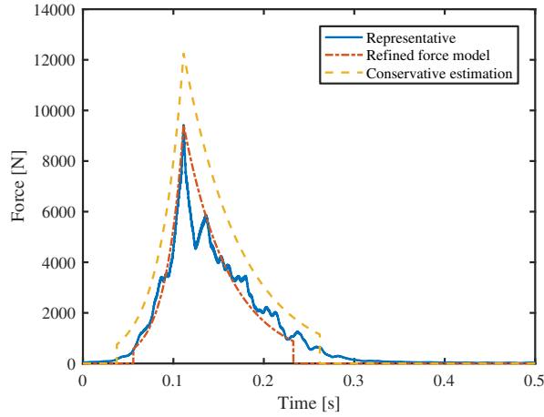
Figure 21: Refined force model for the representative wave slamming force time series.
