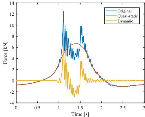
Figure 5: Separation of quasi-static and dynamic parts in a total response force.
