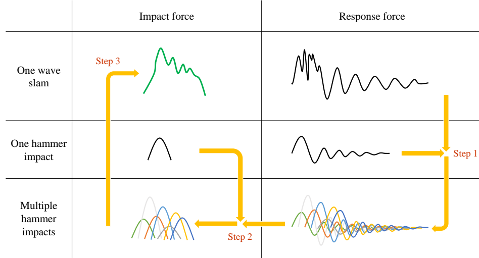
Figure 6: Illustration of the force reconstruction method.
