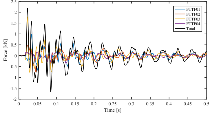
Figure 4: Summation of the forces measured by four transducers.
