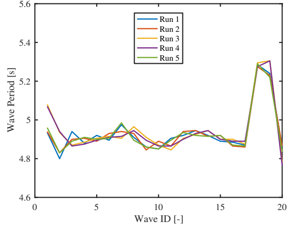
Figure 10: Wave period variation over different runs and waves.
