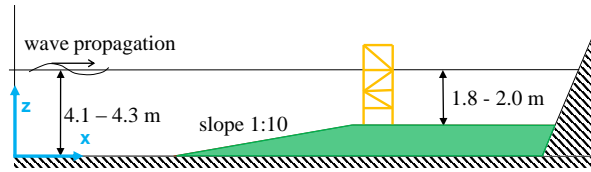
Figure 1: Experimental setup and global coordinates.
