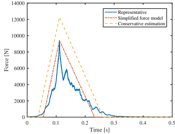
Figure 20: Simplified force model for the representative wave slamming force time series.
