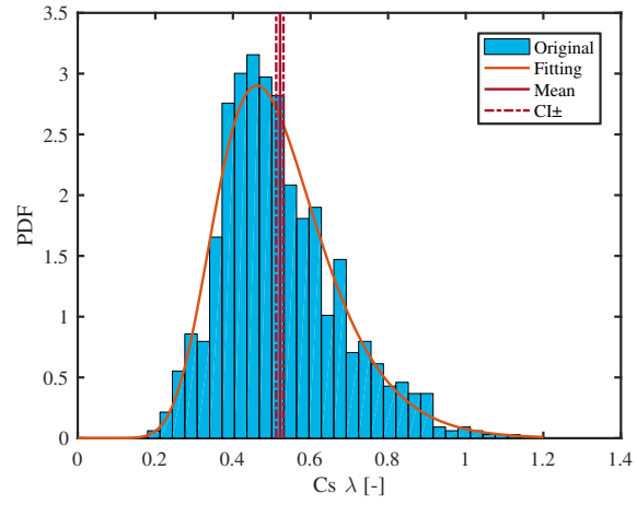
Figure 18: Statistical properties of C_s\lambda , represented by histogram, Gumbel distribution fit, mean and confidence interval of the mean.
