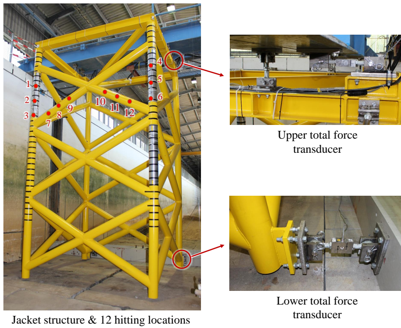
Figure 2: Jacket structure, hammer hitting locations and total force transducers. Figures reprinted with permission from the WaveSlam project.
