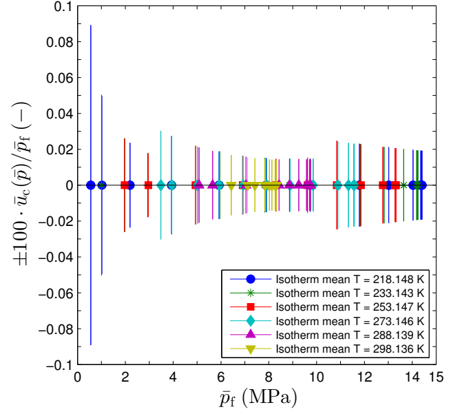
Fig. 2. Pressure standard uncertainty relative to the measured pressure for the VLE measurements performed, expressed as 100 \cdot \tilde{u}_c(\bar{p})/\bar{p}_f . Measured pressure \bar{p}_f . Standard uncertainty \tilde{u}_c(\bar{p}) .
