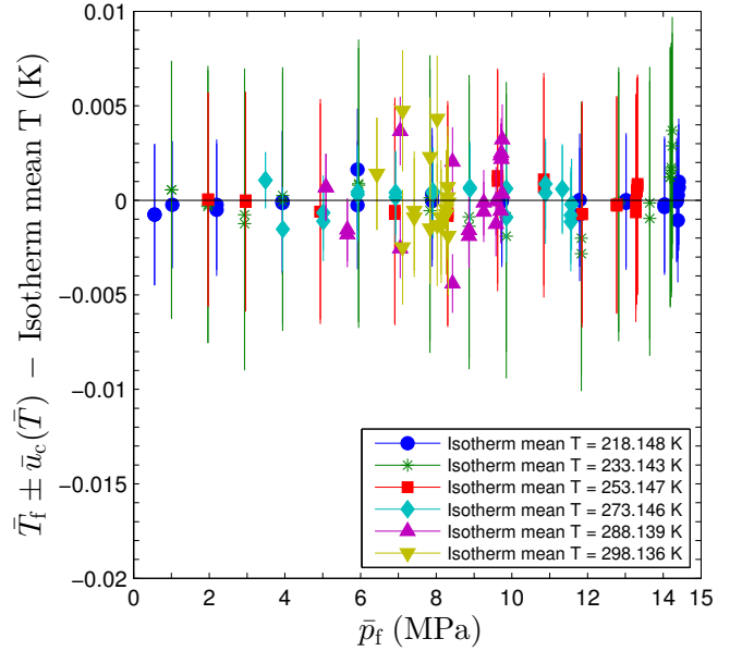
Fig. 3. Temperature deviations for each VLE measurement from isotherm mean temperature, and temperature standard uncertainty, expressed together as \bar{T}_f \pm \tilde{u}_c(\bar{T}) - \text{isotherm mean temperature} , versus VLE experiment pressure \bar{p}_f . VLE experiment mean temperature \bar{T}_f . Temperature standard uncertainty \tilde{u}_c(\bar{T}) .
