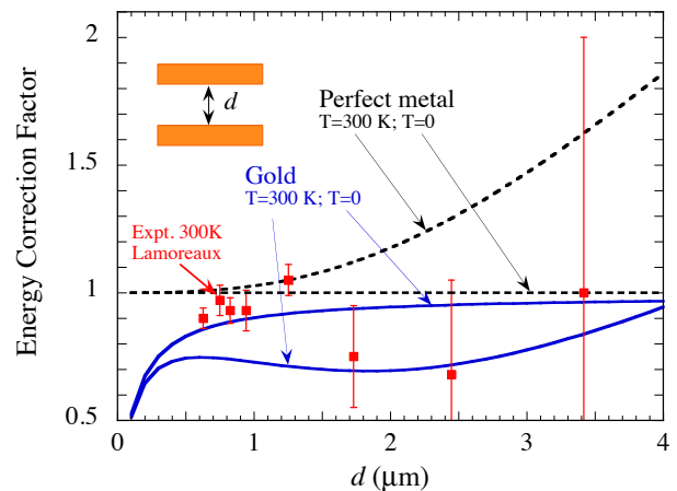
Figure 1. Energy correction factor for two gold plates in the absence of any intervening plasma. The filled squares with error bars are the Lamoreaux's experimental [16] values from the torsion pendulum experiment. The dashed curves are the perfect metal results. The thick solid curves are the results for real gold plates at zero temperature and at room temperature [17]. The dielectric properties for gold was obtained from tabulated experimental optical data.
