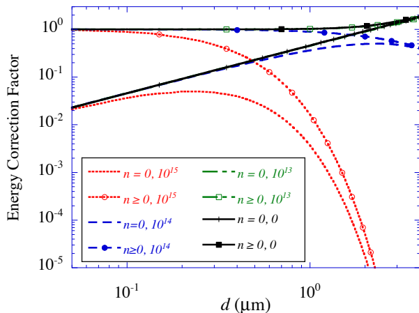
Figure 2. Energy correction factor for two perfect metal plates interacting across a plasma. The curves are the results for perfect metal plates at room temperature for different plasma frequencies ( \omega_p in units of rad/s) for the intervening plasma. We show the results for the n = 0 and n \geq 0 contributions to the interaction free energy.
