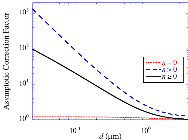
Figure 3. Asymptotic correction factor for two perfect metal plates interacting across a plasma ( \omega_p = 10^{14} \text{ rad/s} ). The results show the ratio between numerically calculated energies and the corresponding asymptotes given in the text. There is very good agreement (ratio close to one) for the n = 0 contribution in the entire range considered. For n > 0 and n \geq 0 the curves go towards one at large surface separations. Note that the asymptotes become more accurate for higher plasma densities.
