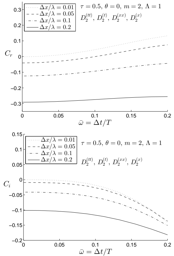
FIGURE 9. Downstream waves dispersion and damping (forward speed and oscillations) for different \Delta x/\lambda ratio with second order finite difference operator for spatial and time derivatives. \tau = U\omega/g , \theta : wave propagation direction, C_r : dispersion, C_i : damping, \Lambda = \Delta y/\Delta x : element aspect ratio.
