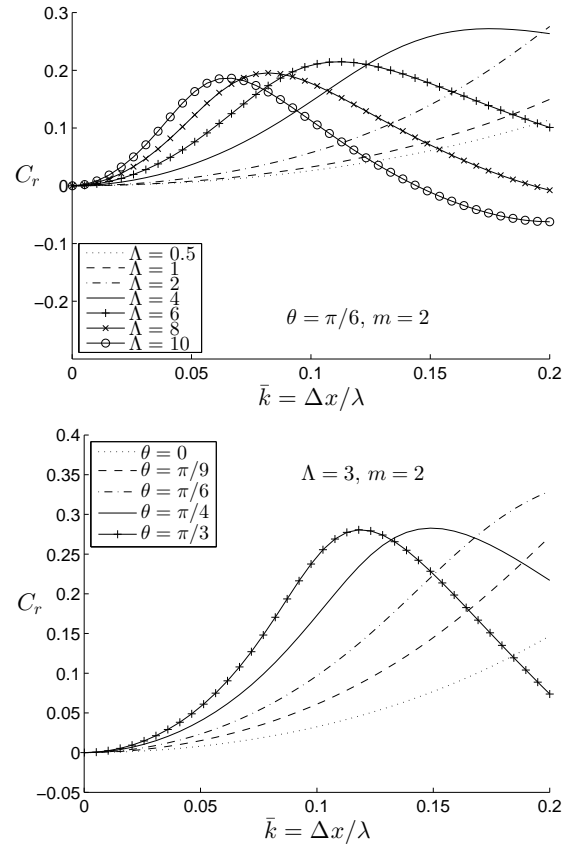
FIGURE 5. Dispersion and damping (steady forward speed) for surface discretization only, different wave propagation directions \theta and element aspect ratio \Lambda . linear elements ( m = 2 ), element aspect ratio \Lambda = \Delta y / \Delta x . C_r : Dispersion, \theta : wave propagation direction. \lambda : Wave length.
