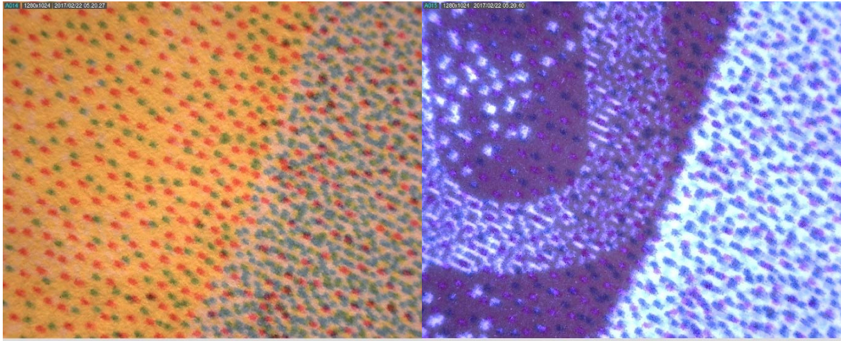
Figure 4. A different image viewed under the microscope. The image under daylight (left) shows the microstructure of an edge area and the UV illumination (right) shows the identical area. The letter “U” which is part of the binary pattern is clearly visible.
