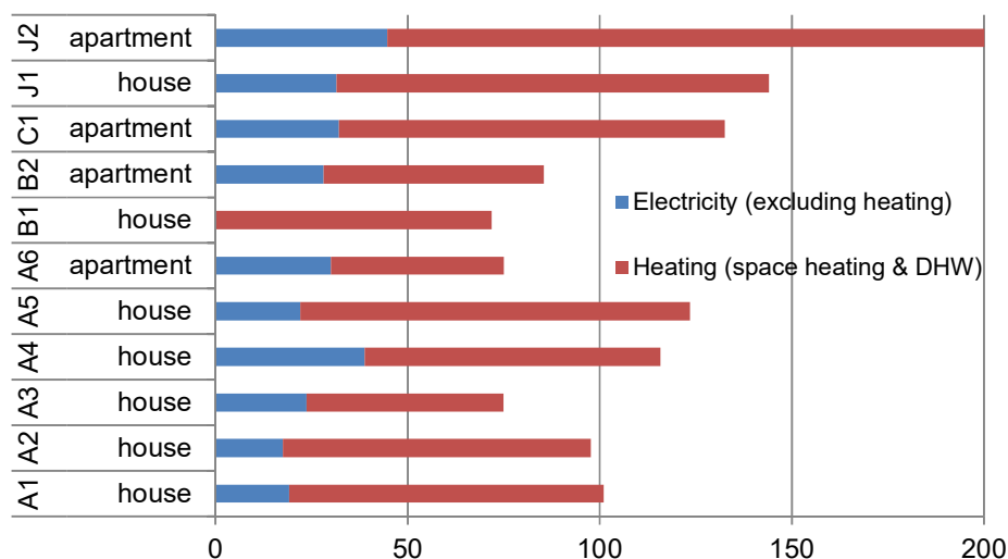
Figure 8 Electricity and heating energy use of residential case study buildings (Unit: kWh/(m 2 .a))
