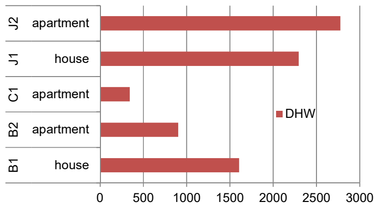
Figure 9 DHW energy consumption indicator of residential case buildings (Unit: kWh/(ca.a))
