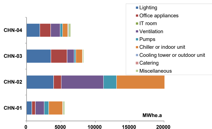
Figure 7 Total electricity use for the office buildings larger than 30000 m 2
