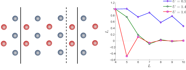
FIG. 1: Left panel : A model of the Josephson junction in (110)-direction. Red (blue) dots denote the A (B)-lattice. The dashed vertical line is the interface for an even junction, while the right solid line is the interface for an odd junction. The left solid line is the same for both even and odd junctions. Right panel : Critical current as a function of length L for different values of the magnetic coupling constant U . The data are normalized to the L = 4 value to simplify comparison. We have used V = 1.9 .
