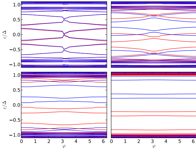
FIG. 3: (Color online) Energy-levels of current-carrying states of the system as a function of superconducting phase-twist across the junction. Red lines denote spin-up states, blue lines denote spin-down states. As the strength of the antiferromagnetic ordering increases ( U increases), spin-down states are lowered in energy by the Zeeman-effect due to the uncompensated spin, while spin-up states increase in energy. Upper left panel: U = 0.5 . Upper right panel U = 1.2 . Lower left panel: U = 1.545 . Lower right panel: U = 2.0 . The contributions to the current are essentially determined by the \phi -derivative of each of the curves. As the levels cross, the levels contributing most significantly to the current changes sign, leading to the 0 - \pi transition. This requires a threshold value, unlike in the ferromagnetic case. Other parameter values are: V = 1.9 , \mu = 0 , L = 5 .
