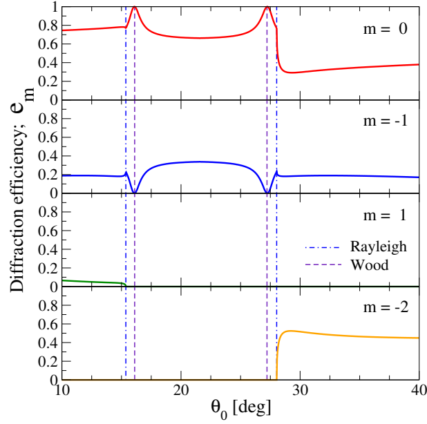
FIG. 3. The diffraction efficiencies e_m(\theta_0) , Eq. (19), as functions of the angle of incidence for a lamellar grating defined by a/d = 0.40 and h/d = 0.30 . The angular positions of the Rayleigh and Wood anomalies, determined by Eqs. (30) and (32), respectively, are indicated by vertical dashed-dotted and dashed lines, respectively. Only diffracted orders m for which e_m(\theta_0) \neq 0 in the range of \theta_0 considered are presented. The wavelength of the incident light assumed in obtaining these results was \lambda/d = 0.7350 . The point on the dispersion curve for this grating corresponding to this wavelength is indicated by arrows in Fig. 2. The numerical calculations were done for M = 10 .
