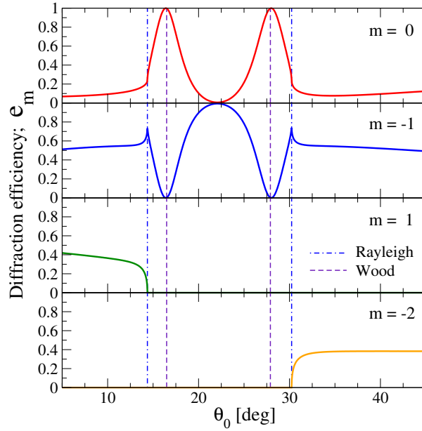
FIG. 5. The same as Fig. 3, but now for a grating defined by a/d = 0.45 and h/d = 0.20 . The wavelength of the incident light is \lambda/d = 0.7518 (indicated by the arrows in Fig. 4).
