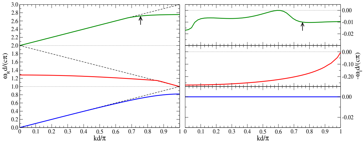
FIG. 2. The dispersion curves for the surface electromagnetic waves supported by a lamellar perfectly conducting grating defined by a/d = 0.40 and h/d = 0.30 . Both the real, \omega_R(k) , and imaginary, -\omega_I(k) , parts of the frequency [\omega(k) = \omega_R(k) - i\omega_I(k)] of these waves are presented in the reduced zone scheme. The first branch of the dispersion (blue line) is located in the nonradiative region of the (k, \omega) -plane, and it corresponds to a true surface wave, the imaginary part of whose frequency vanishes identically. The second and third branches of the dispersion curve (red and green lines, respectively) are both located in the radiative region ( |k| < \omega/c ); they correspond to leaky surface waves, whose frequencies have negative imaginary parts. The dashed (black) lines denote the vacuum light line in the reduced zone scheme. The arrows correspond to the wavelength \lambda/d = 0.7350 [ \omega d/c\pi = 2.7212 ] that will be used to calculate diffraction efficiencies in Fig. 3. The numerical calculations were done for M = 10 , but increasing this value, did not affect the final result.
