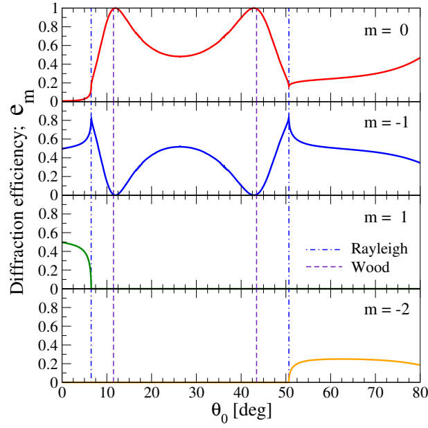
FIG. 7. The same as Fig. 3, but now for a grating defined by a/d = 0.60 and h/d = 0.20 . The wavelength of the incident light is \lambda/d = 0.8867 (indicated by the arrows in Fig. 6).
