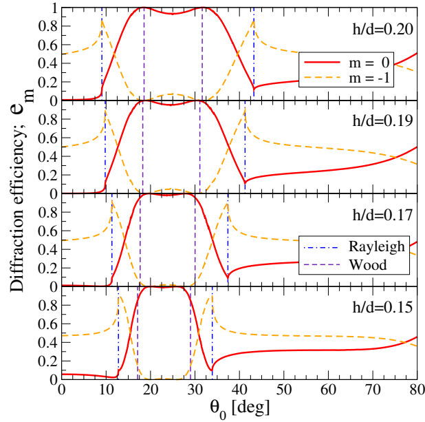
FIG. 8. The diffraction efficiencies, e_0(\theta_0) and e_{-1}(\theta_0) , as functions of the angle of incidence \theta_0 for a grating defined by a/d = 0.60 , and several values of h/d , as indicated on the figure. In obtaining these curves the value kd/\pi = 0.7551 was assumed.
