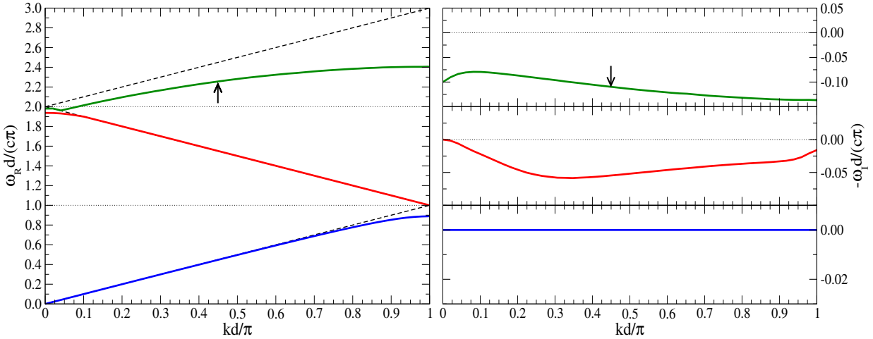
FIG. 6. The same as Fig. 2, but now for a grating defined by a/d = 0.60 and h/d = 0.20 . The arrows correspond to the wavelength \lambda/d = 0.8867 [ \omega d/c\pi = 2.2554 ], which will be used in calculating the diffraction efficiencies presented in Fig. 7.
