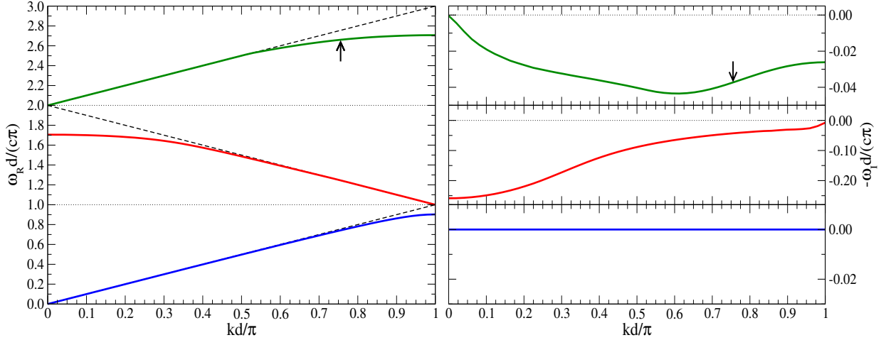
FIG. 4. The same as Fig. 2, but now for a grating defined by a/d = 0.45 and h/d = 0.20 . The arrows correspond to a wavelength \lambda/d = 0.7518 [ \omega d/c\pi = 2.660 ], which will be used in calculating the diffraction efficiencies in Fig. 5.
