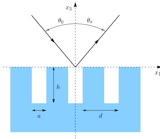
FIG. 1. A depiction of the grating considered in this work, the parameters that define it, and the geometry of the diffraction of light from it.
