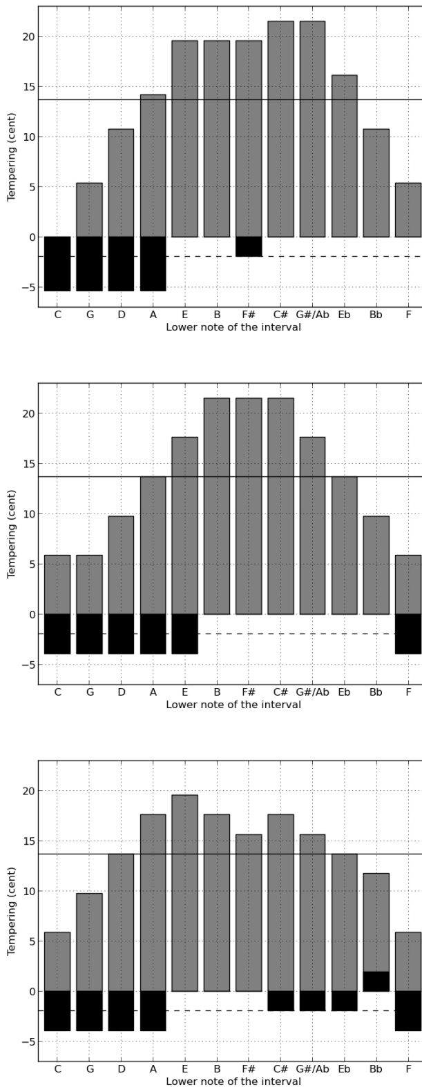
Figure 6. The tempering of fifths (black) and major thirds (grey) as measured in cent for well-known temperaments. Kirnberger III (top), Valotti (middle), and Lehman's Bach temperament (bottom). The solid and the dashed horizontal lines show the tempering of major thirds and fifths in equal temperament respectively.
