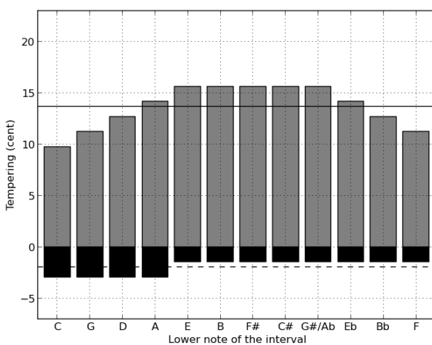
Figure 5. The tempering of fifths (black) and major thirds (grey) as measured in cent for the different choices of F_0 = -S/4 (top), F_0 = -P/6 (middle), and F_0 = -P/8 (bottom). The solid and the dashed horizontal lines show the tempering of major thirds and fifths in equal temperament respectively. See Section 2.4 for details.
