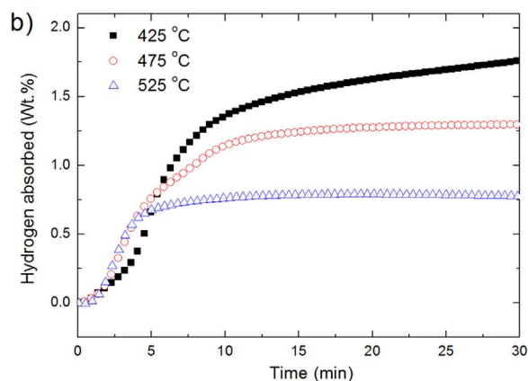
Fig. 4. Hydrogenation in Ar+10%H 2 after cycling in gas containing CO: a) Ti 0.9 V 0.1 , b) Ti 0.9 V 0.1 +nano Pd/Pt.
