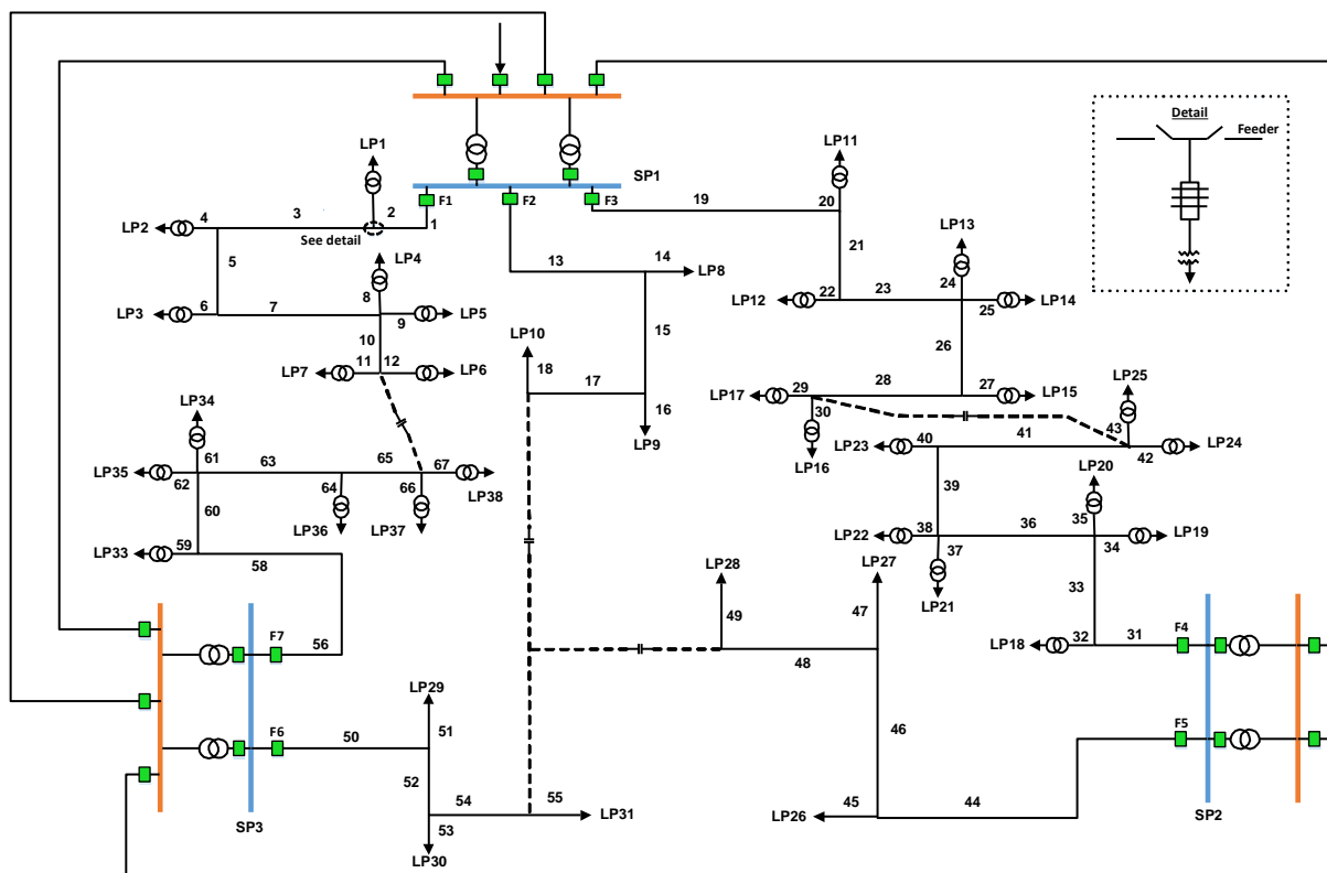
Fig. 3.8 Single diagram of RBTS Bus 4 distribution system [3]
