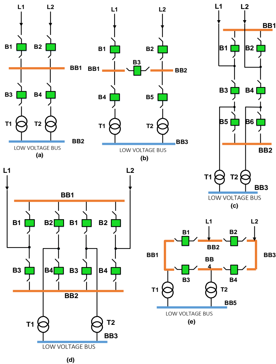
Fig. 4.1 Five distribution substation configurations (a: single bus, b: sectionalized single bus, c: breaker-and-a-half, d: double bus double breaker, e: ring bus) [2][14]
