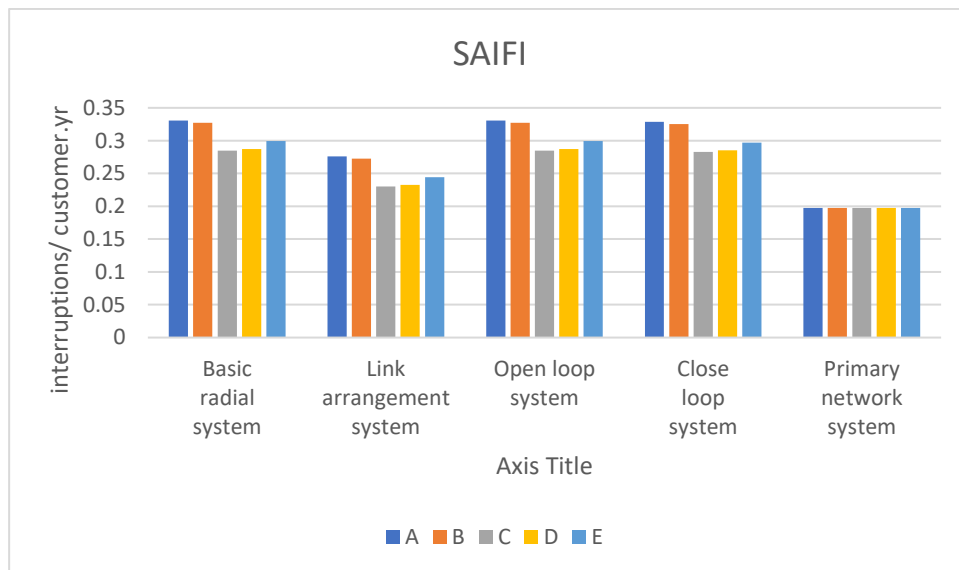
Fig. 4.9 Comparison of system reliability indice (SAIFI) for five distribution system
