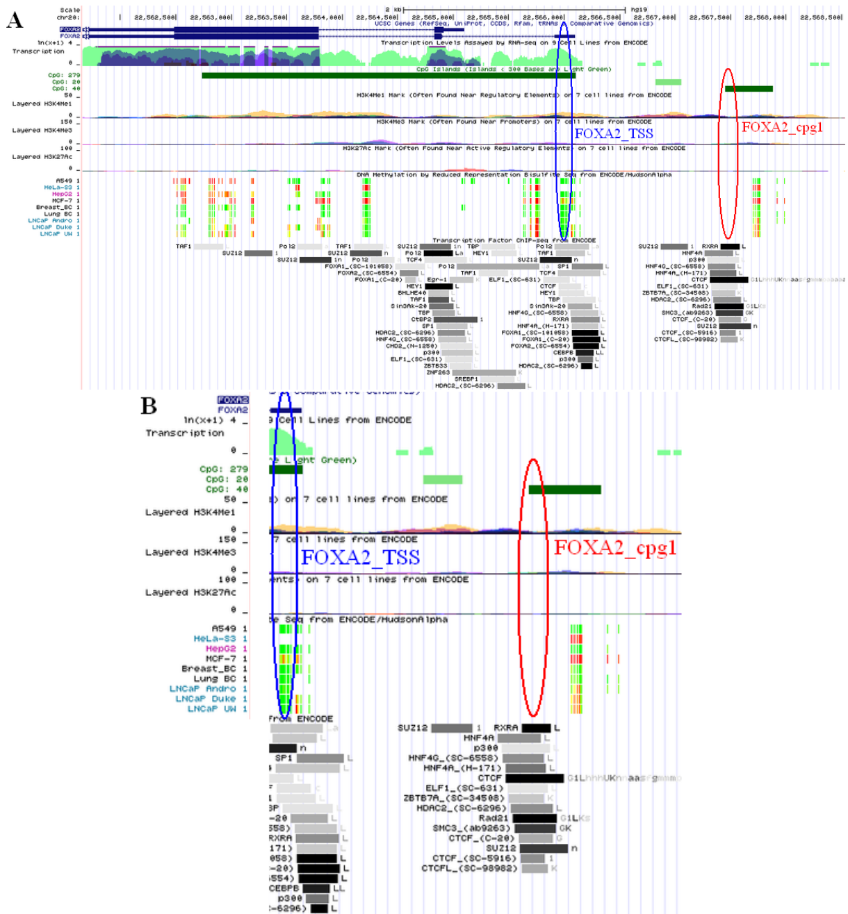
Figure 4.2: Localisation of FOXA2_cpg1 (red oval) and FOXA2_TSS (blue oval) assays represented by data from ENCODE (the gene, transcription levels, CpG islands (dark green lines), histone methylations, histone acetylation, methylation levels and transcription factor binding sites (grey)) is shown in A. In B there are zoomed in on the localisations of the assays. FOXA2_cpg1 is located upstream of the gene in a CpG island, whereas FOXA2_TSS lies around the promoter and also within a CpG island. DNA methylation is represented by red (100 % of molecule sequences are methylated), yellow (50 %) or green (0 %).
