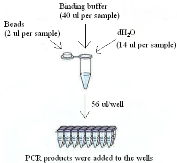
Figure 2.7: Immobilization of PCR products to Streptavidin Sepharose beads (PyroMark Q24 User Guide).
