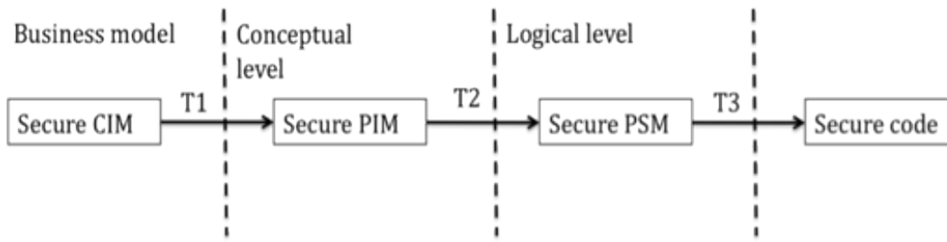
Fig. 2. Framework for designing secure Data Warehouses. Adapted from [32].
