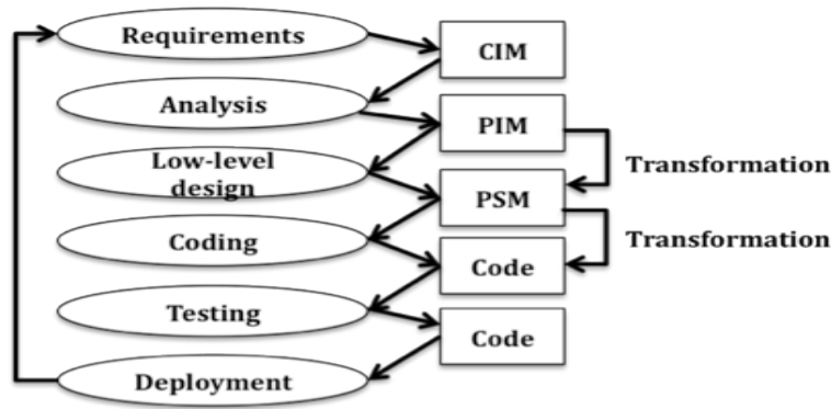
Fig. 1. MDA Software Development Lifecycle. Adapted from [1].
