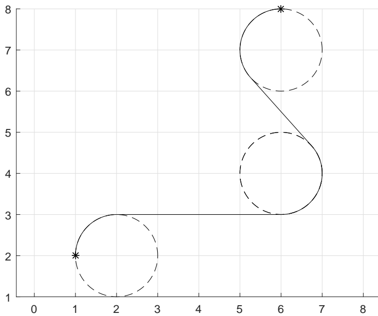
Figure 5.1: An illustration of a simple Dubins path.
