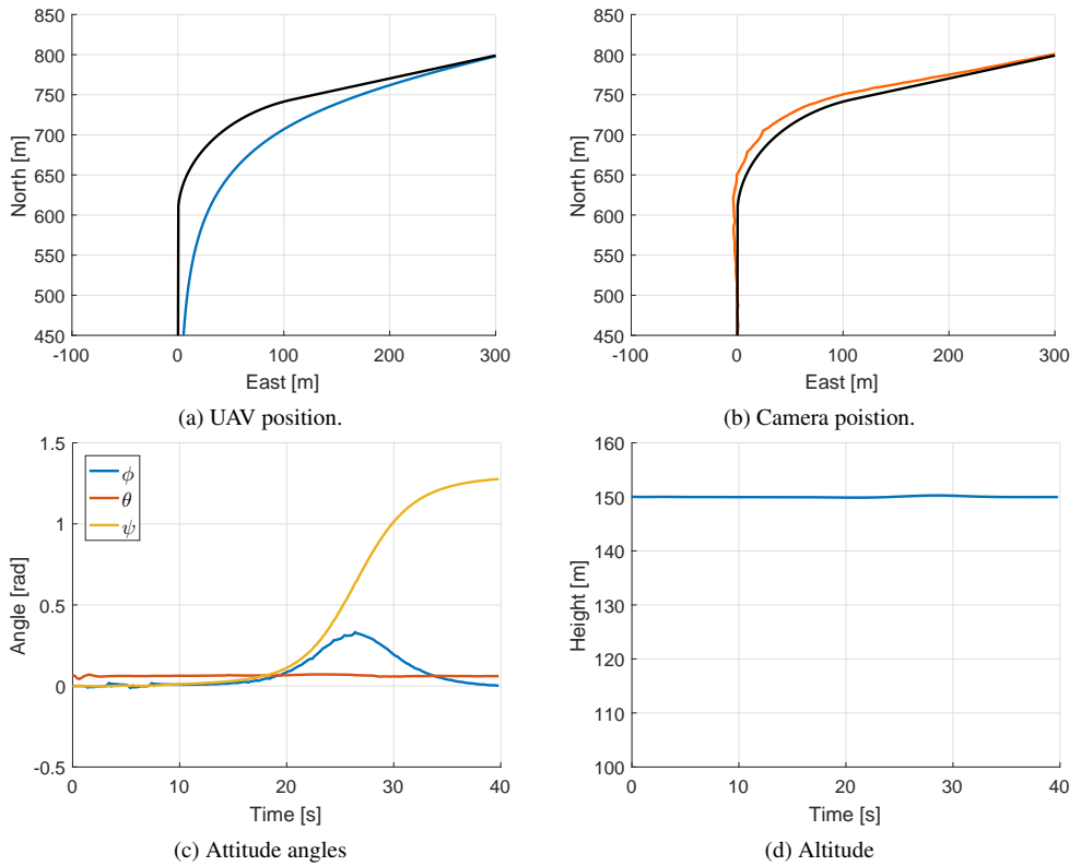
Figure 6.4: Results of optimizing a curved 70^\circ turn.
