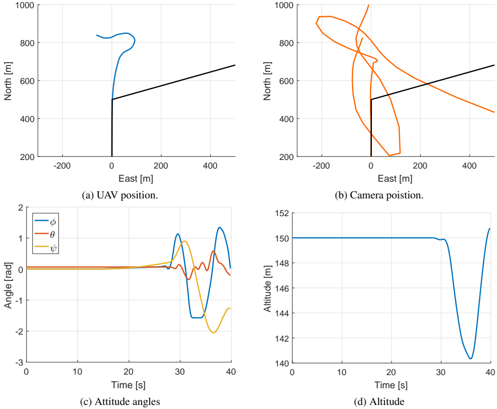
Figure 6.7: Results of optimizing a linear 70^\circ turn with 10^{-5} weight on camera position.
