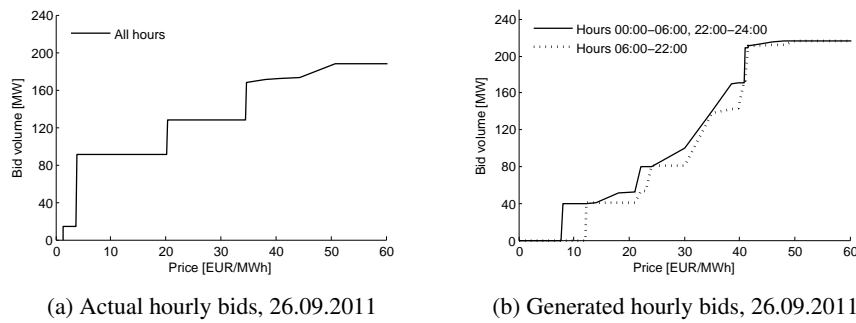
Figure 8: Bids for 26.09.2011 from from Producer A and the bidding model, respectively. The price axes have been cut from 2000 EUR/MWh to make the figures readable.
