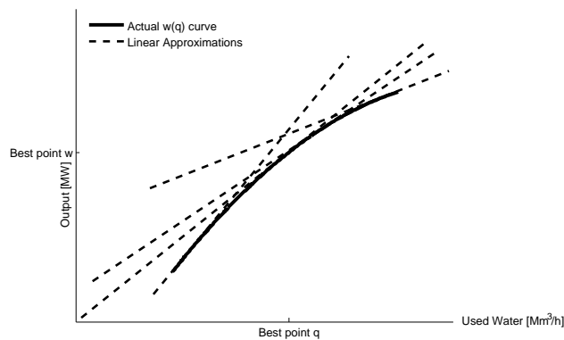
Figure 6: Linear approximations of efficiency curve formulated as conversion from water flow to output power. Minimum and maximum production is indicated by the location of the solid line.
