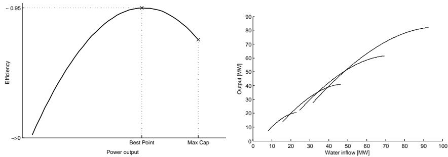
(a) Efficiency curve for a single turbine related to power output. (b) Combined efficiency curves for one to four identical turbines.
