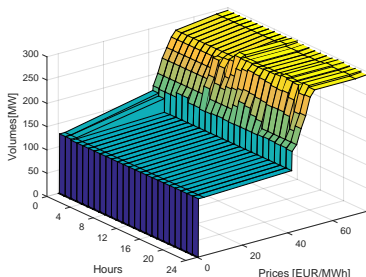
(b) Bids a weekend summer day for Producer B. The bids are quite stable throughout the day. Volumes at the max. and min. prices are constant over the day.
