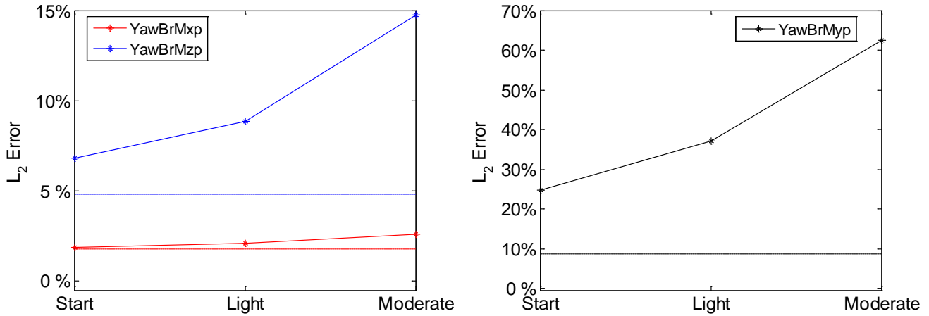
Figure 70 Estimation difference and modeling error of tower root bending moment at different ice on blade categories
