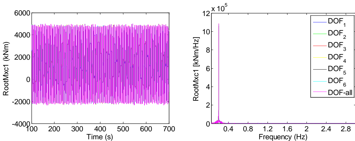
Figure 18 Time series (left) and spectrum (right) of blade 1 root in-plane bending moment
