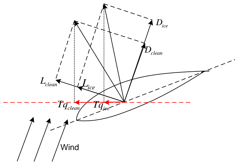
Figure 54 Illustration of torque force change
