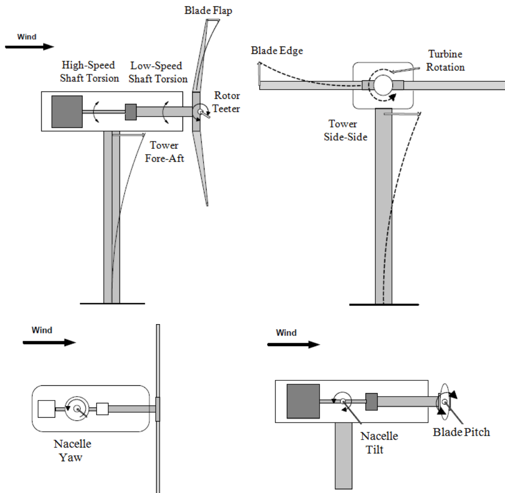
Figure 3 Typical turbine degrees of freedom and motions (Alan D. Wright 2004)
