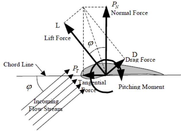
Figure 7 Airfoil section in the rotor plane (J.M. Jonkman 2003)
