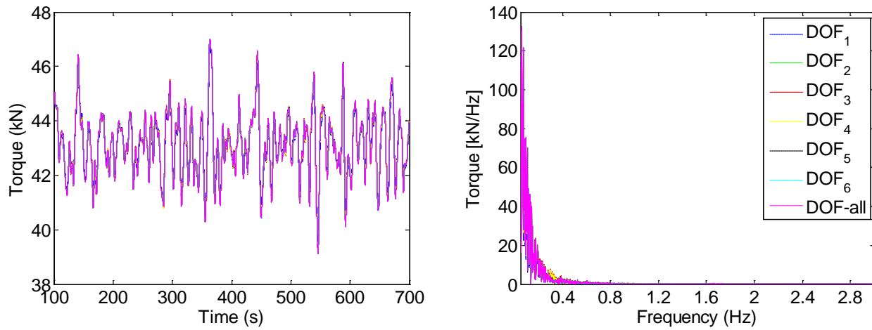
Figure 1 Time series (left) and spectrum (right) of torque under different DOFs
