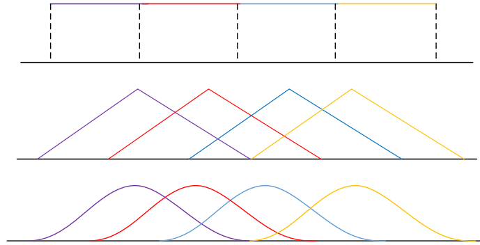
Figure 36 Illustration of interpolation method: Zero order (top) 1 st order (middle) 2 nd order (bottom)
