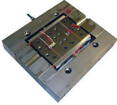
Fig. 1. Custom flexure-guided nanopositioning stage.
