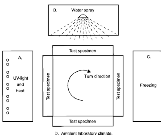
Fig. 14 Test rig for accelerated climate exposure according to NT Build 495 (2000).
