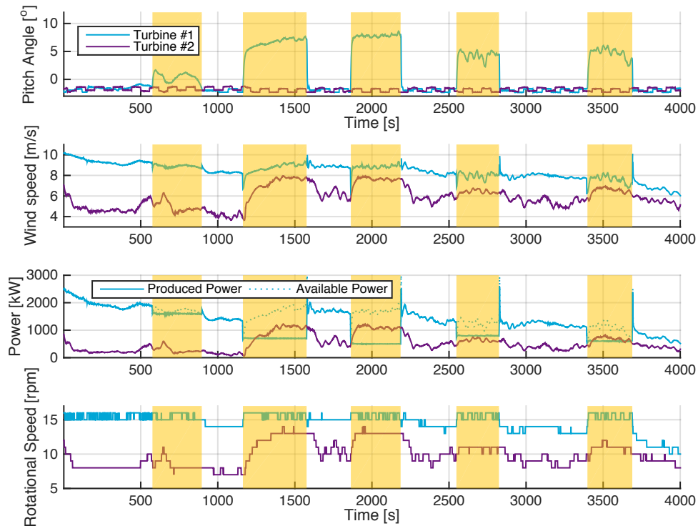
Figure 11.1: Five curtailment experiments performed consecutively. The yellow shaded areas indicate the moments when turbine #1 was being curtailed. In the first experiment the curtailment is often lower than 200\text{ kW} which leads to the rejection of that experiment. The other experiments are all accepted.
