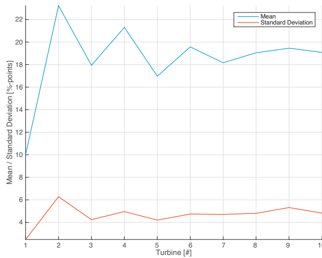
Figure 8.18: Gaussian distribution parameters of turbulence intensity over the turbines.
