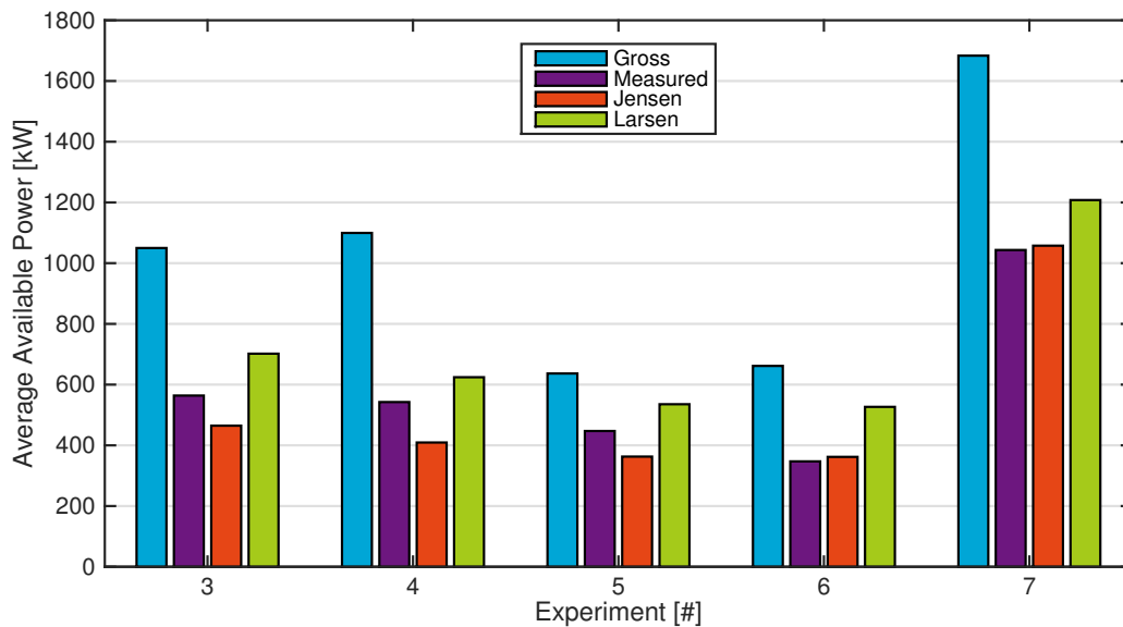
Figure 13.3: Average available power of turbine #2 for gross available power method, measured as the difference between normal and the reference period and the algorithm with the two augmented wake models.
