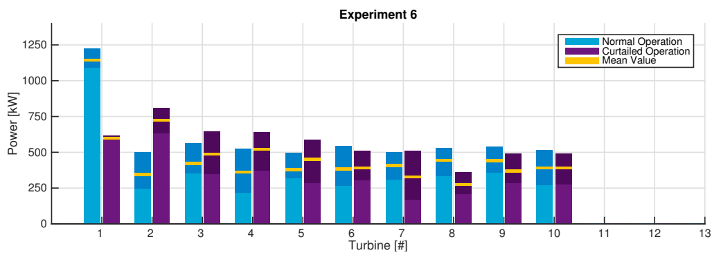
Figure A.11: The power production of all thirteen turbines for the reference period (normal operation) and during curtailment experiment 6. The dark shaded areas indicate the minimum and maximum measured values, while the yellow line shows the mean value.
