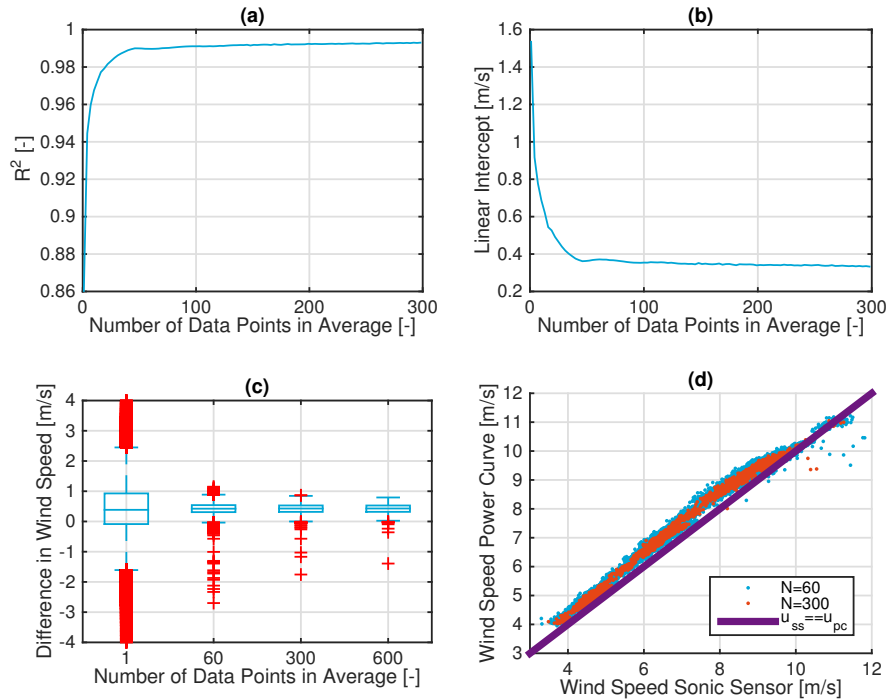
Figure 8.6: Accuracy of using the power curve to determine the wind speed with respect to the sonic sensor. The number of data points in average refers to how many power data points are converted to wind speed - using equation 8.1 - averaged before comparing it to the average of the wind speed measurements. In a and b the coefficient of determination and the linear intercept are shown for the linear regression. In c and d the convergence is visualized with boxplots and the data points themselves for different number of data points in the average. The red points in figure c indicate outliers.
