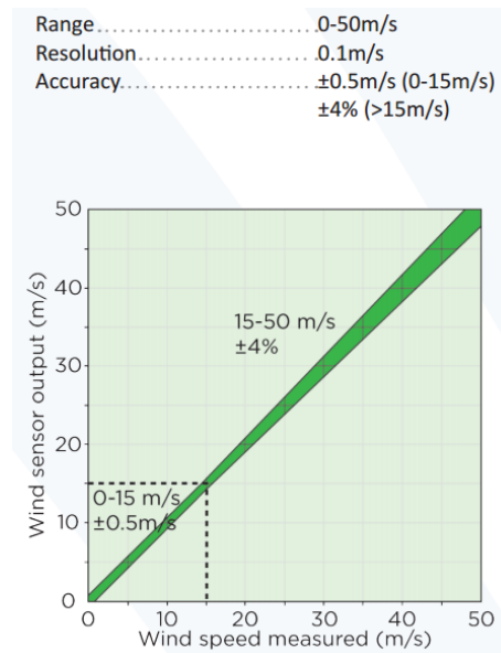
Figure 8.4: Accuracy of sonic wind sensor [31]
