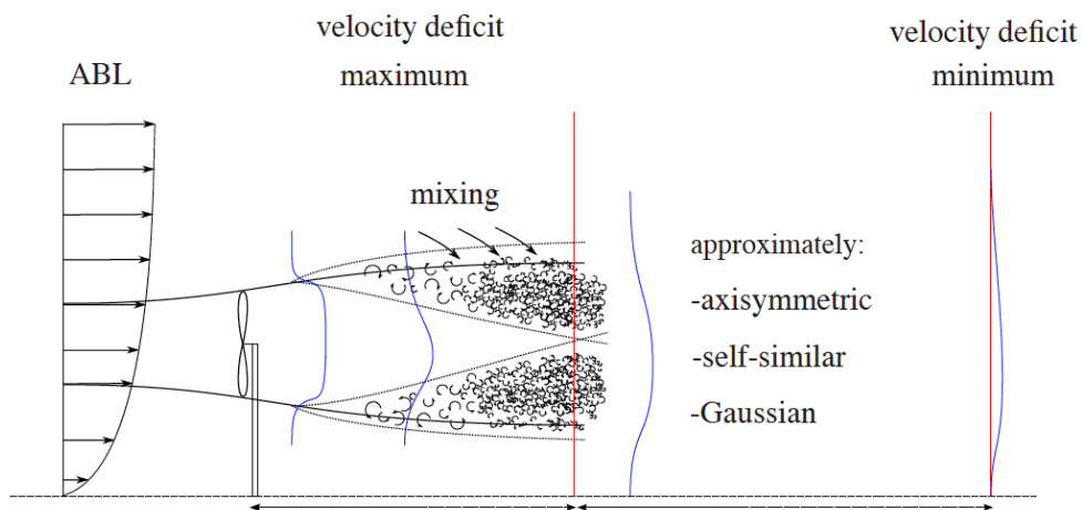
Figure 4.1: Wake expansion[17]
