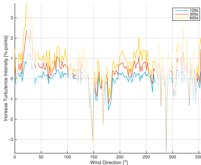
Figure 8.14: Difference of several time spans vs taking a time span of 60s. The dotter parts of the line indicate that there were not enough data points available.
