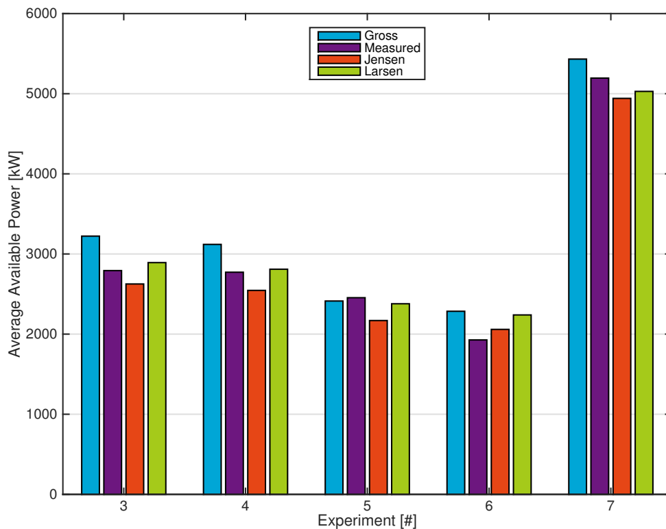
Figure 13.5: Sum of average available power of turbine #1, #2 and #3 for gross available power method, measured as the difference between normal and the reference period and the algorithm with the two augmented wake models.
