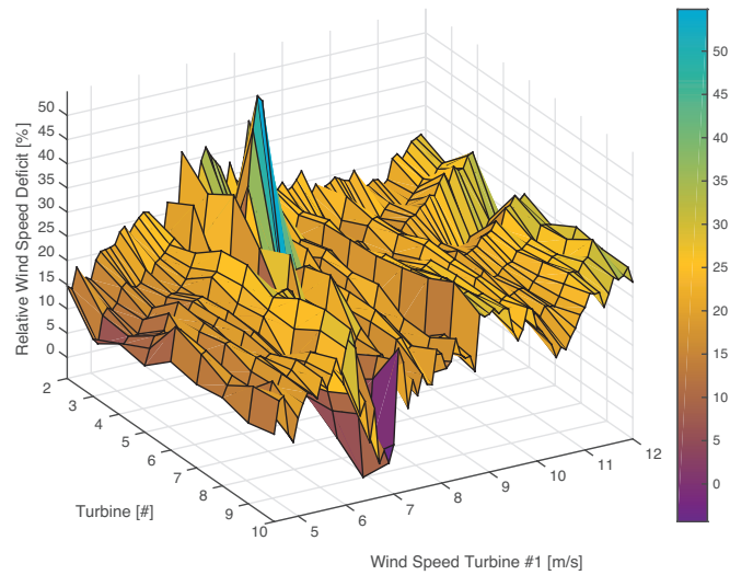
Figure 8.11: Relative wind speed deficit calculated as the wind speed in percentage of the wind speed at turbine #1, similar to figure 8.10.
