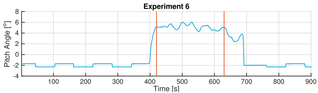
Figure A.10: Pitch angle of turbine #1 corresponding to experiment 6. The vertical red lines indicate the limits of the used experiment data.
