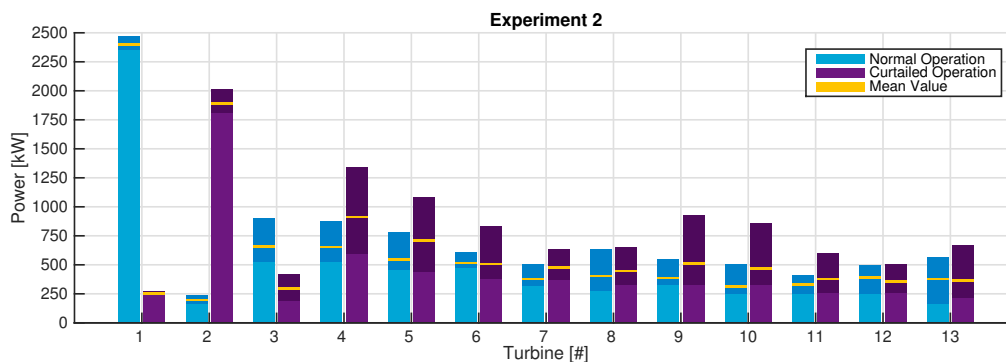
Figure A.2: The power production of all thirteen turbines for the reference period (normal operation) and during curtailment experiment 2. The dark shaded areas indicate the minimum and maximum measured values, while the yellow line shows the mean value.
