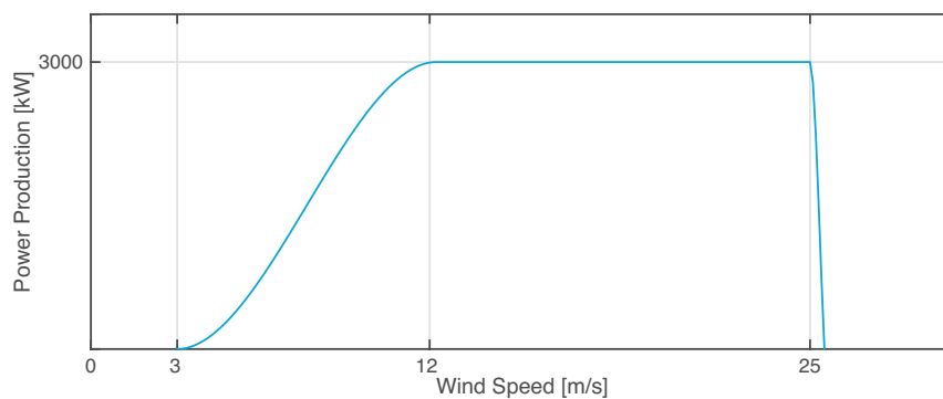
Figure 8.5: Qualitative representation of the power curve
