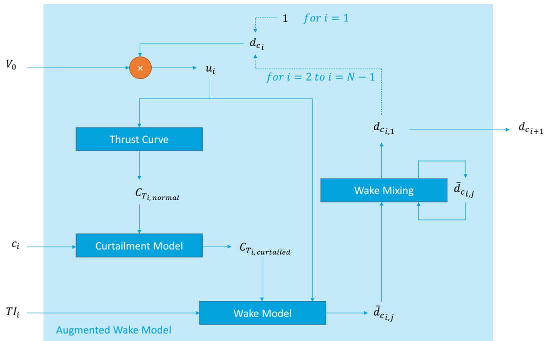
Figure 3.2: The augmented wake model, see tables 3.1 and 3.2 for the explanation of the used symbols. Note that turbine and wind farm constants, like rotor diameter and turbine spacing, are not visualized.
