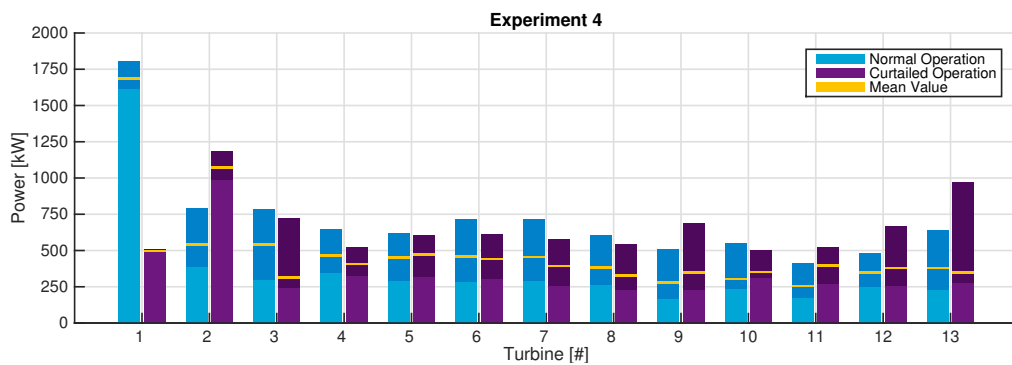
Figure A.6: The power production of all thirteen turbines for the reference period (normal operation) and during curtailment experiment 4. The dark shaded areas indicate the minimum and maximum measured values, while the yellow line shows the mean value.
