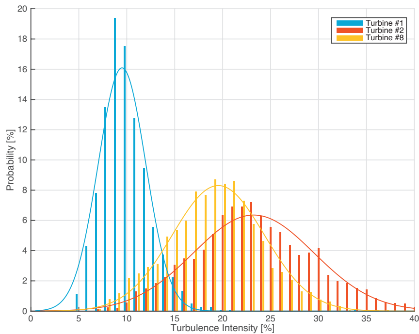
Figure 8.17: Normal probability behaviour of the total local turbulence intensity for different turbines. Note, the curves have been slightly moved to match the bar locations.
