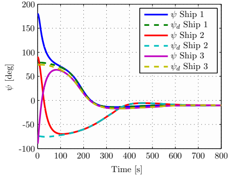
Figure 4.5: Yaw angle and its desired value \psi_d .
