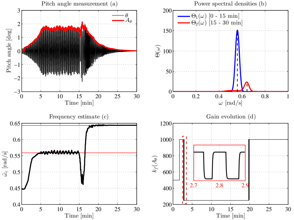
Figure 3.5: Test I: estimation of wave encounter frequency from exponentially modulated pitch angle measurements collected during regular wave experiments R-1173 and R-1189 . The estimator rapidly converges to and track the peak frequency of the power spectral density \Theta(\omega) .
