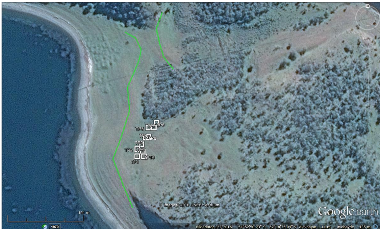
Fig. 50. Locations of test pits (all negative) at the Base of the Varela Hill. Note the double beach ridge here, showing that the Mid-Holocene transgression maximum sea level reached here from both sides. The high point of the two beach ridges are marked with green lines.
