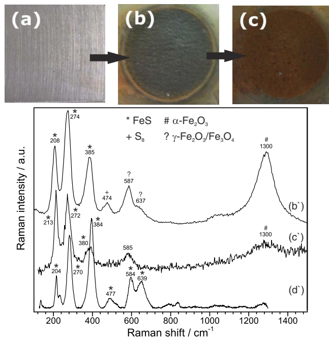
Figure 2. (a) The bare metal before exposure to saline H 2 S saturated acetic solution. (b) Image of area of exposure after anodic polarization for 44 h at 200 mV above E_{\text{corr}} and (b') the corresponding Raman spectrum. (c) Image of corrosion products after aging in air for 90 d and (c') the corresponding Raman spectrum. (d') Reference Raman spectrum for mackinawite as found in the RRUFF database. 50 In the spectra, peaks have been assigned by symbols to certain substances, see Table I. The assignment to FeS is based on the RRUFF database, 50 and is in disagreement with some sources. 29,51,52
