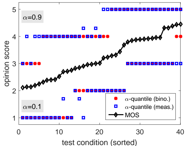
(b) Quantile-MOS Plot. The 10%- and 90%- quantiles ' \square ' for the web browsing study as well as the MOS ' \blacklozenge ' are given for the different test conditions (increasingly sorted by MOS). There are strong differences between the MOS and the quantiles. The maximum difference between the 90%-quantile and MOS is 4 - 2.14 = 1.86 . The quantiles for the shifted binomial distribution ' \bullet ' are also given which match the empirically derived quantiles.
