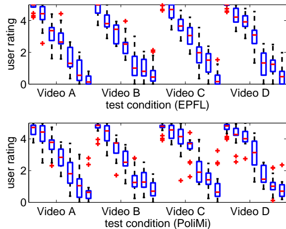
(a) Box Plot. A graphical illustration of the subjective ratings on a continuous scale is a box plot. For each test condition, the user ratings represent a continuous random variable. The box \square quantifies the lower quartile and the upper quartile values as box. The median is provided as line - in the box. Whiskers (dashed lines) extend from each end of the box to the most extreme values within 1.5 times the interquartile range from the ends of the box. Outliers + are data with values beyond the ends of the whiskers. This plot shows also the test settings (four videos, seven packet loss settings) for the two labs (upper and lower subplot).
