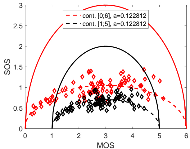
Figure 16: Transformation of user ratings from speech QoE results from rating scale [0; 6] to rating scale [1; 5] leads to the same SOS parameter a . However, the values of MOS and SOS (tuple depicted as diamond marker) as well as the maximum SOS for a given MOS (solid lines) are changing of course.
