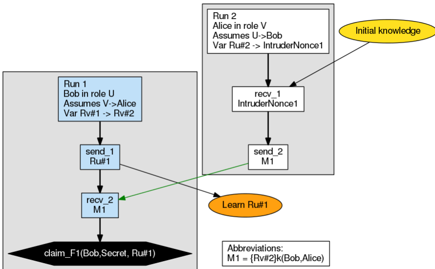
Scyther pattern graph for the TEST protocol, claim TEST,F1 in role U.
