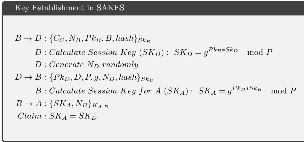
Figure 4.6: Figure of the messages sent between communicating parties in SAKES' key establishment between the end device (A), the 6LoWPAN router (B), and the remote server (D). In SAKES, the session key is established between the router and the server before the router distributes it to the end device.
