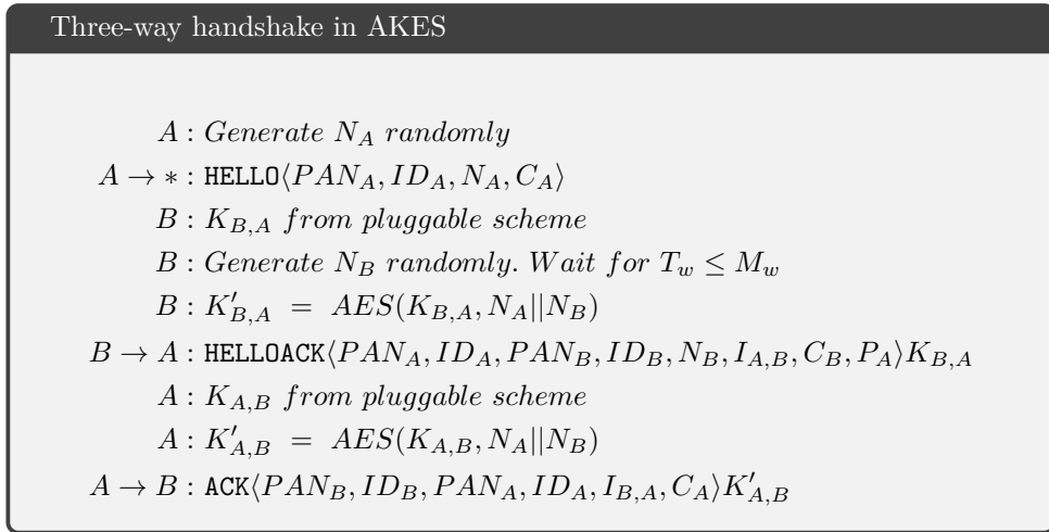
Figure 4.3: Figure of the messages sent between communicating parties during AKES' three-way handshake.
