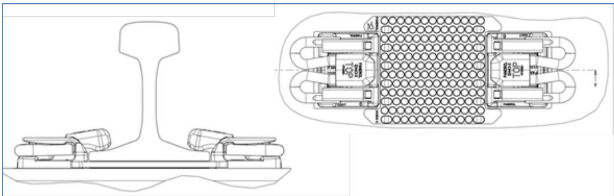
Figur 22 – Befestigelse Pandrol FE Fastclip 44
