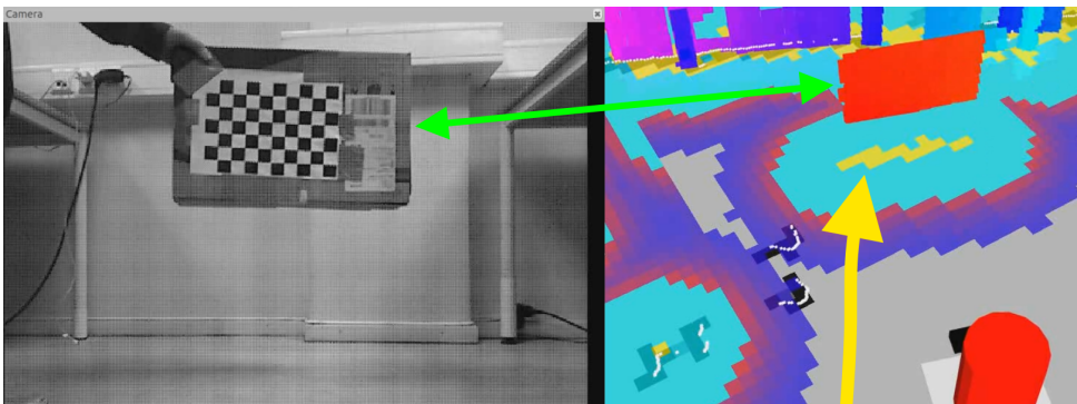
Figure 4.22: 3D Obstacle detection with the live robot. The nodelet obstacles_detection filters out the floor and publishes a point cloud which can be sent to the move_base node. The yellow arrow points to the local cost map, which is based on real-time sensor data and used by the local planner.
