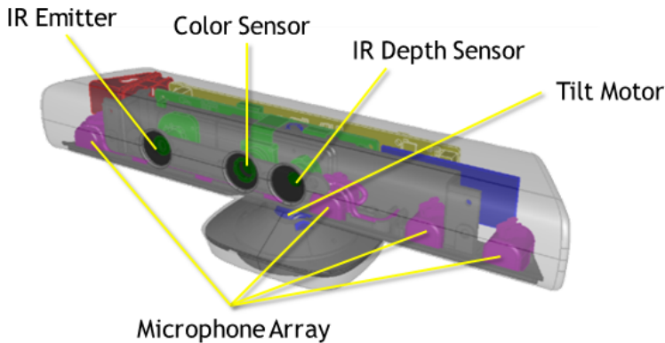
Figure 3.2: Kinect sensor components. (Image credits: Microsoft[kinc])
