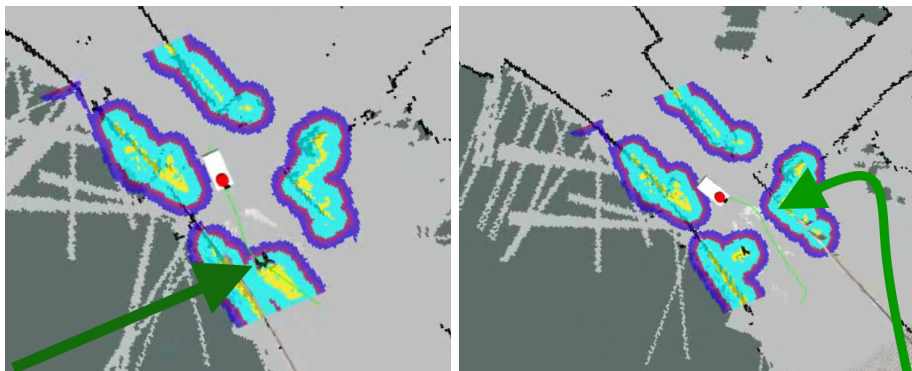
(a) A person has moved into the path of the robot. (b) A new path is planned, avoiding the new obstacle.
