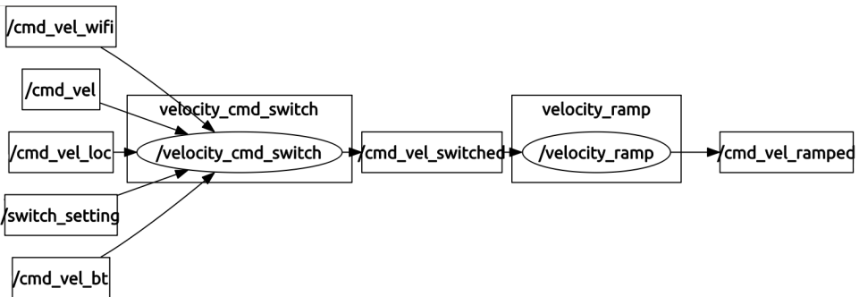
Figure 4.12: Nodes and topics for motion control. (see figure 3.1 for an explanation of this figure).
