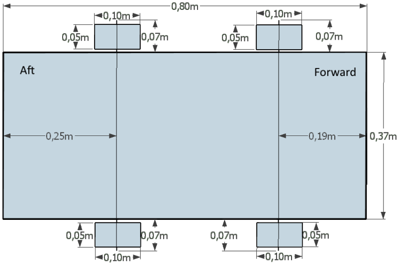
Figure 4.6: The robot footprint. Dimensions are used for the navigation planners and for modeling.
