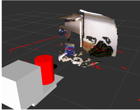
Figure 4.9: Sensor input placed with correct transformations from base_link .
