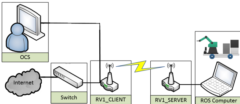
Figure A.1: Network hardware setup.
