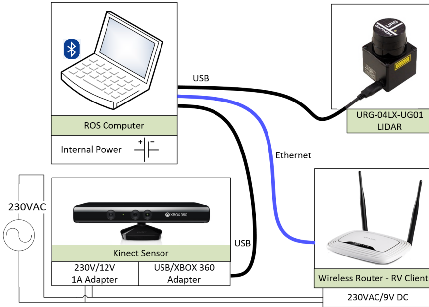
Figure 4.2: Sensor and power supply connections.
