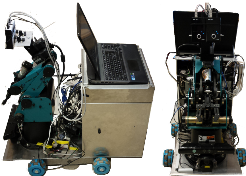
(a) Robot left side.
