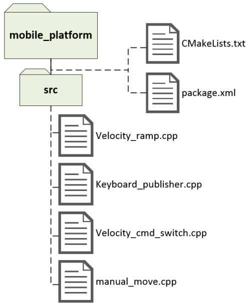
Figure 4.11: Files within the package mobile_platform .
