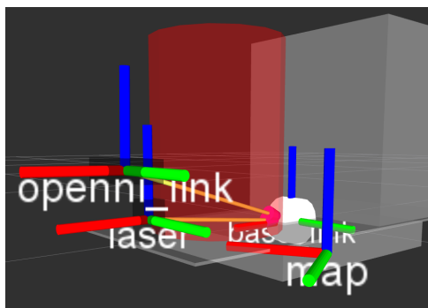
Figure 4.8: Robot model with frames for laser, Kinect, robot base and map.
