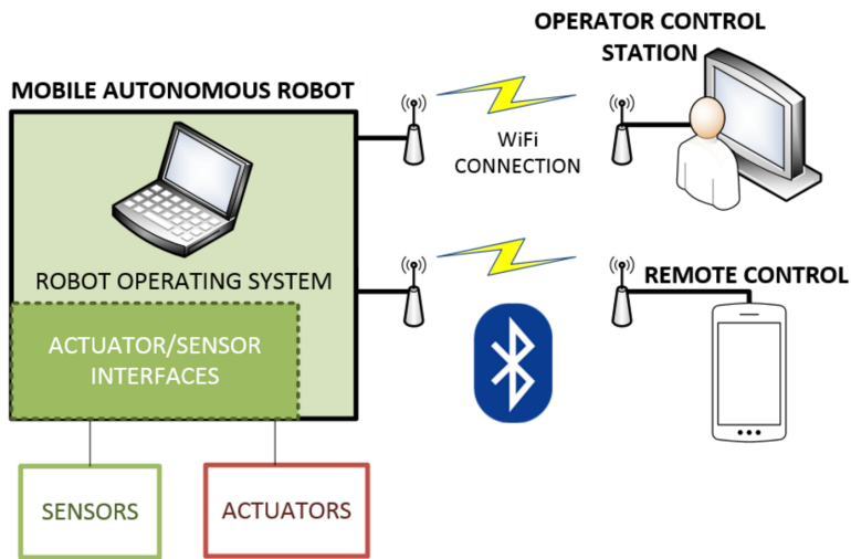
Figure 1.1: System Concept. An on-board computer using ROS to handle actuators and sensors. Remote operation is available through an OCS or a hand-held device with Bluetooth.
