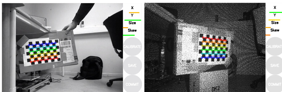
(a) RGB camera calibration. The camera can be calibrated when a sufficient number of samples have been obtained. (b) IR camera calibration. The chessboard pattern will be difficult to detect, because the IR projector is not blocked.
