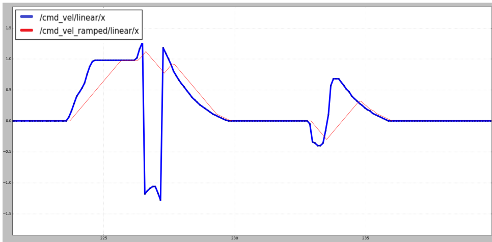
Figure 4.13: The node velocity_ramp limits the rate of change of the velocity command sent to the motor control card. The blue line represents commands entering velocity_ramp , while the red line shows the acceleration constrained output command.
