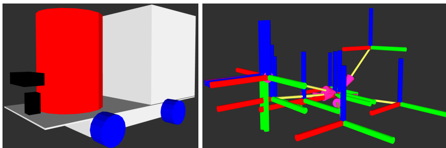
(a) Complete URDF model when viewed in rviz . (b) URDF model in rviz with all link frames and transformations.
