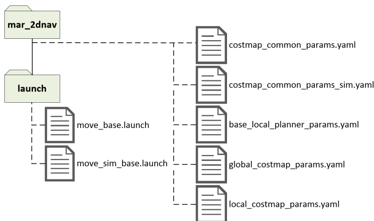
Figure 4.20: Files for configuring and launching the navigation stack.
