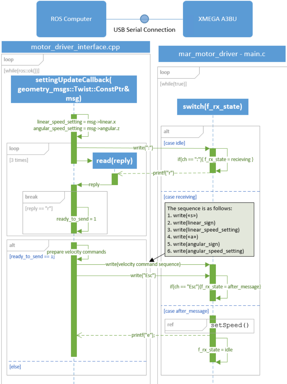
Figure 4.15: Velocity command transmission sequence from the motor_driver_interface in the ROS computer to the motor control card (XMEGA A3BU).
