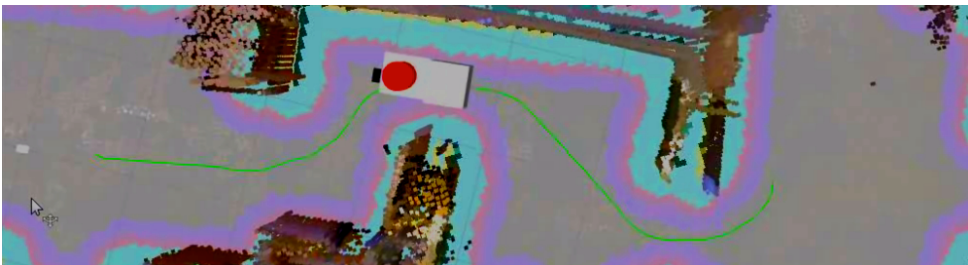
Figure 5.10: Global planning with the live robot. The green line illustrates the globally planned path. The inflated obstructions in the global costmap are highlighted as colored spots.
