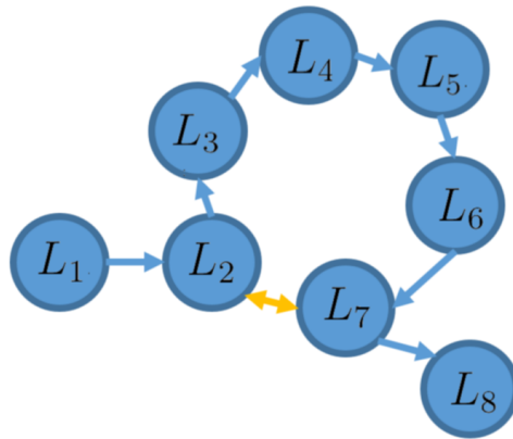
Figure 3.3: Conceptual illustration of a graph created by RTAB-Map over time 1 \leq t \leq 8 . A loop closure hypothesis was accepted at t = 7 , as shown by the yellow arrow. Feature descriptors in L_2 and L_7 are sufficiently similar to accept this as a loop closure.
