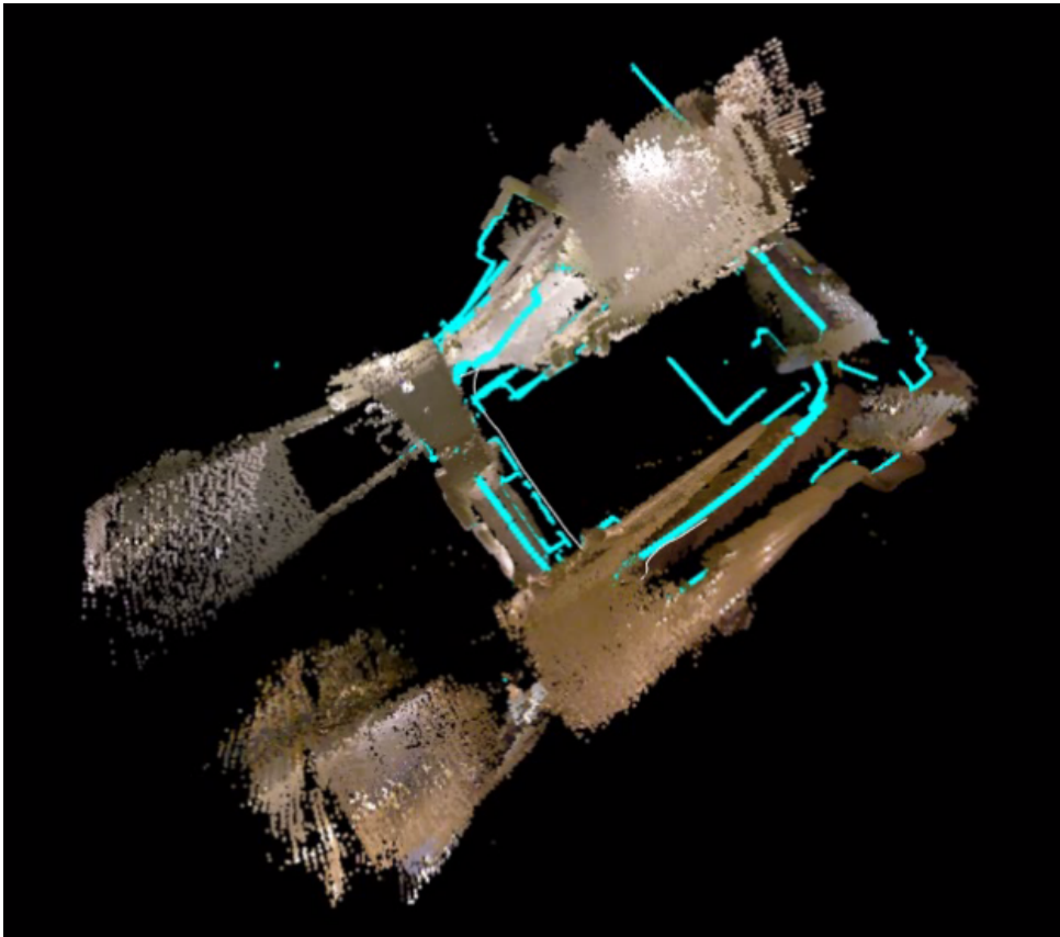
Figure 5.9: The resulting 3D map of the same area as in figure 5.7a.
