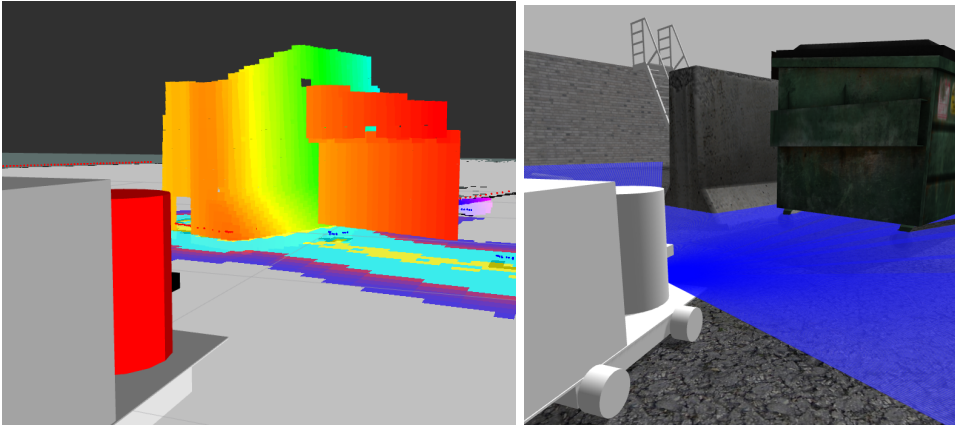
(a) A point cloud representation of the obstruction. Notice how the local costmap is based on the detected point cloud. (b) The obstruction in the Gazebo simulation. Notice how the LIDAR only detects the wheels below the container.
