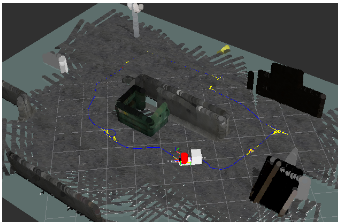
Figure 5.2: An example of a resulting point cloud map after running RTAB-Map in Gazebo.
