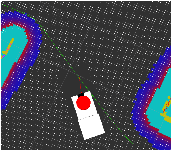
Figure 5.6: The robot footprint is illustrated by the clear rectangle that surrounds the robot model. The coloured areas are map locations with high cost.
