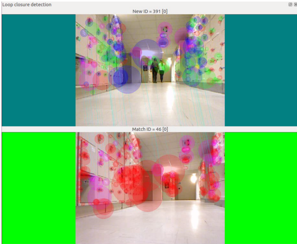
Figure 5.8: An example of an accepted loop closure hypothesis during a live mapping session. As before, the matched features are indicated by the pink circles.
