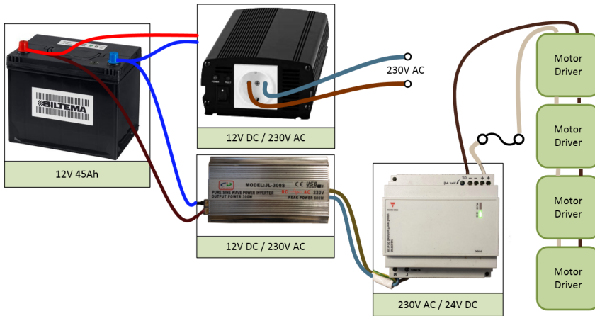
Figure 4.4: Example of a feasible power supply setup.
