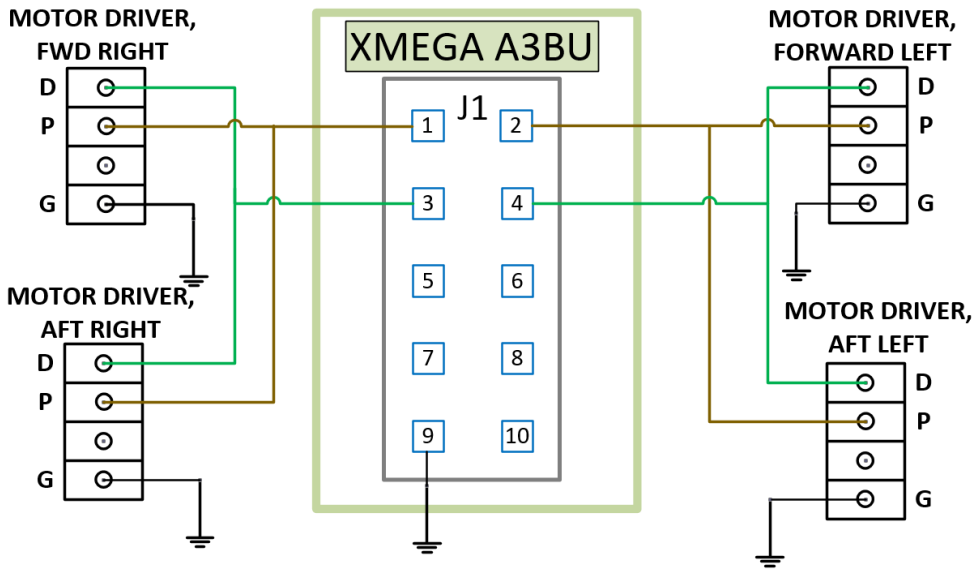
Figure 4.14: Connections between each wheel motor driver and the motor control card, XMEGA A3BU. The connections are unchanged from [Asp13], except for some improved connection for better short circuit prevention.
