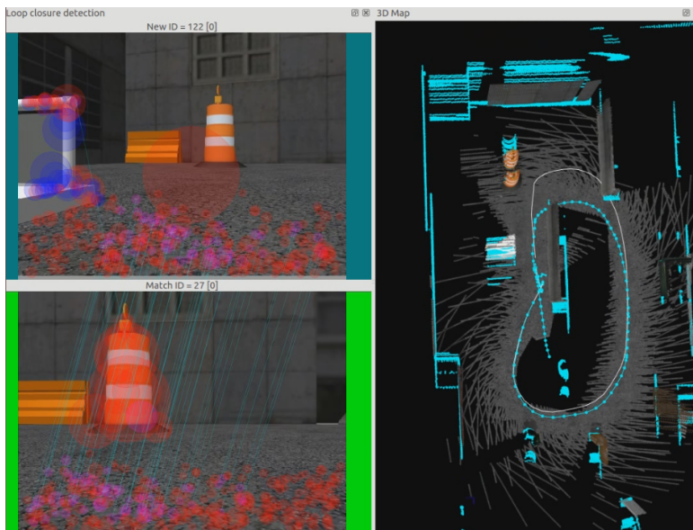
Figure 5.3: Example of an incorrect loop closure detection. The pink circles indicate matching features. The right part shows an incorrect map adjustment. Observe how the matching features are located on the asphalt plane.
