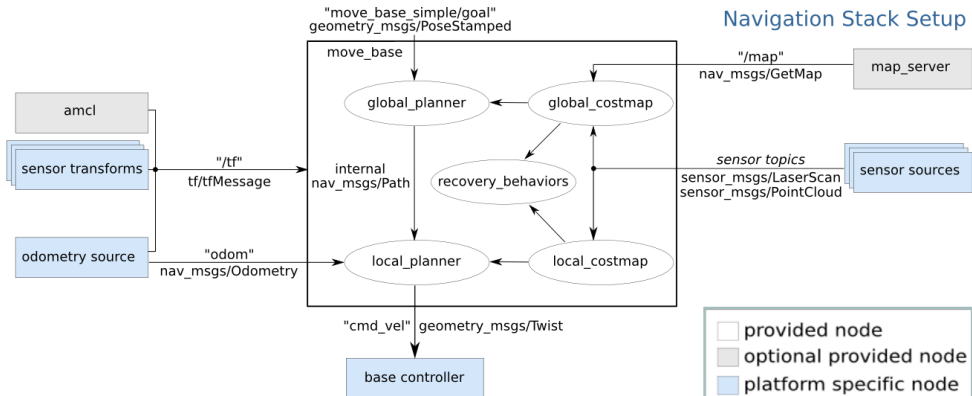
Figure 3.4: move_base and the navigation stack. (Image credits: ros.org)
