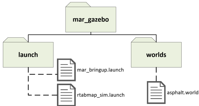
Figure 4.10: Folders and files specific for the simulator.
