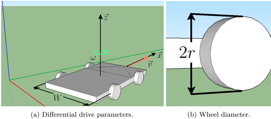
Figure 4.16: Parameters for differential drive kinematics. Note that the frame vectors \vec{z} and \vec{x} refer to the base frame of the robot in this case, and not the world frame.
