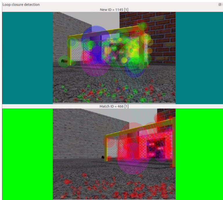
Figure 5.4: An example of an accepted and correct loop closure hypothesis. This example is from the "Asphalt" world simulated in Gazebo.
