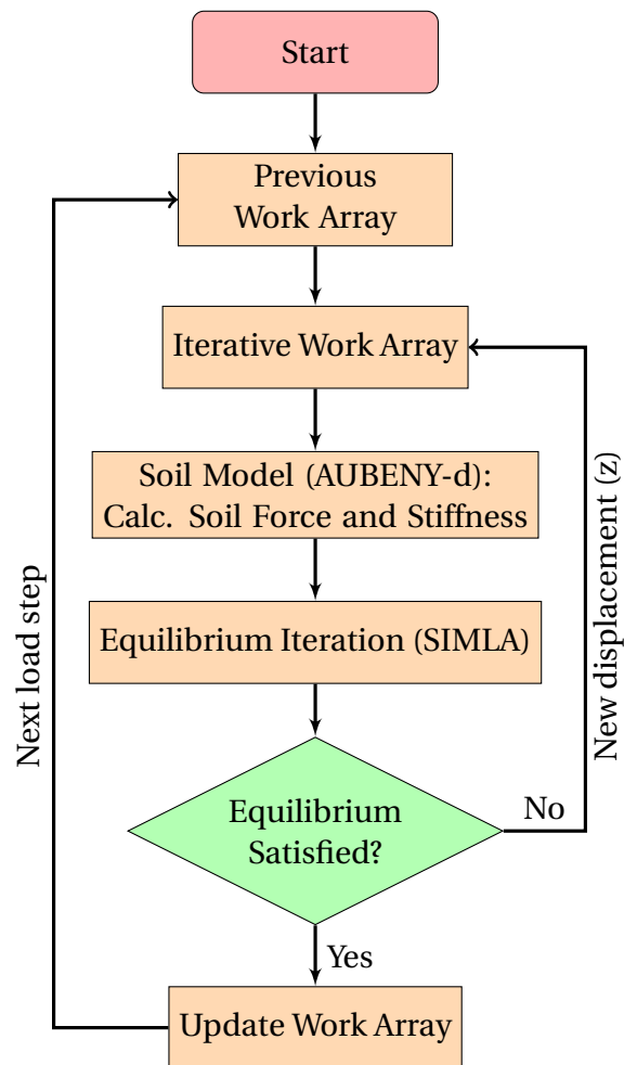
Figure 9.1: Flowchart of Soil Model in SIMLA (Irman, 2015)
