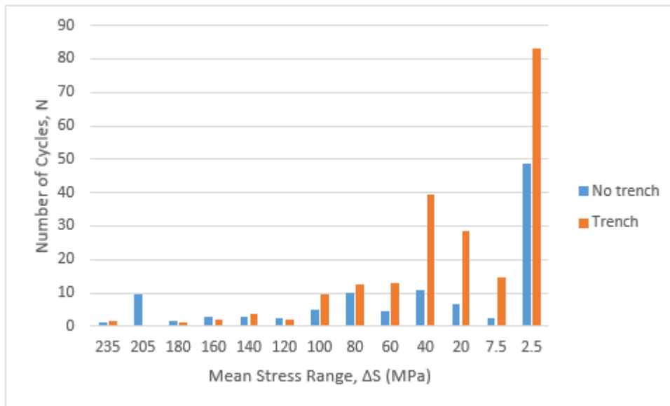
Figure 11.7: Stress Histogram of Riser Element 119
