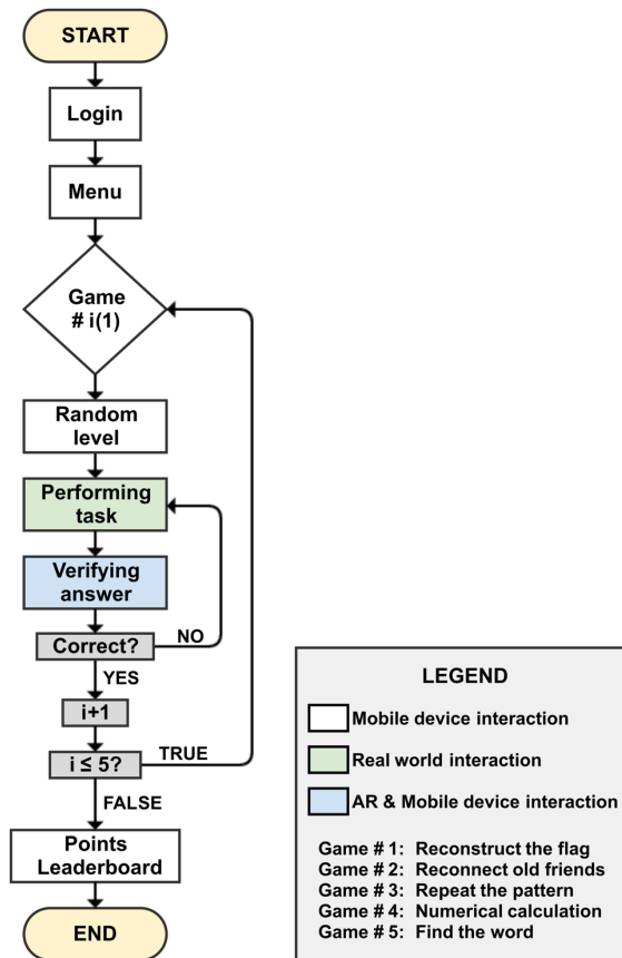
Figure 3.7: The flowchart of a full gaming session with Smartkuber.
