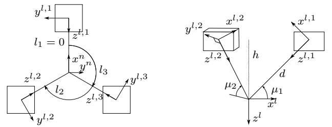
(a) Top view. Three hexacopters are positioned evenly around a load in the center. (b) Side view where you can see two hexacopter bodies and their relative position to the load.
