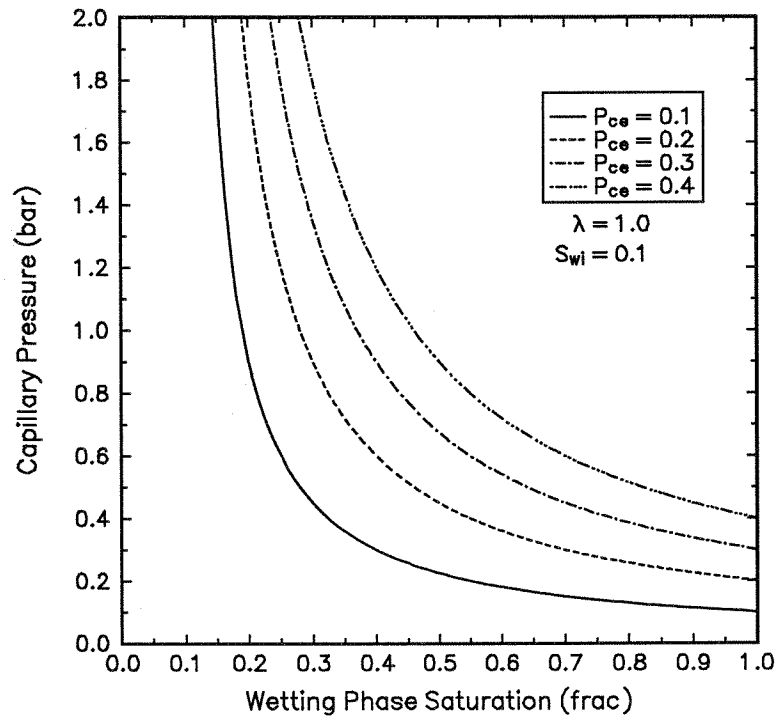
Fig. 3.17 Corey capillary pressure function for various values of P_{ce}
