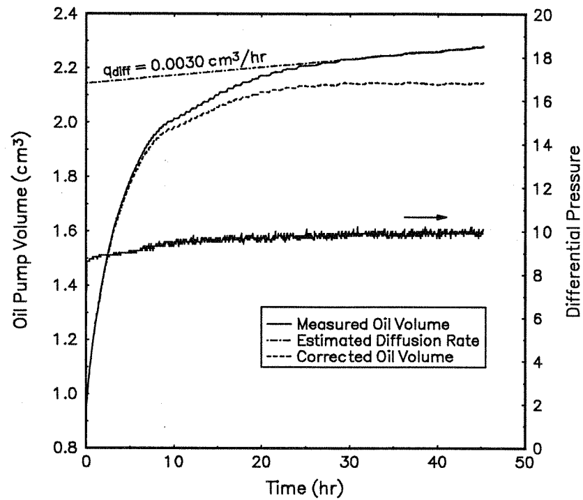
Fig. 3.63 Example of produced oil volume vs. time for run 92-8 at \Delta p = 10 \text{ mbar} ( p = 130 \text{ bar} and \text{IFT} = 1.5 \text{ mN/m} )
