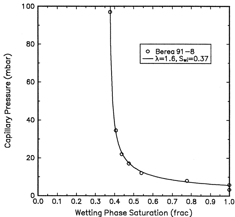
Fig. 3.55 Capillary pressure curve for Berea sandstone at 105 bara with Corey curve (IFT=3.2 mN/m)
