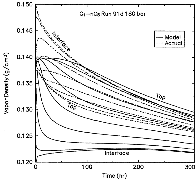
Fig. 2.24 Model and actual density for the vapor phase vs. time
