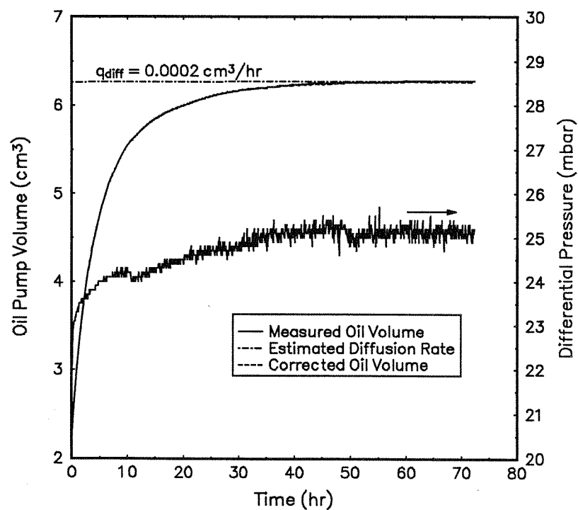
Fig. 3.64 Example of produced oil volume vs. time for run 92-8 at \Delta p = 25 \text{ mbar} ( p = 130 \text{ bar} and \text{IFT} = 1.5 \text{ mN/m} )
