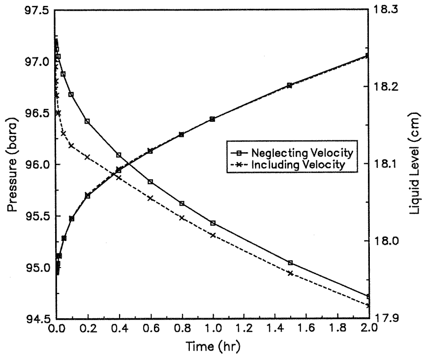
Fig. 2.9 Comparing CVD simulators at first two hours for C_1 - C_5 (no VLT)
