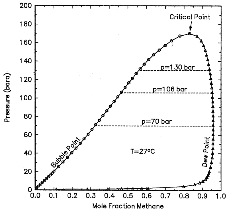
Fig. 3.53 Pressure-composition diagram for the C 1 -nC 5 system (Berry and Sage, 1970)
