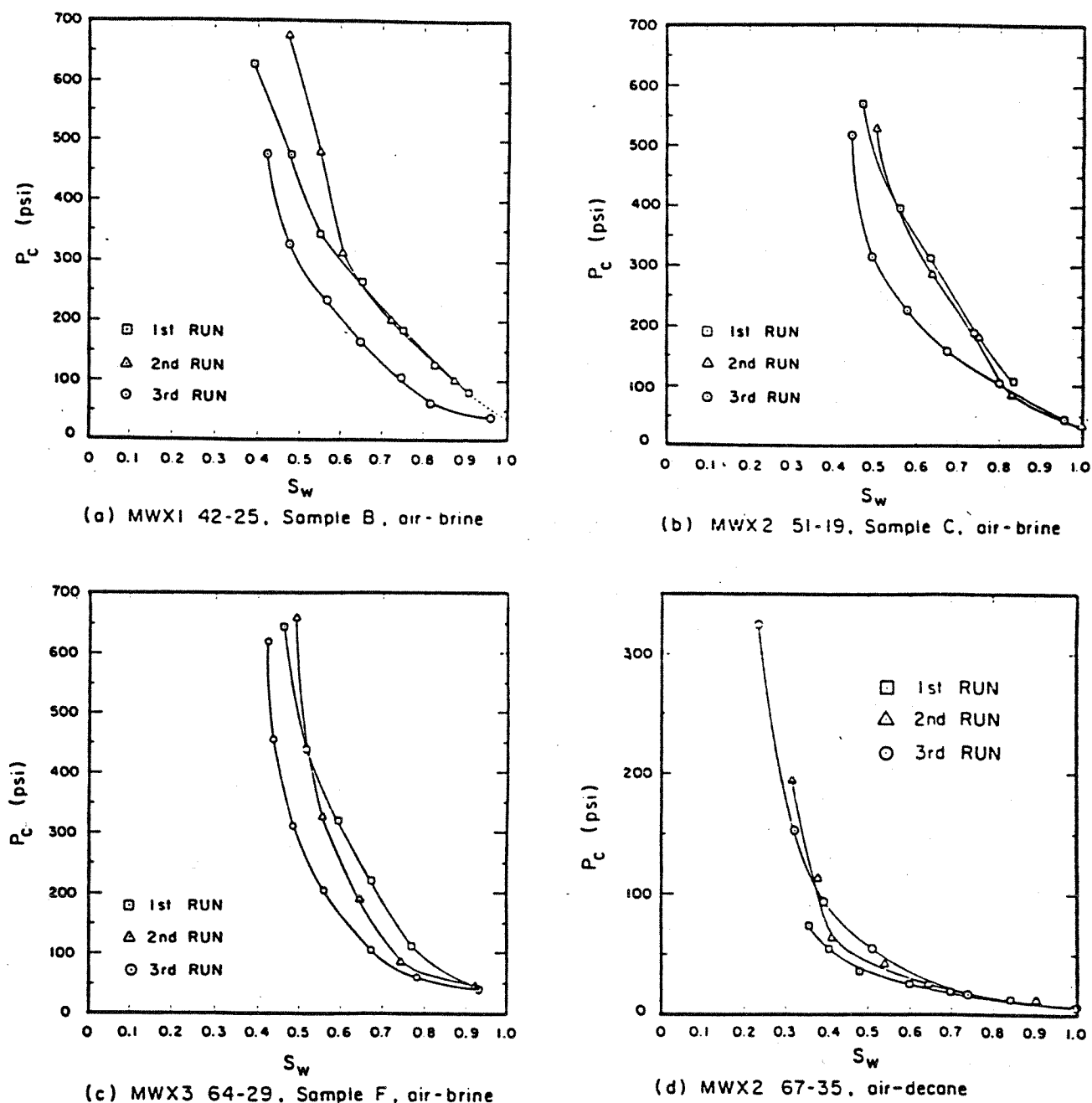
Fig. 3.21 Capillary pressure curves for repeated runs on a given core using the Hassler and Brunner method on centrifuge data (Ward and Morrow, 1987)
