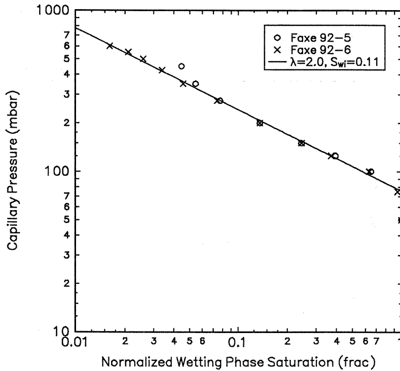
Fig. 3.58 Corey log-log curve fit for Stevens chalk at 105 bara (IFT = 3.2 mN/m)
