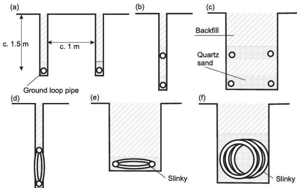
Figure 9. Examples of horizontal configuration.
