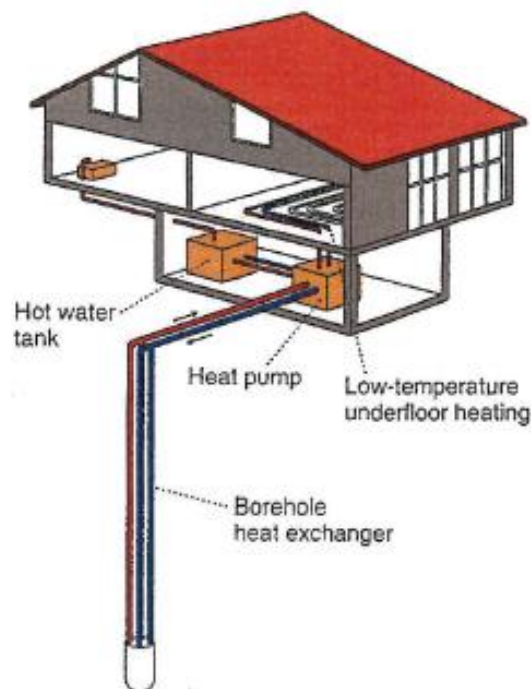
Figure 10. Example of vertical configuration [Dickson et al., 2004].
