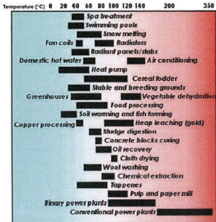
Figure 4. Utilization of geothermal fluids [Dickson et al, 2004]
