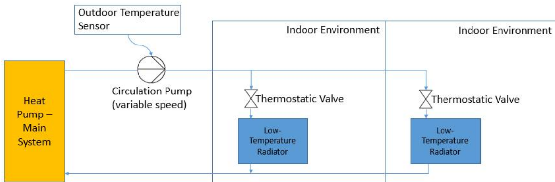
Figure 15. Sketch of how the space heating system should be.
