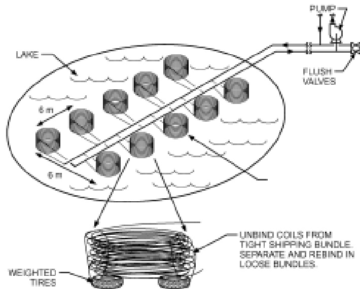
Figure 5. Configuration for a closed-loop application [ASHRAE Handbook 2011, HVAC Applications].
