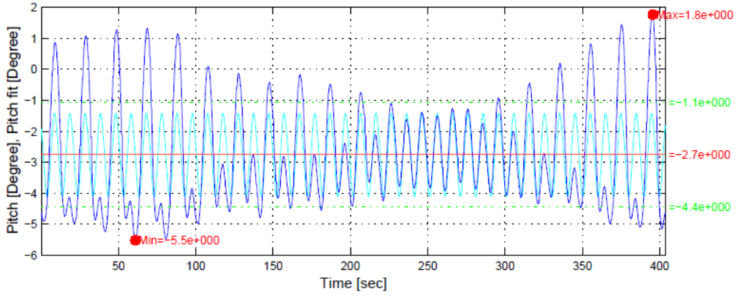
Figure 6.41: Model test pitch results with H=5m and T=9.9s
