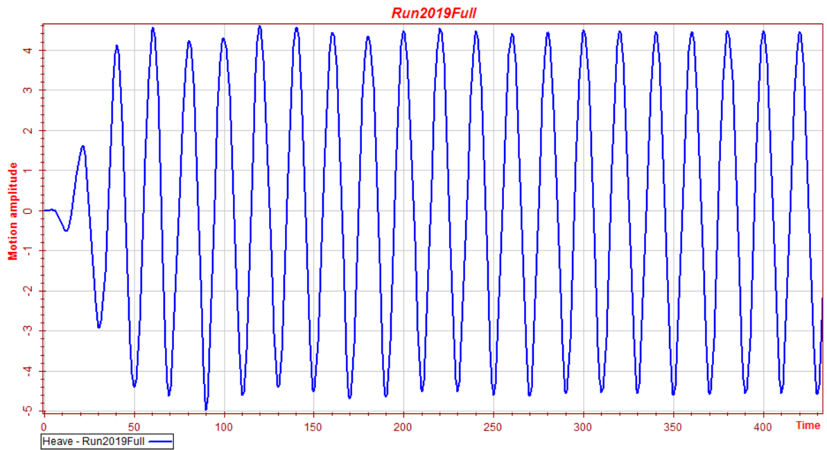
Figure 6.33: Wasim heave results with H=9\text{m} and T=20\text{s}
