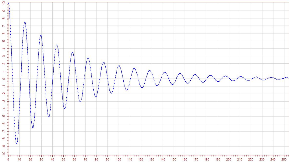
Figure A.5: Pitch decay test results in pitch from Wasim
