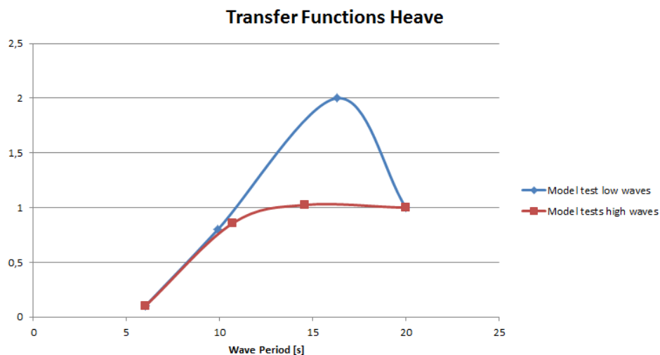
Figure 7.2: Heave RAOs calculated with different wave heights
