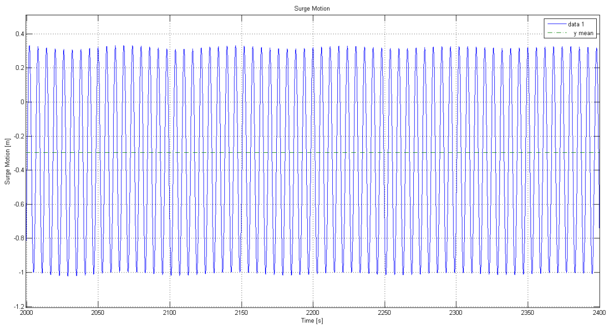
Figure 6.2: Matlab surge results with H=3m and T=6s
