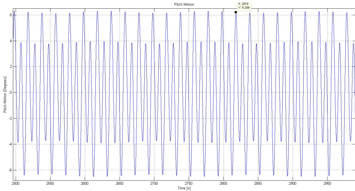
Figure 6.35: Matlab pitch results with H=9m and T=20s
