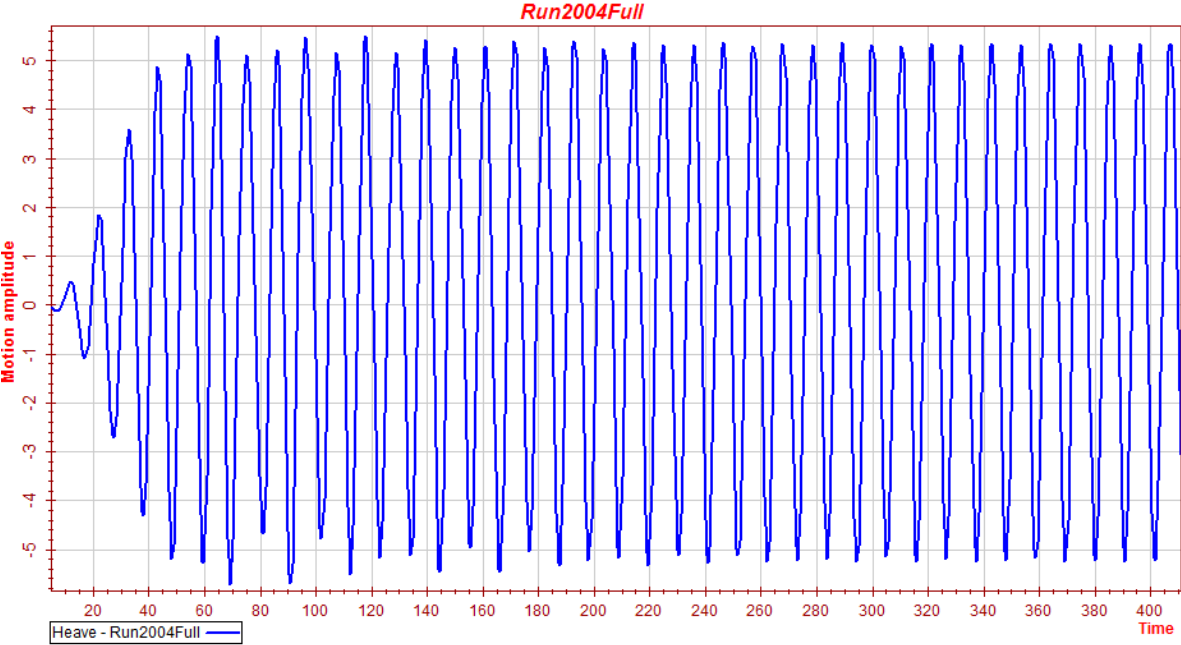
Figure 6.6: Wasim heave results with H=3m and T=6s
