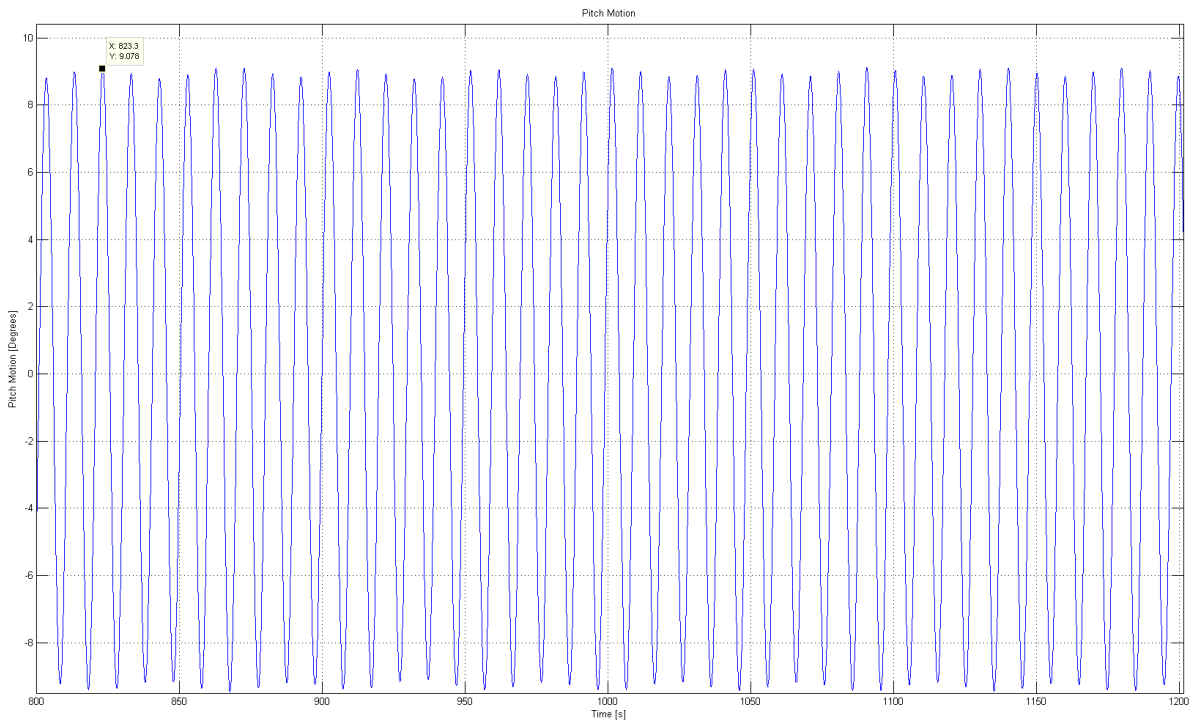
Figure 6.42: Matlab pitch results with H=5m and T=9.9s
