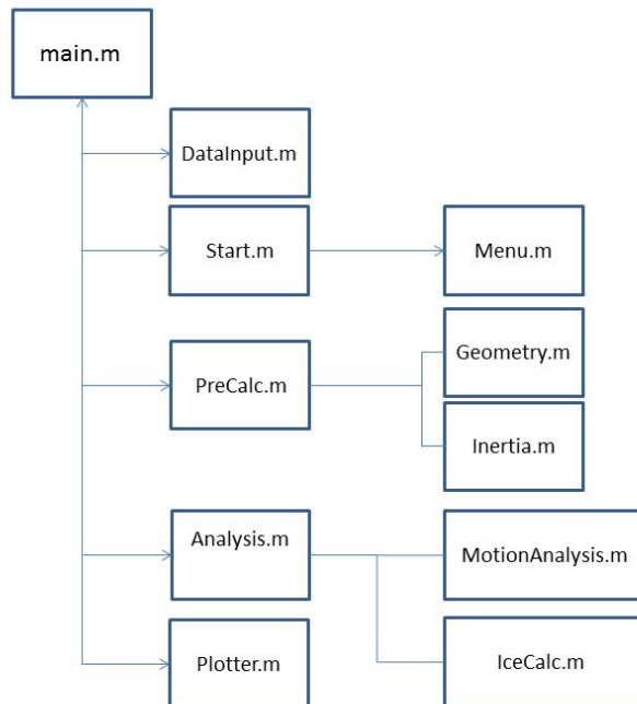
Figure 3.3: Flow diagram with main subroutines
