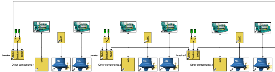
Figure 2.3: Example of power plant view, including the bus-tie breakers, thrusters, generator sets, and other loads block. This power plant is used for simulation of drilling rig in Section 2.4.
