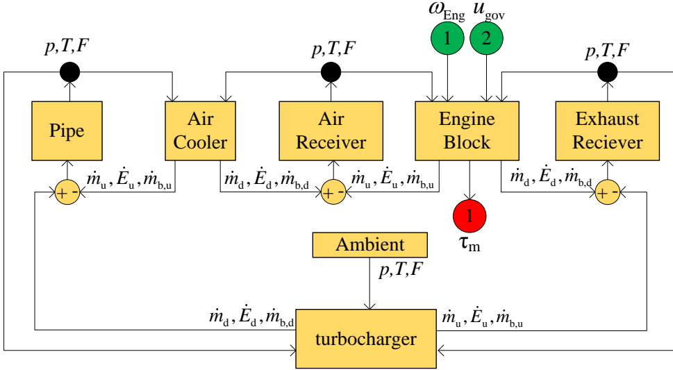
Figure 2.5: Mean value engine system model scheme, including a turbocharger, a charge air cooler and incylinder process.
