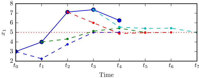
Figure 4.2: Nominal and fault prediction when the relaxable constraints are relaxed during the first three steps, and during the three first fault predictions. Note that the three first fault predictions can violate the state constraint x_1 \geq 5 for the entire horizon and terminal constraint. The system is presented in Section 4.7.1.
