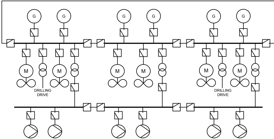
Figure 6.2: Power plant of simulated drilling vessel used in case study.
