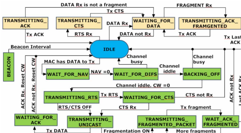
Figure 33. The Finite state machine of 802.11 [63, fig.1]
