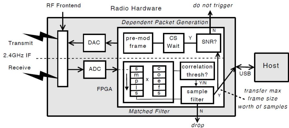
Figure 32. Matched filter & dependent packet design [69, fig.7].
