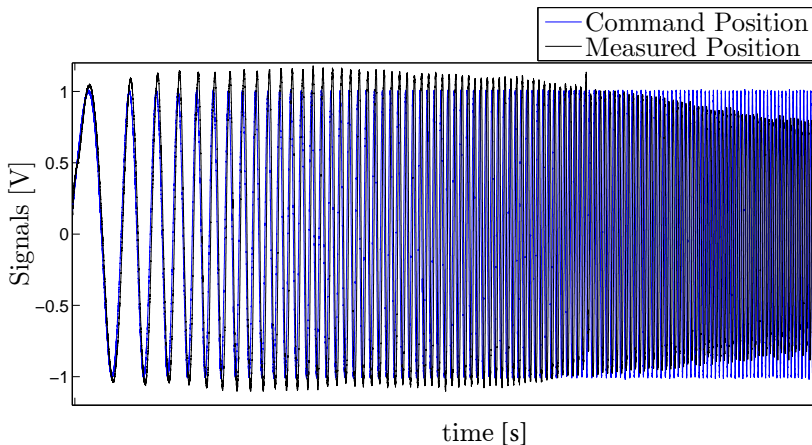
Figure 3.10: The servo system is following a 1V amplitude command signal with increasing frequency as time increases.
