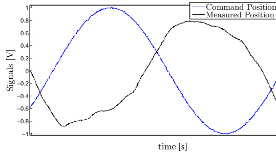
Figure 3.11: Figure 3.10 zoomed in at the end.
