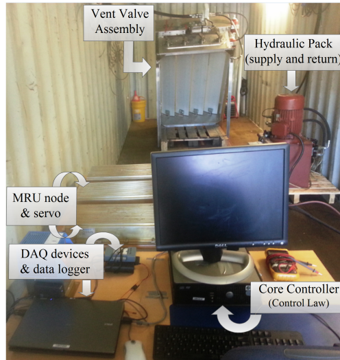
Figure 3.5: Test overview.
