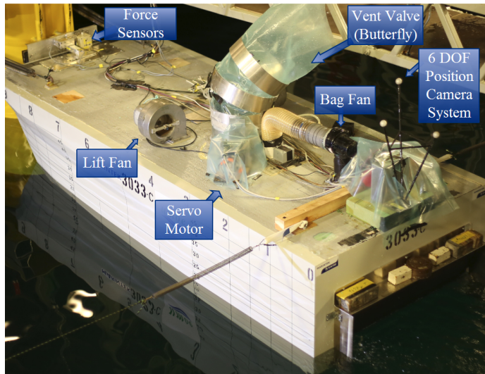
Figure 1.21: The location of certain instrumentation. Picture taken in the Ship Model Tank, Sintef Marintek.
