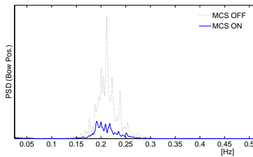
Fig. 6. Head sea, H_s = 1m , T_s = 5s
