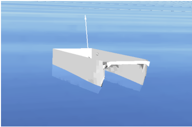
Fig. 3. SES Simulation and visualization using ShipX plug-ins
