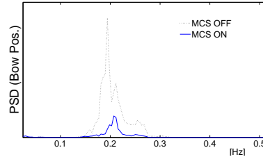
Fig. 8. 135° sea, H_s = 1m , T_s = 5s
