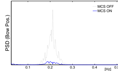
Fig. 9. 180° sea, H_s = 1m , T_s = 5s
