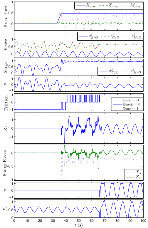
Figure 10: Simulation run with three phases. The label on the y-axes describe the corresponding signal
