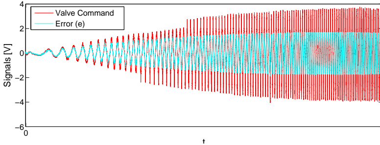
Figure 3.13: Valve Command and error signal.
