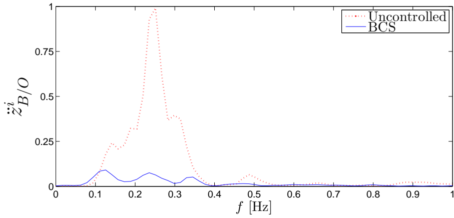
Figure 3.18: Bow acceleration PSD plot with, and without, the BCS active.
