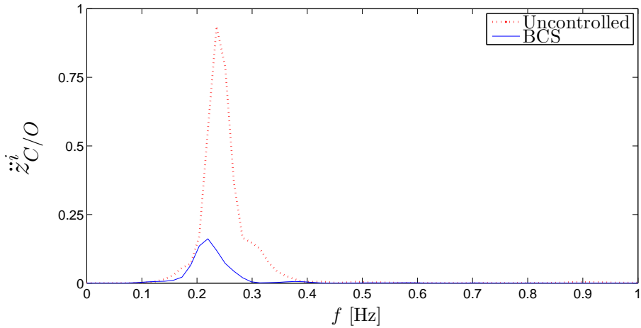
Figure 3.19: CG acceleration PSD plot with, and without, the BCS active.
