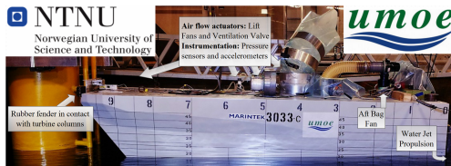
Figure 4: The Wave Craft model test. Courtesy of Umoe Mandal.
