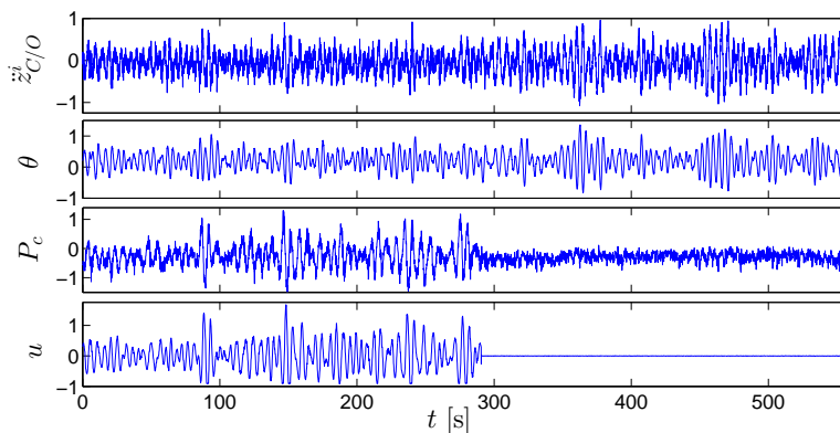
Figure 3.15: Time series plot of the bow acceleration. The BCS is initially on and turned off at t = 290 s.
