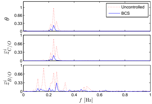
Figure 16: PSD curves showing BCS performance, no turbine contact. Upper: pitch angle, middle and lower: acceleration in bow- and CG, respectively.
