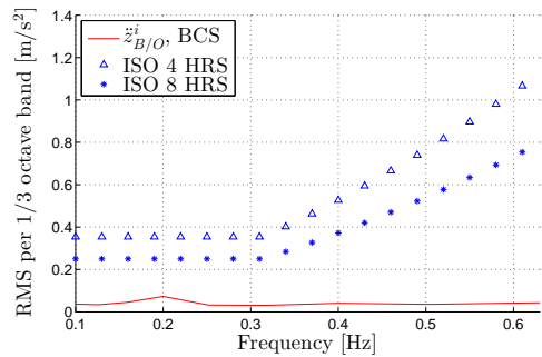
Figure 17: ISO 2631/3 (1997) Seasickness criterion.
