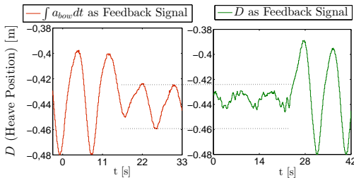
Fig. 2. The plot shows the effect of a long crested regular wave, T_p = 8.5s . D is measured by lab equipment and \int a_{bow} dt was given by numerical integration of a high-pass filtered accelerometer signal. The accelerometer was attached at the origin of the \{p\} frame.
