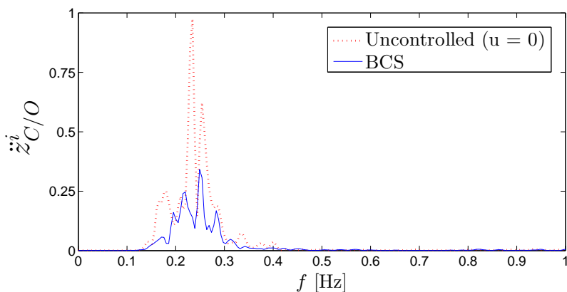
Figure 3.16: PSD plot of the bow acceleration with, and without, the BCS active.
