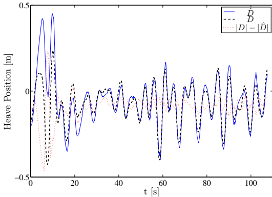
Fig. 11. Bias is added to the accelerometer, b_{z,k} = +2 .
