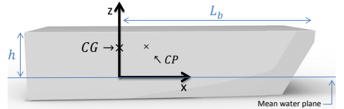
Fig. 5. Body fixed coordinate system B . CG and CP are set to illustrate possible longitudinal positions but not actual design parameters.
