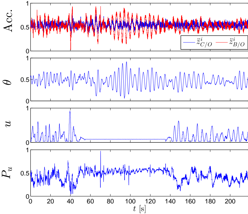
Figure 3.17: Time series with and without ( t = \{53, 1356\} s) the BCS active.
