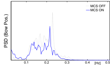
Fig. 10. 90° sea, H_s = 1.5m , T_s = 7s
