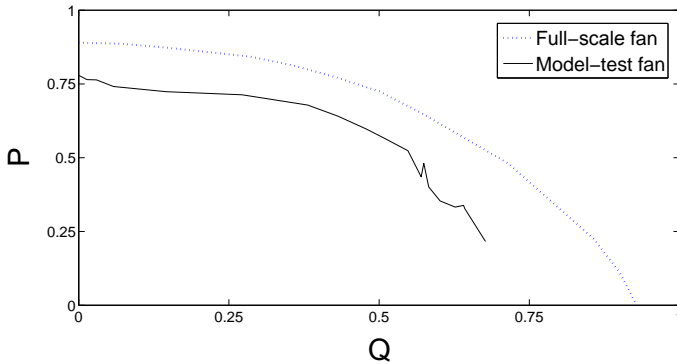
Figure 1.27: Lift Fan Characteristics. The actual full-sized, optimal speed, Wave Craft fan are intentionally designed with a safety margin in terms of air flow capacity.
