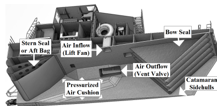
Figure 3: A typical SES. Illustration by Umoe Mandal.
