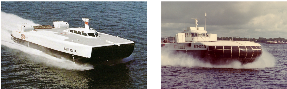
Figure 1.11: The SES-100A (131 ton) and SES-100B (93.4 ton), from left to right. Top speed: 80 and 94 knots, respectively.
