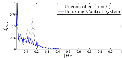
Figure 13: PSD figure of the bow motion with and without the BCS active.
