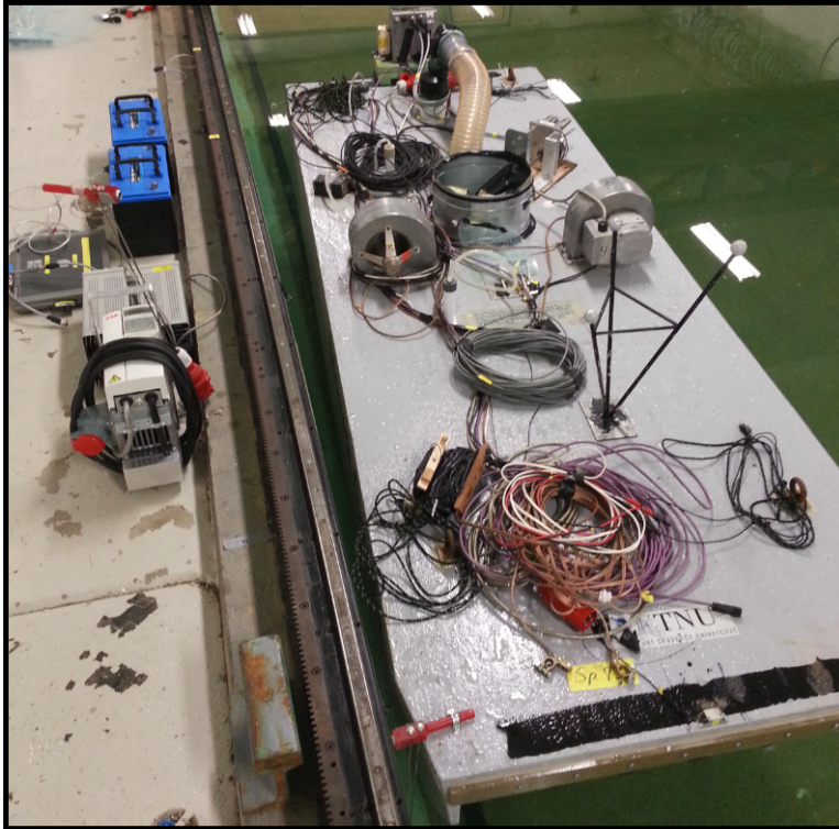
Figure 1.24: Complete model-test equipment.
