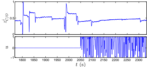
Figure 12: Time series of the bow motion with and without the BCS active. BCS is turned on at t = 2050\text{s} .
