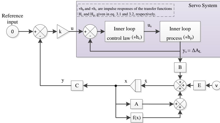
Figure 3.4: A block diagram of the inner and outer loop system
