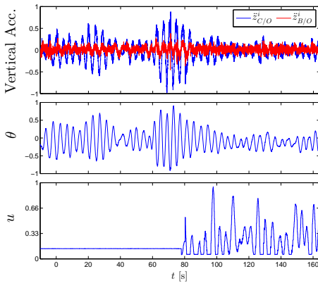
Figure 15: Time series for BCS performance, no turbine contact. Upper: vertical acceleration, middle: pitch angle, lower: controller output. The BCS is turned on at t = 79s .
