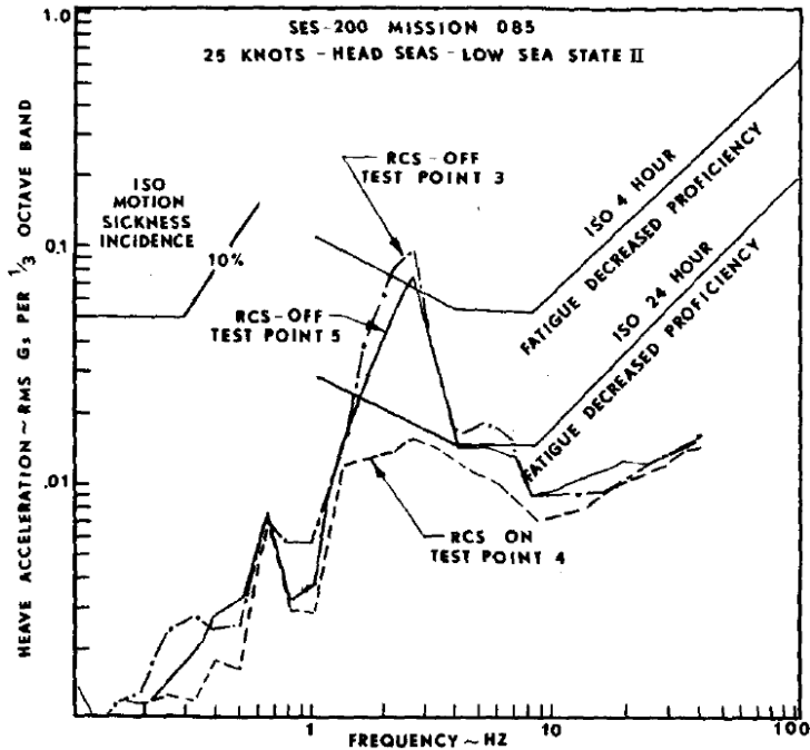
Figure 1.17: Heave accelerations for SES-200 per 1/3 octave band in low sea state II. Picture taken from [16].
