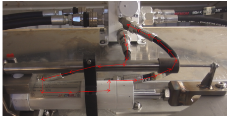
Figure 3.7: Direction of the hydraulic flow.
