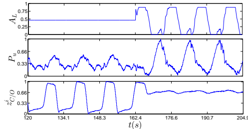
(b) T_p = 11.7\text{s} . BCS is turned on at t = 162\text{s} .
