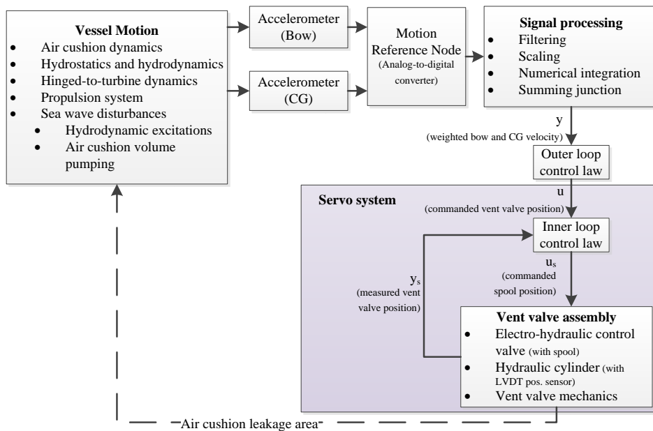
Figure 3.3: Inner and outer loop control system.
