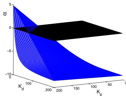
Fig. 7. \alpha - The real value of the complex conjugated pair of poles that determine stability
