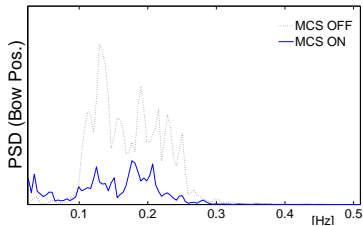
Fig. 11. 135° sea, H_s = 2m , T_s = 7.5s
