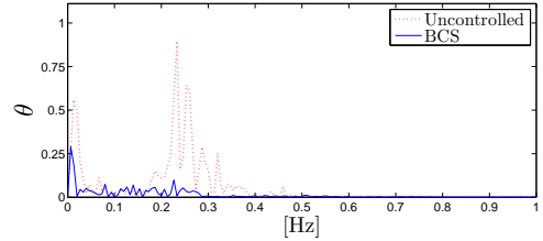
Figure 20: BCS performance, turbine contact, PSD figure for pitch.
