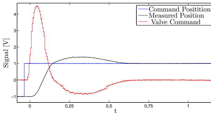
Figure 3.9: A step response is commanded on the input.
