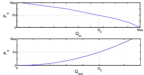
Figure 8: Leakage air-flow characteristics.
