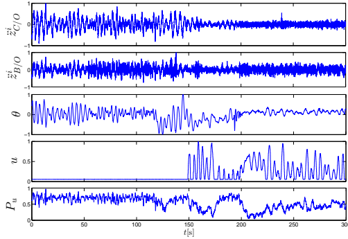
Figure 18: BCS performance, turbine contact, time series for vertical acceleration, pitch, controller output and cushion pressure.
