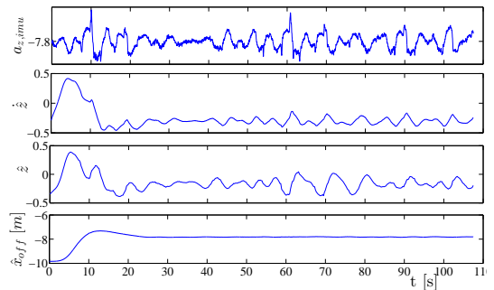
Fig. 10. Bias is added to the accelerometer, b_{z,k} = +2 .
