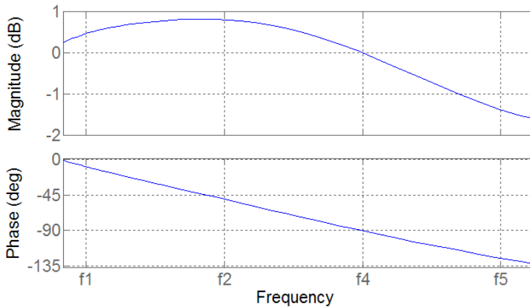
Figure 3.12: Bode Plot - illustrates the frequency response from the input (Command Pos.) to the output (Measured Pos.).
