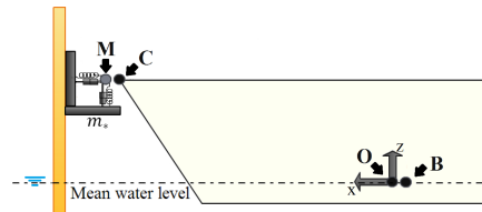
Figure 6: Uncompressed horizontal spring - no contact.
