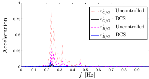
Figure 19: BCS performance, turbine contact, PSD figure for vertical acceleration.
