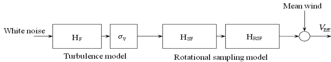
Figure 12: Effective wind model
