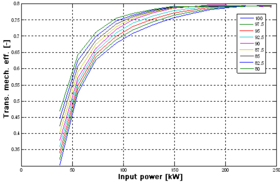
Figure 19: Extrapolated and interpolated transmission efficiency
