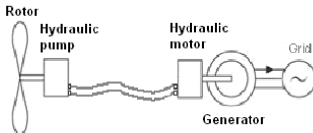
Figure 1, Hydraulic driven generator
