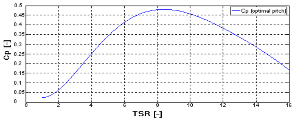
Figure 18: Best Cp curve
