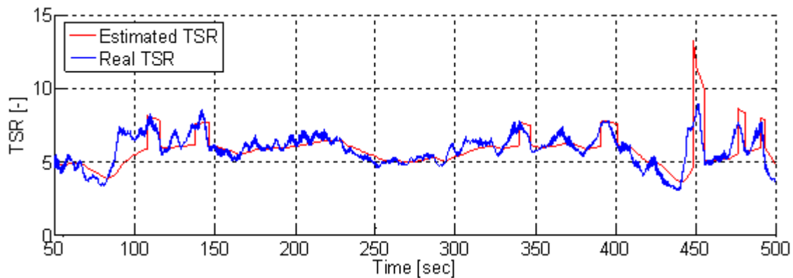
Figure 42: Estimated TSR
