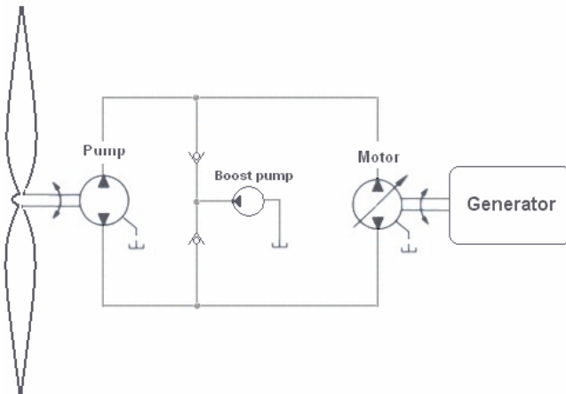
Figure 3: Hydraulic transmission, principle sketch
