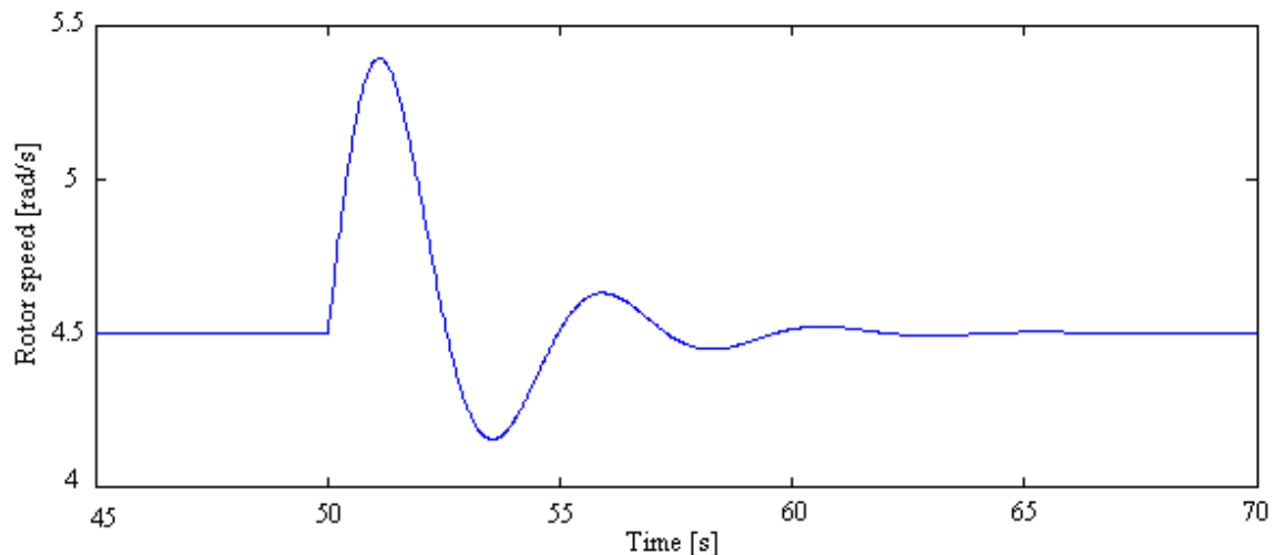
Figure 32: Closed loop torque step response
