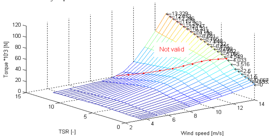
Figure 11: Rotor torque Look up table
