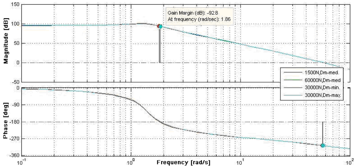
Figure 24: Bode plot without regulator, \omega_p(s)/D_m(s)
