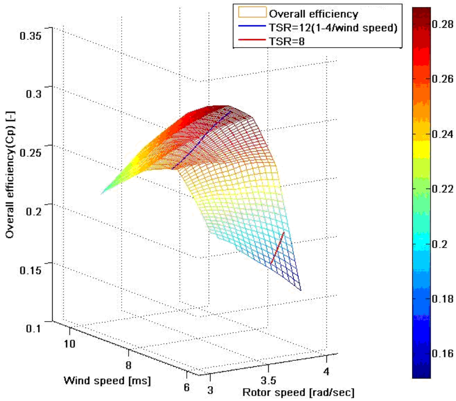
Figure 20: Overall efficiency 3-D plot
