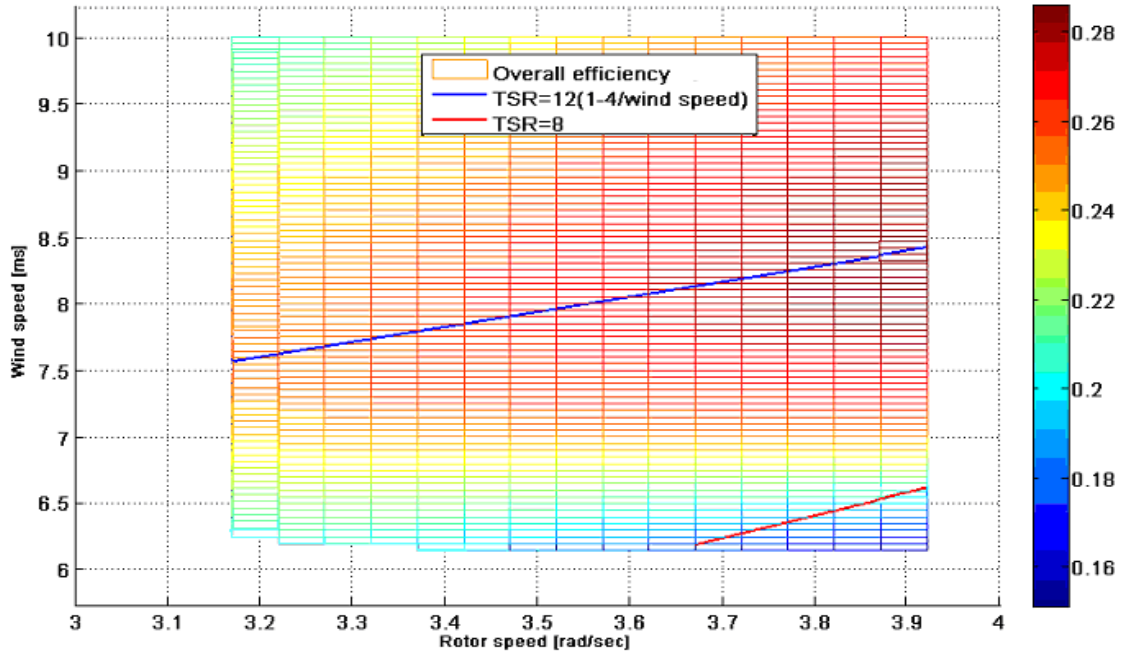
Figure 21: Overall efficiency in wind rotor speed plane
