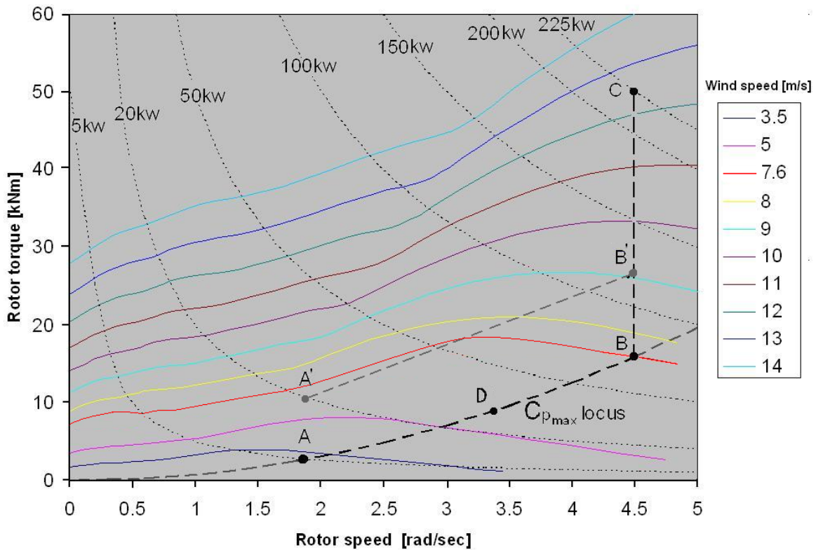
Figure 16: Variable speed variable pitch strategy
