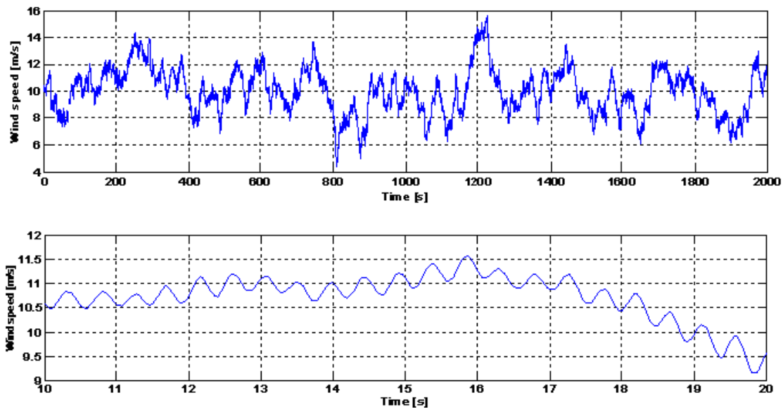
Figure 13: Effective wind speed
