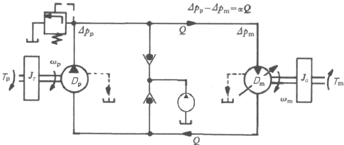
Figure 4: System sketch of hydraulic transmission model
