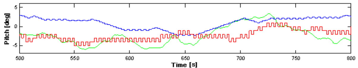
Figure 37: Searching pitch regulator, zoomed view
