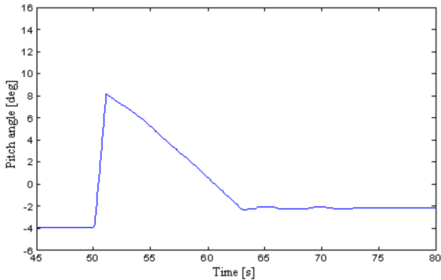
Figure 46: Over-speed pitch action
