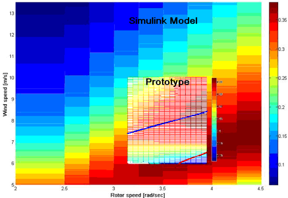
Figure 49: Model efficiency vs. real prototype efficiency
