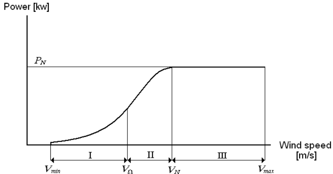
Figure 14: Ideal power curve
