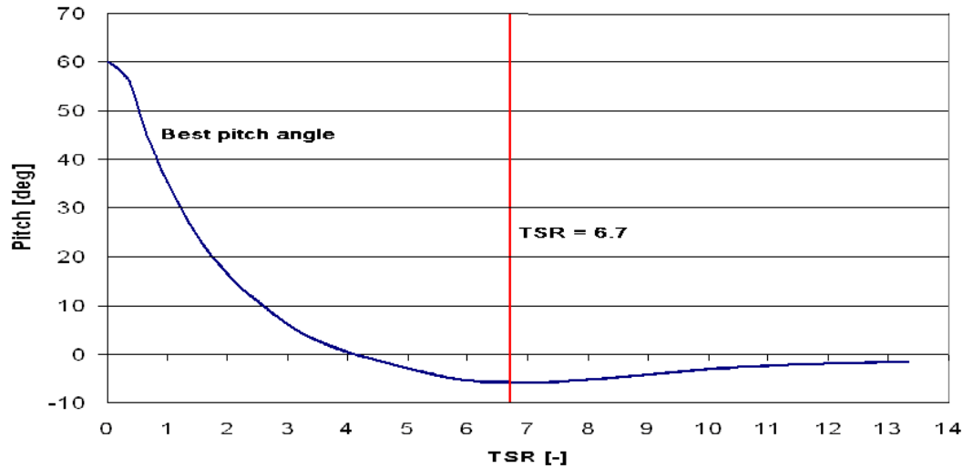
Figure 38: Best pitch angle
