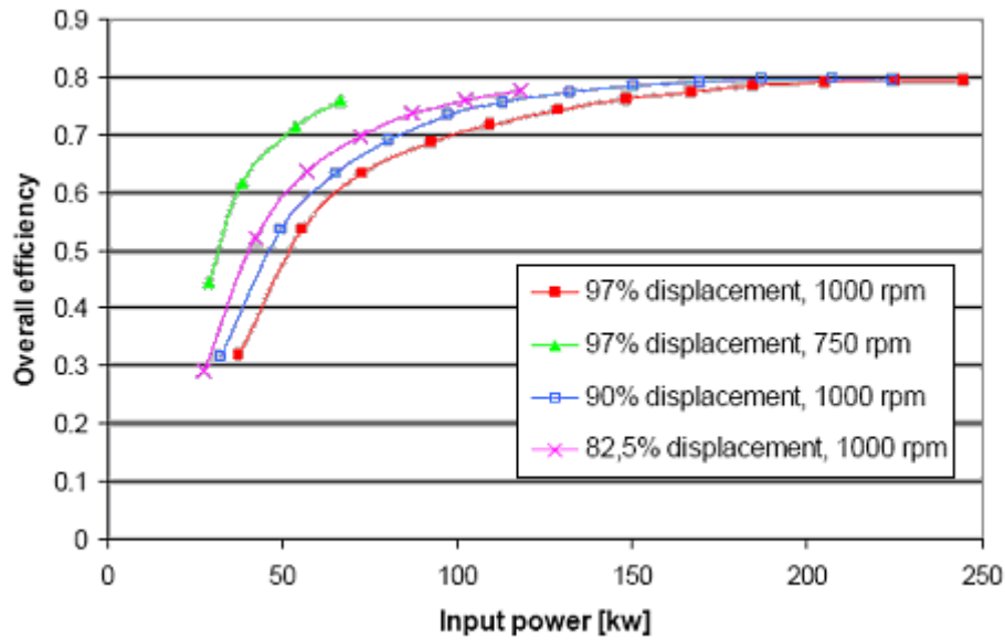
Figure 15: Transmission efficiency [Varpe S. A., 2007]
