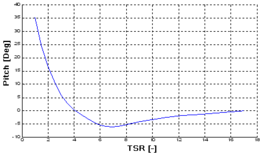
Figure 9: Best pitch
