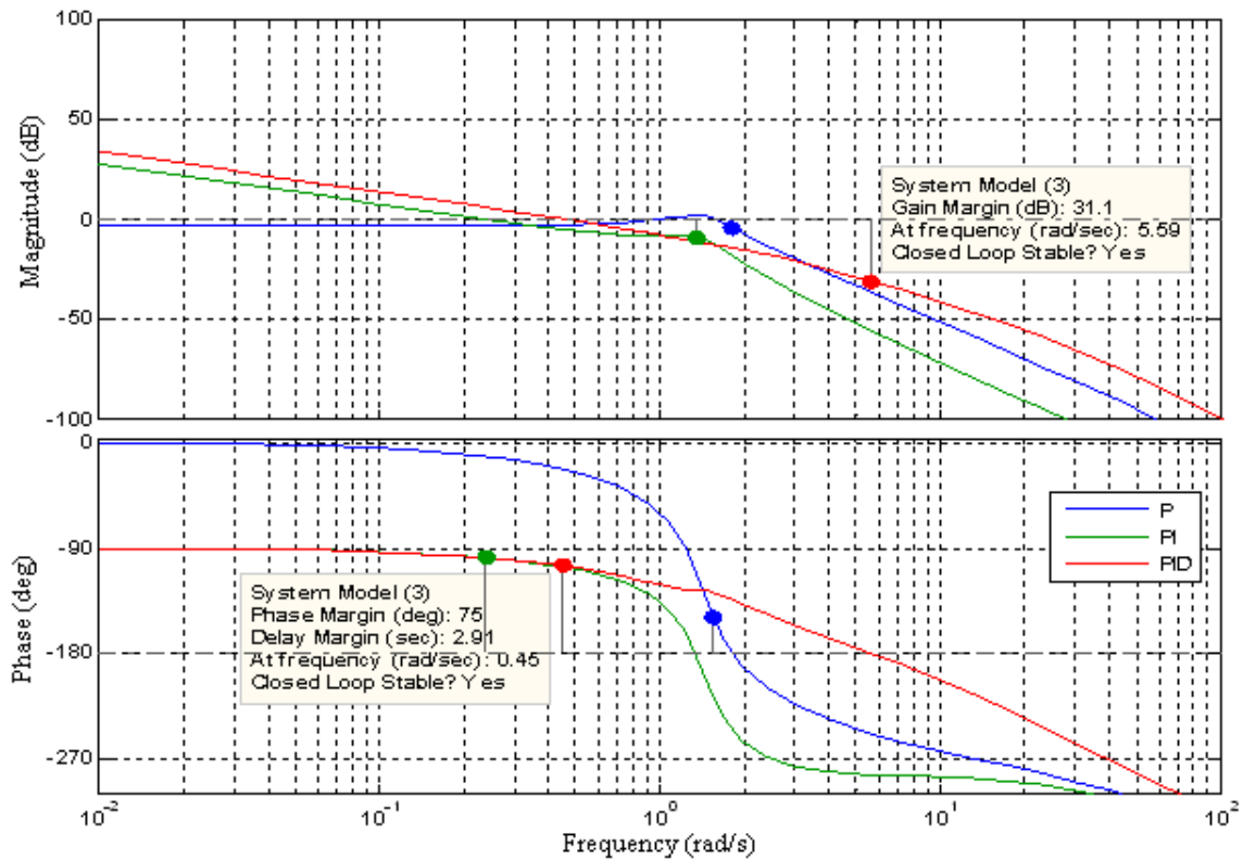
Figure 29: Open loop Bode plot with regulator, \omega(s)/e(s)
