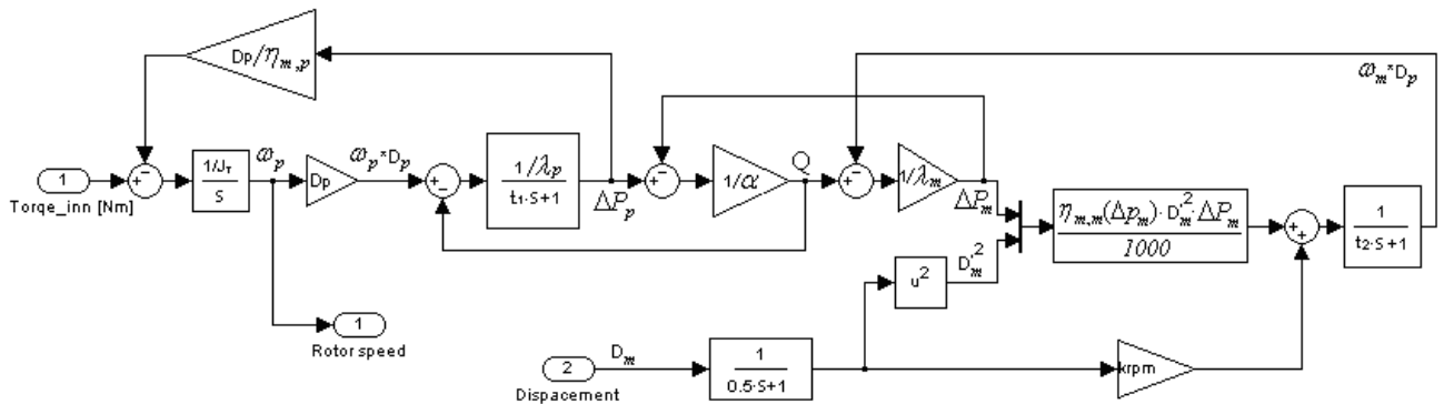
Figure 7: Basic block diagram
