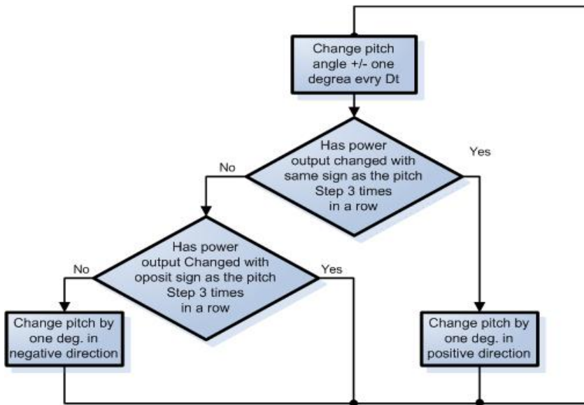
Figure 35: Pitch search flow chart, method 2
