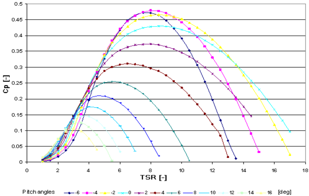
Figure 17: Cp curve [Haugset S. K., 2006]
