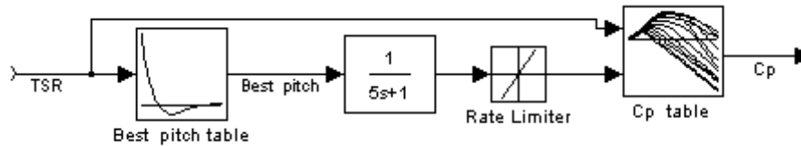
Figure 10: Pitch control model
