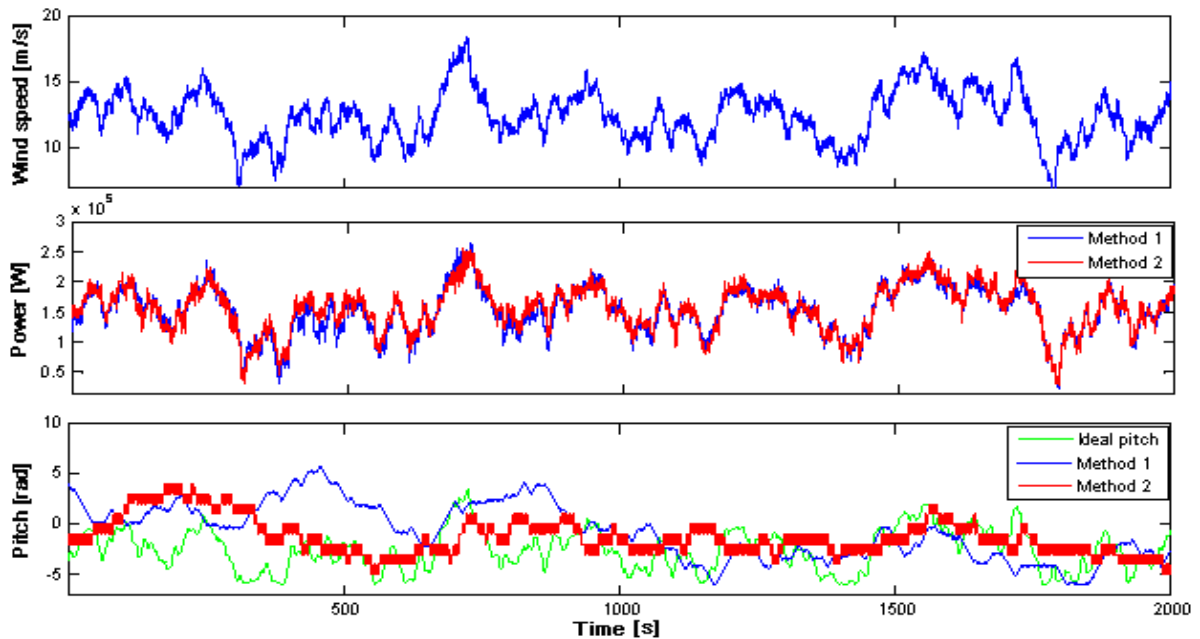
Figure 36: Searching pitch regulator
