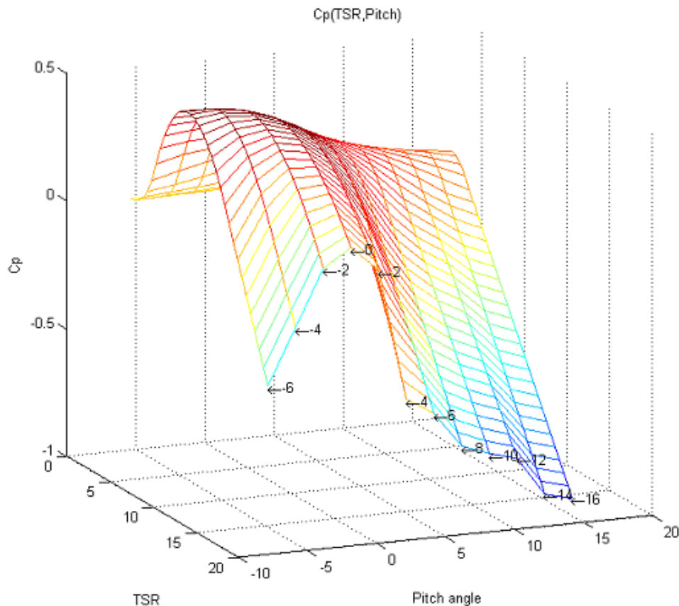
Figure 8: C_p(TSR, Pitch)
