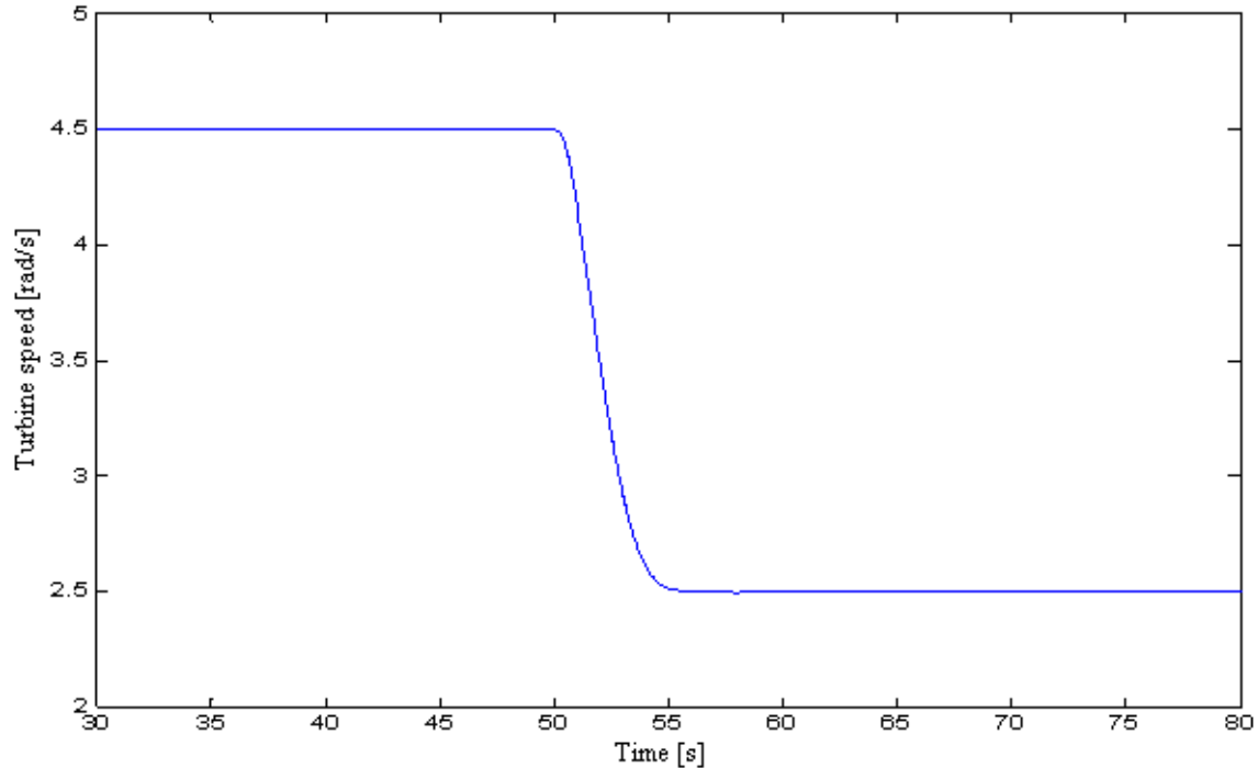
Figure 30: Turbine speed reference step response, PID
