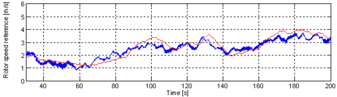
Figure 39: Rotor speed reference
