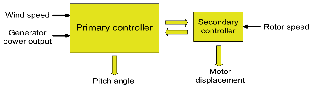
Figure 22: Primary and secondary control
