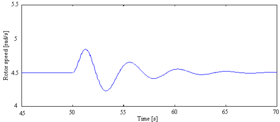
Figure 33: Rotor speed wind step response
