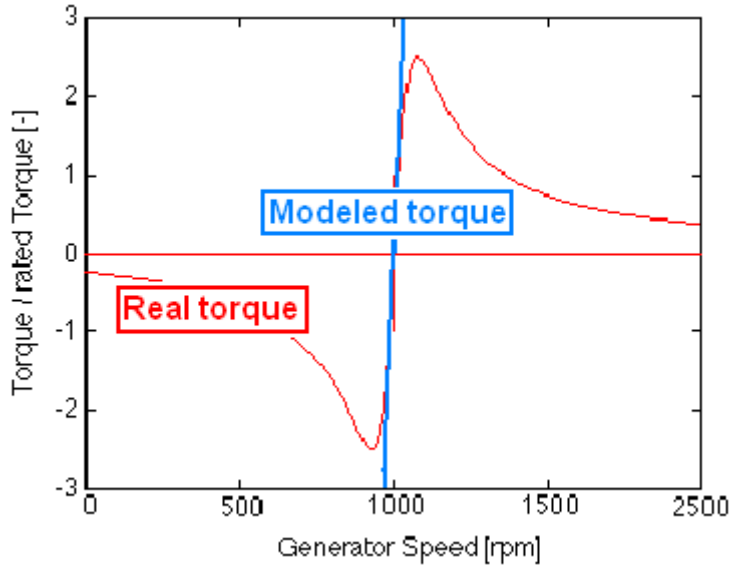
Figure 6: Generator torque vs. speed
