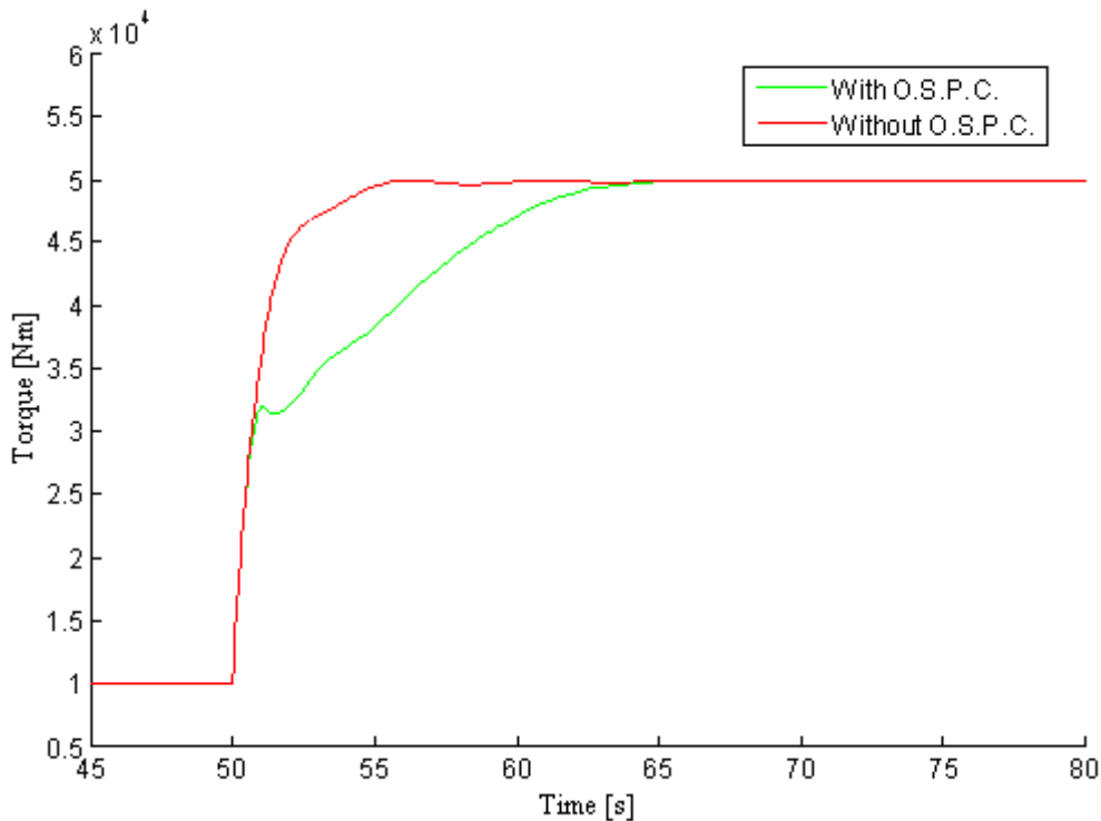
Figure 47: Over-speed torque impact
