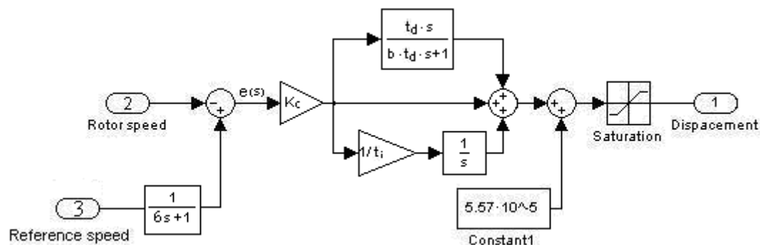
Figure 31: PID controller with damped reference
