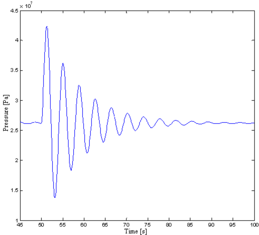
Figure 27: Pump diff. pressure step response
