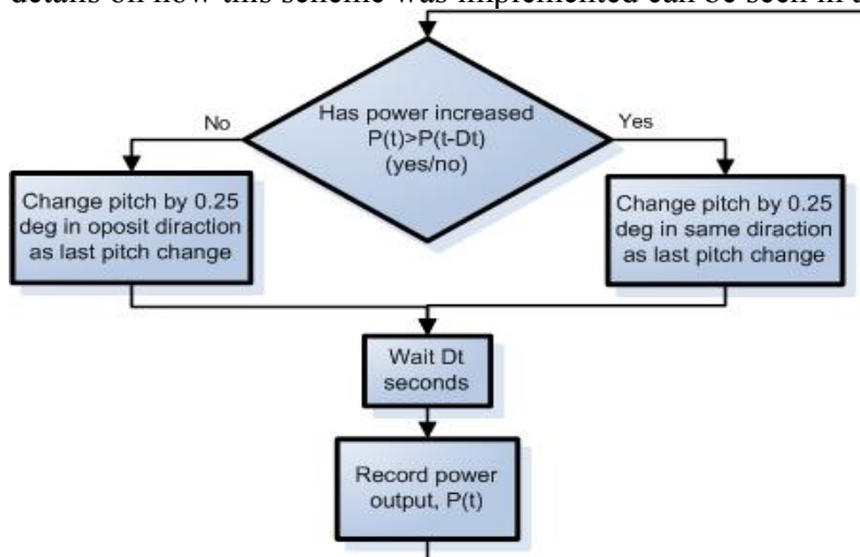
Figure 34: Pitch search flow chart, method 1
