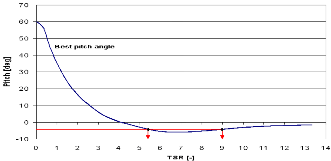
Figure 40: Best pitch angle
