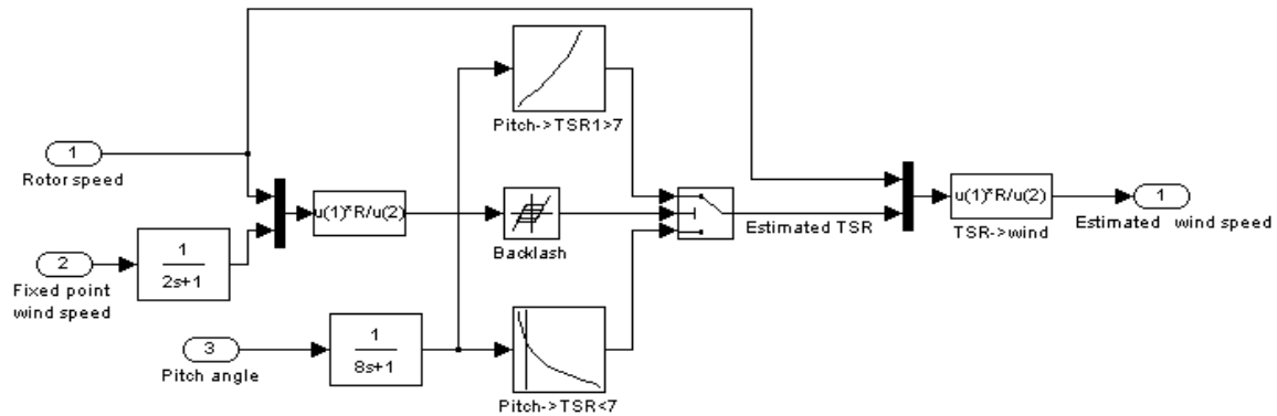
Figure 41: Wind speed estimator
