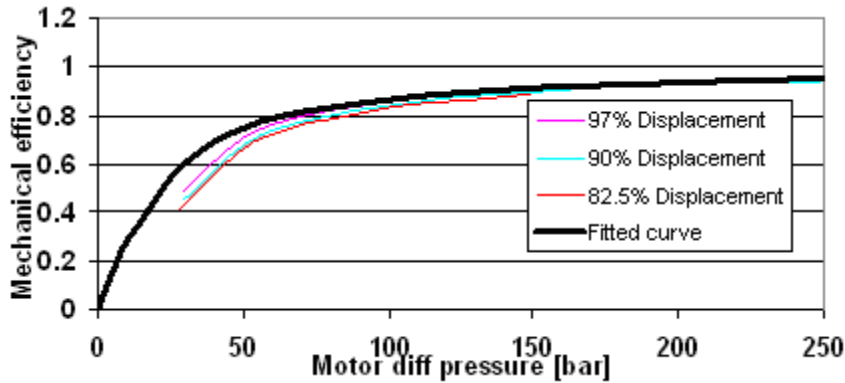
Figure 5: Motor mechanical efficiency
