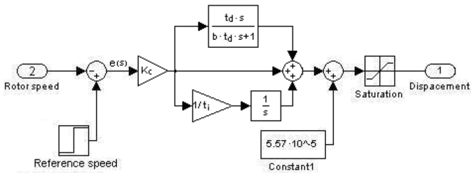
Figure 28: P, PI, PID controller
