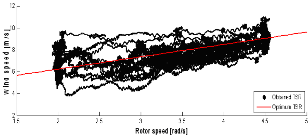
Figure 44: Rotor speed vs. wind speed
