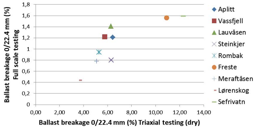
Figure 4.34 Comparison between cyclic triaxial testing and full scale rail track model testing in terms of ballast breakage (0/22.4 mm). Original grading 22.4/63 mm.
