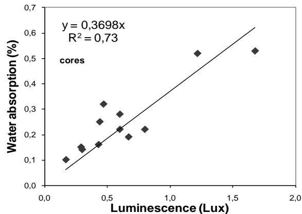
Figure 4.39 A graphic plot between luminescence and water absorption from drilled cores.
