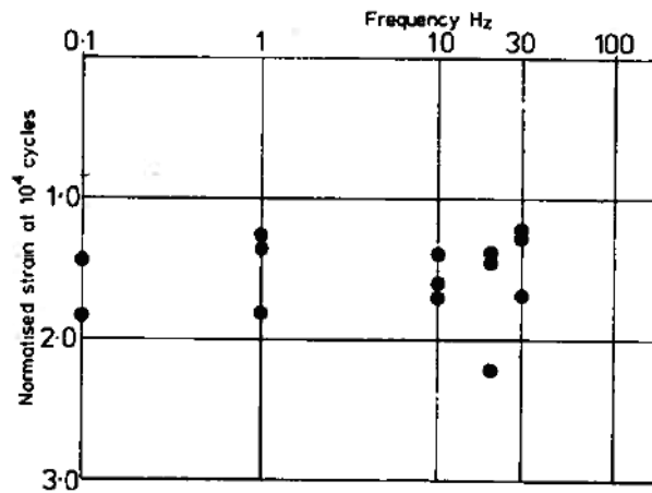
Figure 2.19 The permanent axial strain produced by 10^4 load cycles is plotted against loading frequency (Shenton 1975).
