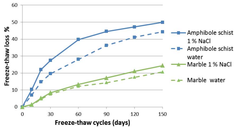
Figure 4.17 Long term weathering curves for two rocks with confirmed low frost resistance (the reference rocks from Beiarn, Nordland county).
