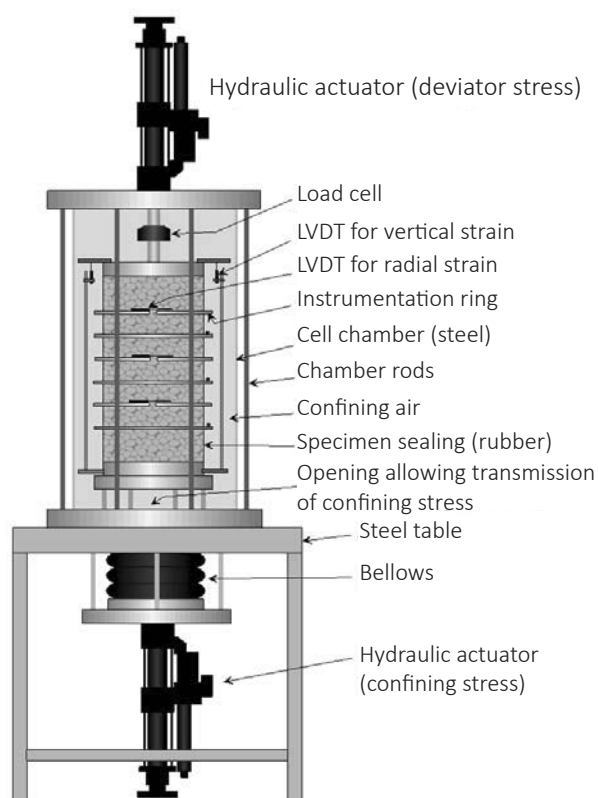
Figure 2.13 The triaxial cell apparatus with specimen, cables not shown (Skoglund 2002).
