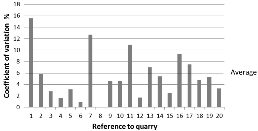
Figure 2.6 Coefficient of variation (COV) for Los Angeles abrasion values (modified after Cuelho et al. 2007).
