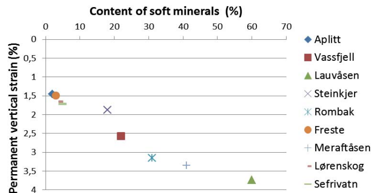
Figure 4.33 Permanent vertical strain from triaxial tests (dry) compared with rocks' content of soft minerals (mica, chlorite and carbonate). Regression coefficient ( R^2 ) is 0.95.
