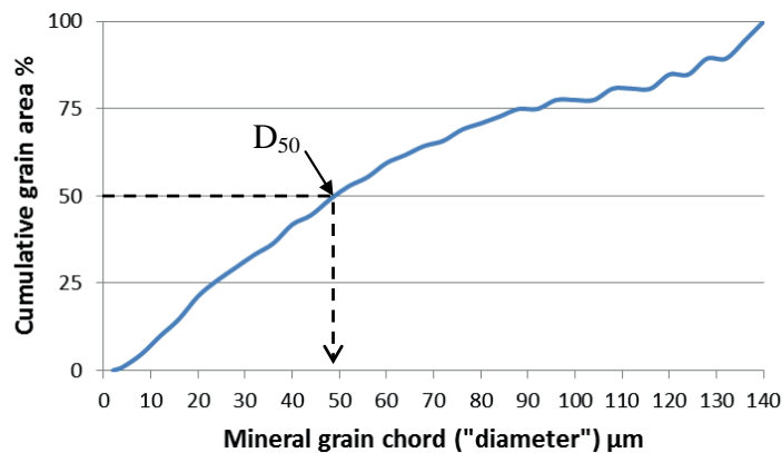
Figure 4.45 An instance of cumulative mineral grain size distribution curve based on calculated mineral grain area (Greenstone, Meraftåsen quarry). The curve is technically comparable with that of sieving of aggregates. D_{50} is about 49 micro meter.
