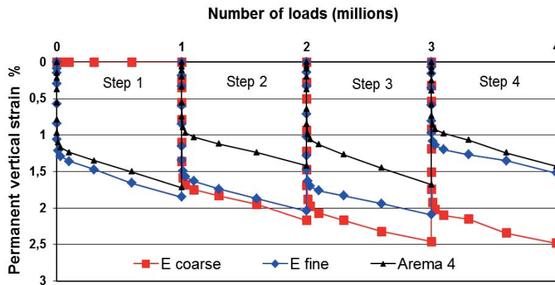
Figure 4.24 Vertical permanent strain against number of loads. Each of the three different gradings (Ecoarse, etc) was tested through four steps and totally subjected to 4 million load applications. Data from step 1 for grading Ecoarse was unintentionally not recorded.
