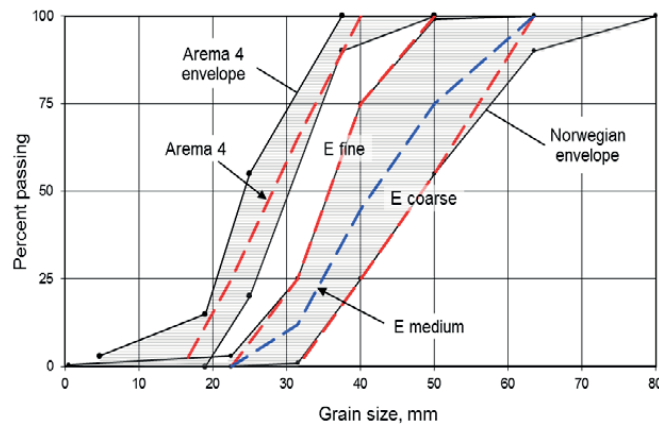
Figure 3.1. Ballast grading curves employed in the large scale triaxial tests and the full scale rail track model test.
