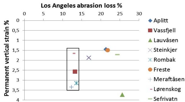
Figure 4.30 Variation of permanent vertical strain in ballast layer from triaxial cyclic loading with dry LAA value (31.5/50 mm)
