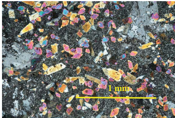
Figure 4.44 Micro image from thin section of a very fine grained greenstone (Meraftåsen 08115-2B) in X-polarised light.
