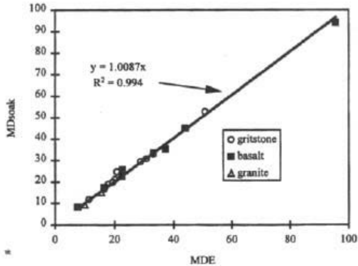
Figure 4.47 Correlation between wet and soaked micro-Deval loss (Woodside and Woodward 1998).
