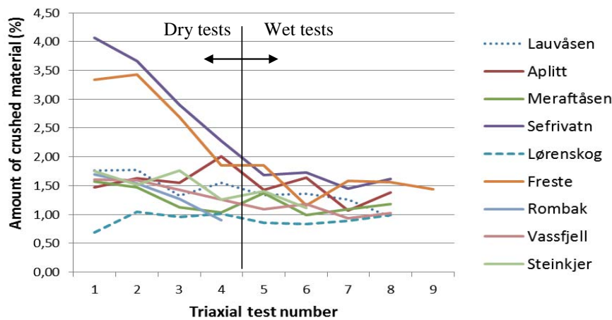
Figure 4.12 Amount of crushed material 0/22.4 mm after each triaxial test. The test fraction at the beginning of each test was 22.4/63.0 mm. Number 1 to 4 represent dry state, and 5 to 8 represent wet state. Mica gneiss from Rombak was tested only in dry state.
