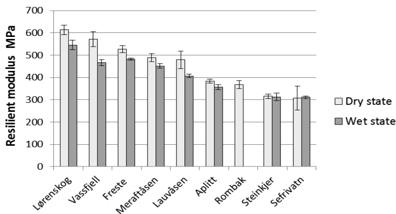
Figure 4.3 Resilient modulus of cyclic triaxial tests in dry and wet state (average of four tests). One standard deviation (+ / -) is added to the columns.
