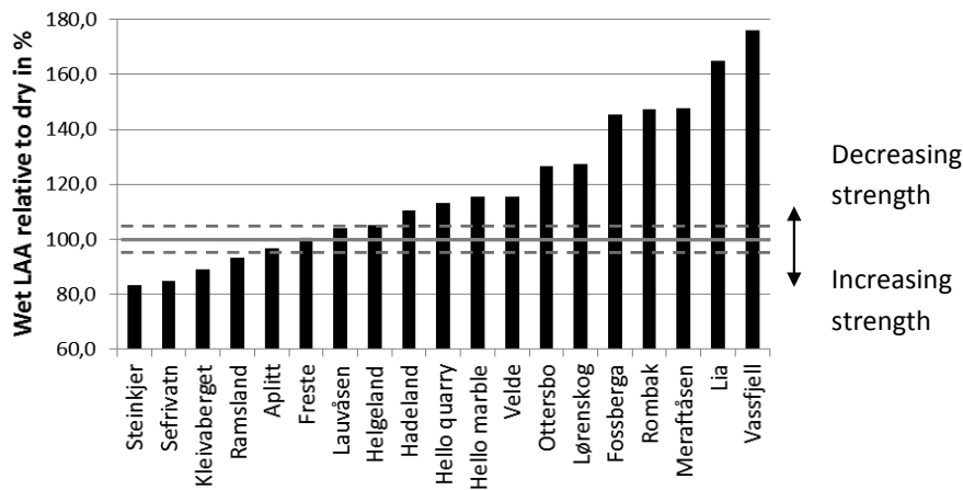
Figure 4.7 Los Angeles abrasion values (31.5/50 mm) of water saturated rocks in per cent of the strength (LAA) of air-dried rocks. Dotted lines suggest one standard deviation (average).
