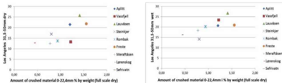
Figure 9: Total amount of crushed material from full scale model test (4x1 million loadings /only dry state) plotted against LAA_{31.5-50mm} . Left: dry state with R^2 = 0.56 . Right: wet state with R^2 = 0.58 , but increase to 0.73 when Freste (medium grained) is removed.
