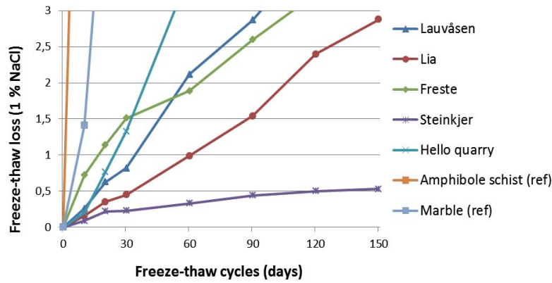
Figure 4.16 Example of long term recording of frost resistance in 1 % NaCl solution. Freeze-thaw loss in % of dry weight. Fraction 8/16 mm and 1 kg sample weight.
