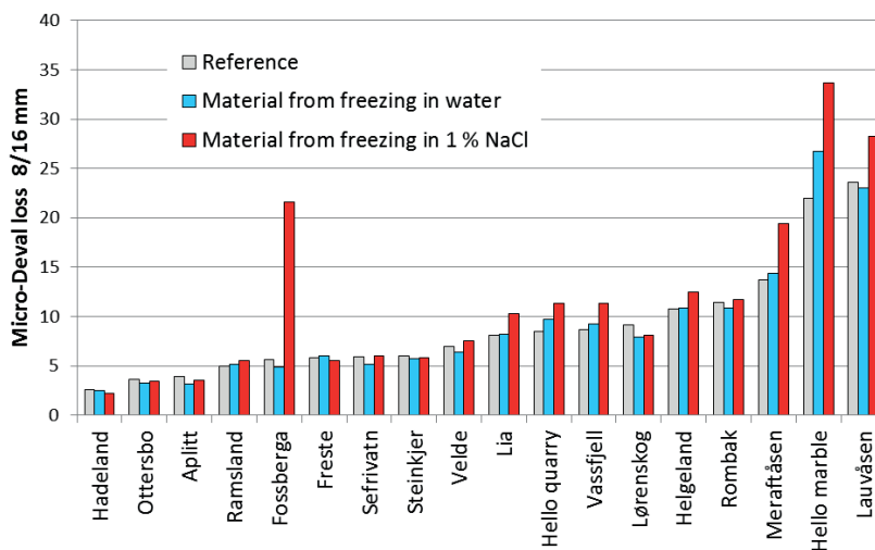
Figure 4.18 Micro-Deval test run on aggregates (8/16 mm) after subjected to 150 freeze-thaw cycles.
