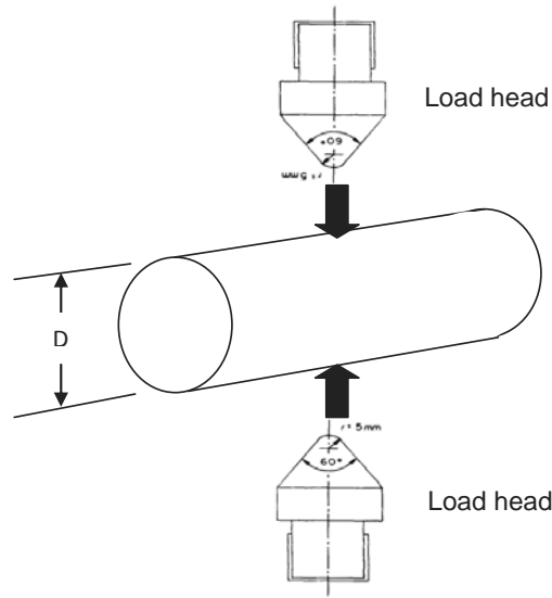
Figure 2.8 Point Load test on drilled cores from rocks. Diameter D was 50 mm.
