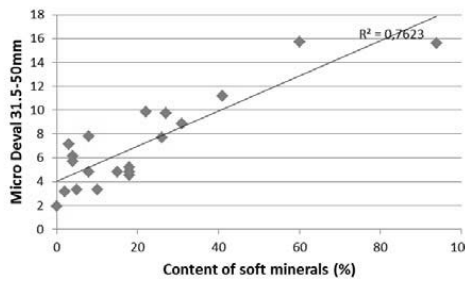
g). Soft minerals (mica, chlorite and carbonate)
