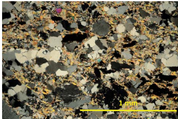
Figure 5: Thin section image of a very fine grained meta sandstone (Steinkjer quarry), X-polarised light.
