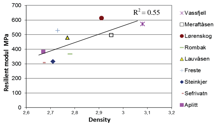
Figure 4.2 Relationship between ballast elastic property and rock density
