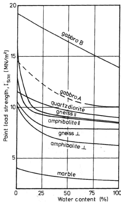
Figure 2.1 Point load strength index ( I_{S(32)} ) as a function of the water content in rock cores (Broch 1974).
