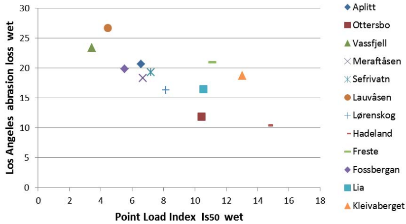
Figure 4.10 Correlation between Los Angeles abrasion 31.5/50 mm and Point Load Index, both wet state.
