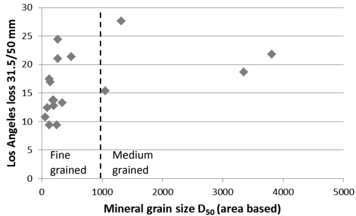
Figure 4.46 The significance of variation in average mineral grain size D_{50} on Los Angeles abrasion loss (mechanical strength).
