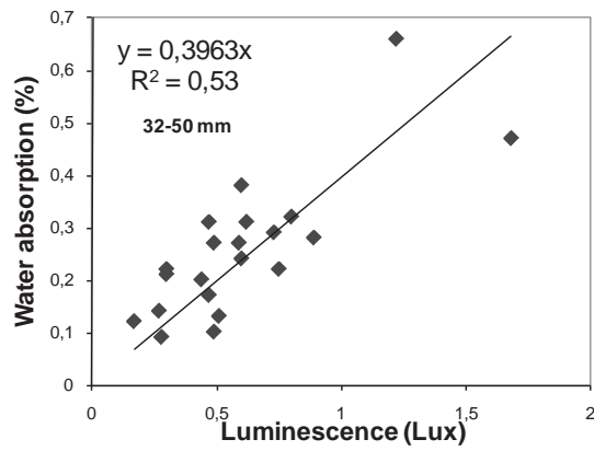
Figure 4: Graphical plot between luminescence and water absorption from fraction 32-50 mm.
