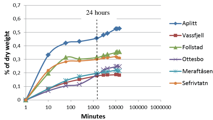
Figure 4.40 Absorption of water on drilled cores. No vacuum used. Test finished after 10 days (Bjerga 2011).
