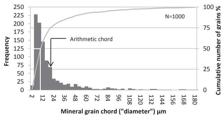
Figure 3: Mineral grain size frequency (the relative values of the different grain-size categories) and cumulative grain size distribution curve for a meta sandstone (Steinkjer quarry) based on measurements of grain "diameter". Average (median) grain size is 10 micro meter (marked on the plot (50%)), arithmetic average (calculated) is 22 micro meter (not multiplied with French factor 1.75)
