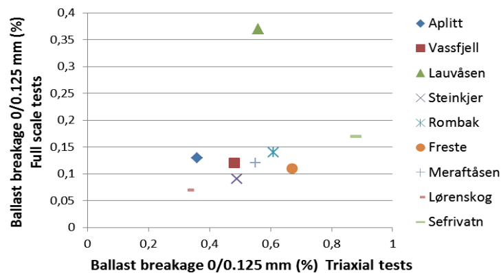
Figure 4.35 Comparison between triaxial testing and full scale model railway track test in terms of ballast breakage (0/0.125 mm). Original grading 22.4/63 mm.
