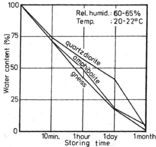
Figure 2.4 Water content in rock cores as a function of storing time in a laboratory environment with relative humidity of 60-65 % and temperature of 20-22 °C (Broch 1974).
