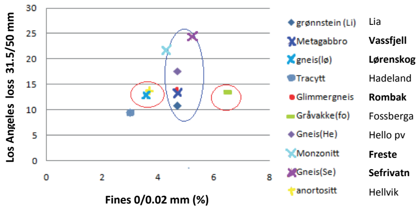
Figure 4.37 Production of fines during Los Angeles abrasion tests versus LAA value for several rock types. Tested fraction was 31.5/50 mm. Modified after Bjerga (2011).
