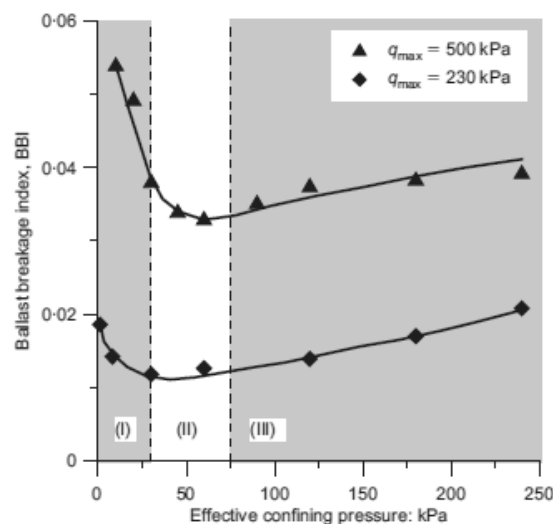
Figure 2.14 Effect of confining pressure on particle degradation at different deviatoric stress levels (Indraratna et al. 2005).
