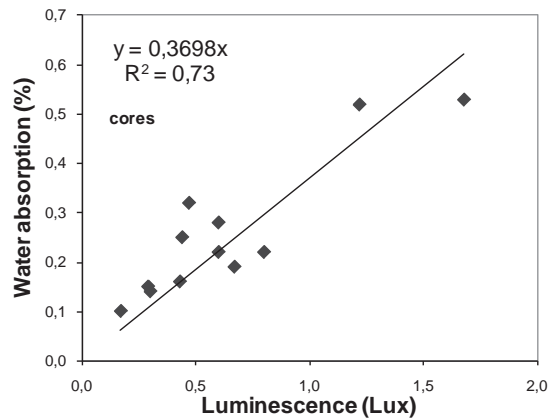
Figure 5: Graphical plot between luminescence and water absorption from drilled cores.
