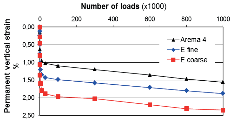
Figure 4.25. Permanent vertical strain against number of loads. Each curve represents the average of four steps, totally 4 x 1 million loadings (average of three steps for grading Ecoarse).
