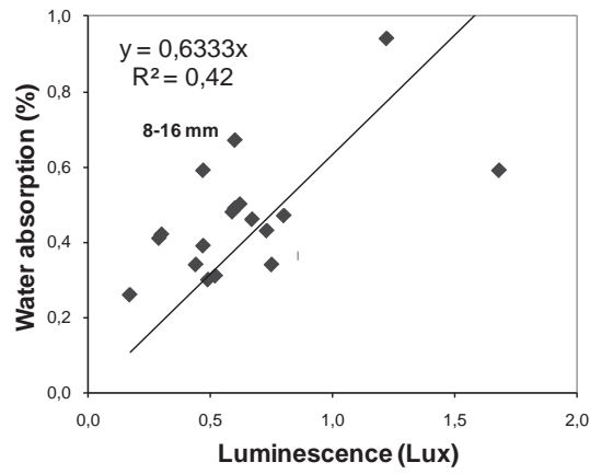
Figure 3: Graphical plot between luminescence and water absorption from fraction 8-16 mm.
