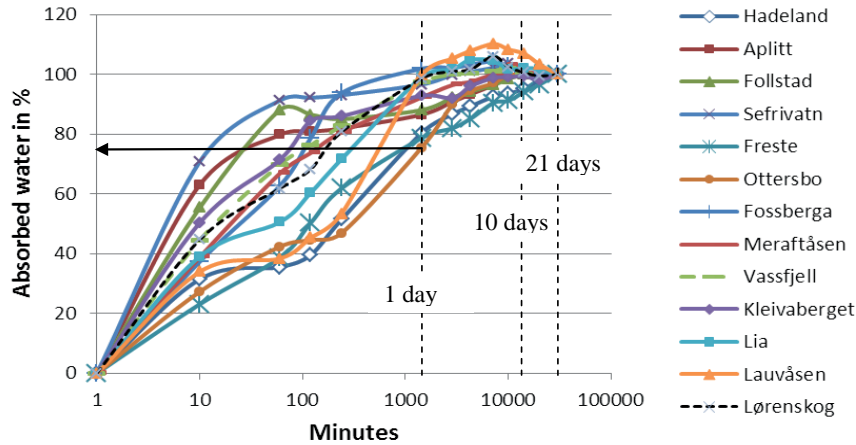
Figure 2.2 Percent absorbed water as a function of time (soaked in water) for drilled cores. Weighing conducted after 10 min, 1h, 2h, 4h, 1d, 2d, 3d, 5d, 7d, 10d, 14d and 21days. Arrow marks 75 % absorption.
