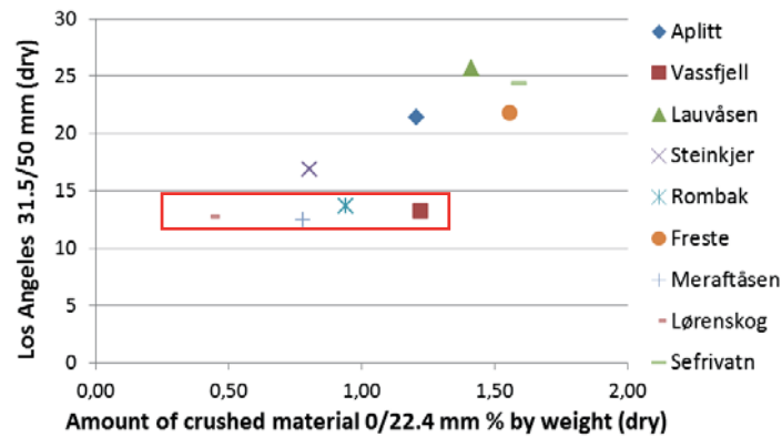
Figure 4.26 Total amount of crushed material from full scale model test (4x1 million loadings and dry state) related to mechanical strength (LAA dry). R^2=0.64 .
