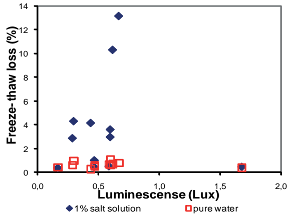
Figure 6: Graphical plot between freeze-thaw loss and luminescence.
