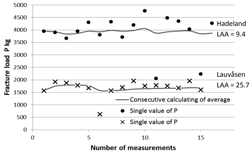
Figure 2.9 Example of calculation of arithmetic value of fracture load P for two rocks as a function of number of measurements. Core diameter D was 50 mm. LAA values relate to fraction 31.5-50 mm.
