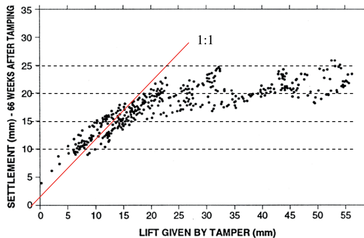
Figure 6.3 Measurement of sleeper settlements 66 weeks after tamping as a function of tamping lift (modified after Selig and Waters 1994).
