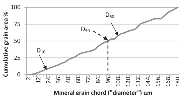
Figure 4: An instance of cumulative mineral grain size distribution curve based on calculated grain area (meta sandstone /Steinkjer quarry). The curve is comparable with that of sieving of aggregates. D_{50} is about 95 micro meter.
