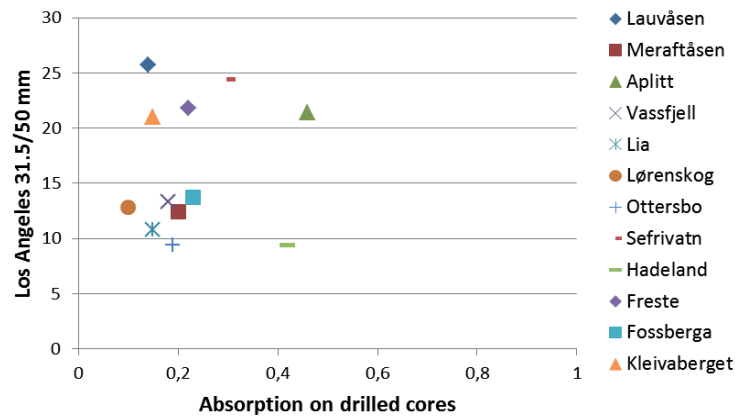
Figure 4.42 Correlation between dry Los Angeles abrasion loss _{31.5/50 \text{ m}} test and water absorption (24h) for drilled cores.
