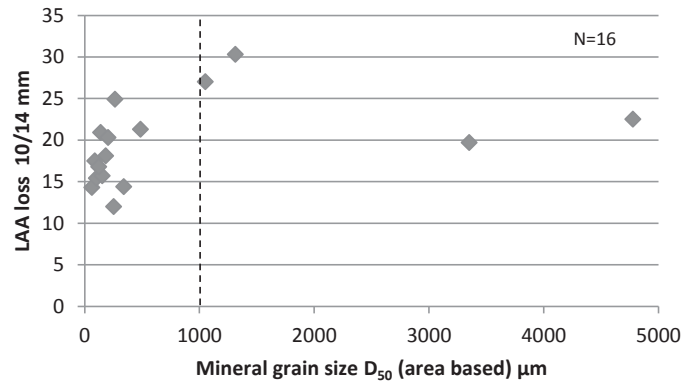
Figure 7: Mineral grain size D_{50} based on grain area plotted against LAA 10/14mm (mechanical strength) loss. Most samples were crystalline rocks and are constituted of mainly hard minerals.
