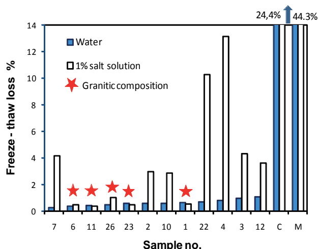
Figure 9: Freeze-thaw results for 14 different rock types (fraction 8-16 mm) after 150 freeze-thaw cycles. C = carbonate rock and M = mica amphibole schist.
