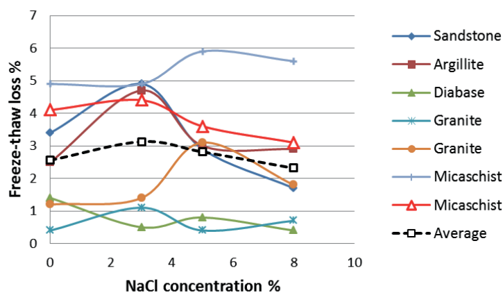
Figure 2.10 Correlation between sodium chloride concentration and freeze-thaw degradation (weight loss), modified after Verbech and Klieger 1957.
