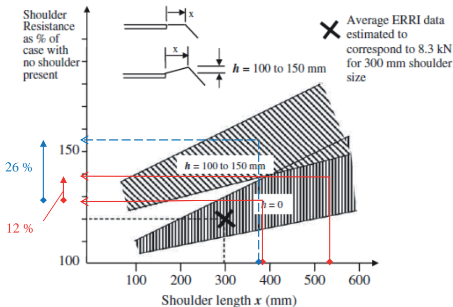
Figure 6.7 Track's lateral resistance depending on the design of the ballast shoulder (modified after ERII 1995).
