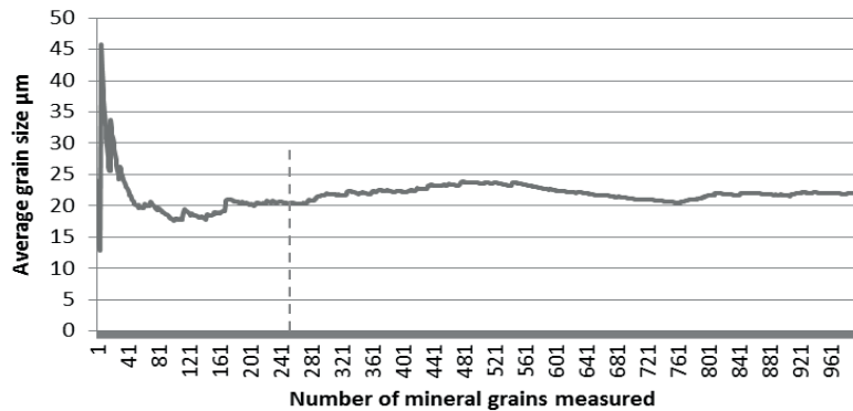
Figure 2: The plot shows the relation between calculated average mineral grain size (arithmetic) and the number of grains counted (Steinkjer quarry). Note that average grain size is stable after approximately 250 measurements.
