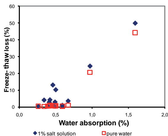
Figure 8: Graphical plot between freeze-thaw loss and water absorption from 8-16 mm fractions including mica schist and carbonate rock.
