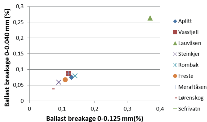
Figure 4.38 Ballast breakage from full scale railway track model test. Original grading 22.4/63 mm. Correlation between fraction 0/0.040 mm and 0/0.125 mm. R^2 = 0.985
