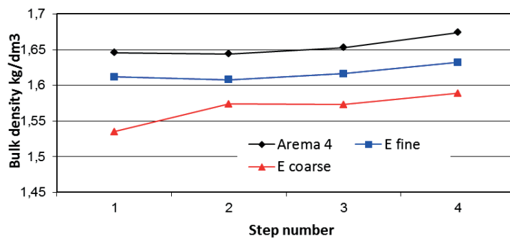
Figure 4.23 Change in specimens' bulk density from step 1 to step 4 (from cyclic triaxial testing in Paper I).
