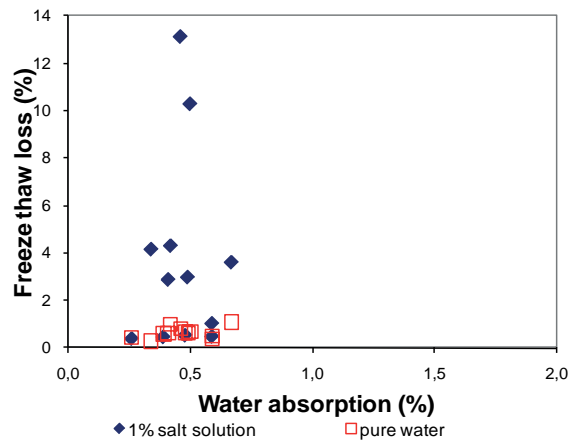
Figure 7: Graphical plot between freeze-thaw loss and water absorption from 8-16mm.
