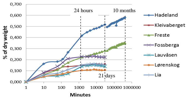
Figure 4.41 Absorption of water on drilled cores. No vacuum used.
