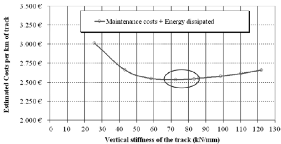
Figure 6.4 Relationship between track stiffness and total costs (Lopez Pita et al. 2004)
