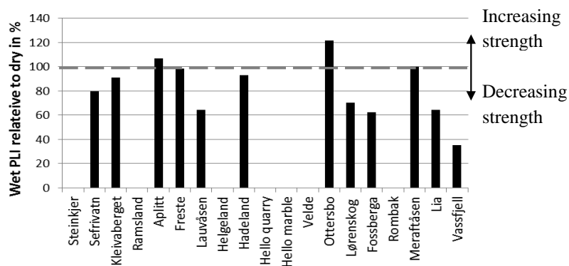
Figure 4.9 Point Load Index (Is 50 ) or tensile strength for water saturated rocks in per cent of the strength of air dried rocks. Drilled core diameter was 50 mm.
