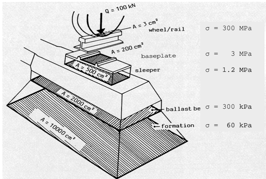
Figure 1.2. Example of pressure distribution from wheel/rail interface down to ballast/subballast interface (modified after Esveld 1989/ Führer 1978).
