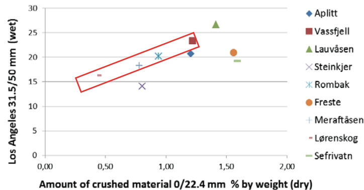
Figure 4.27 Total amount of crushed material from full scale model test (4x1 million loadings (dry state) related to mechanical strength ( LAA_{31.5/50 \text{ m wet}} ). R^2=0.41 .
