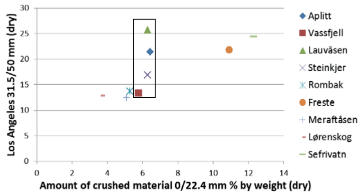
Figure 4.28 Total amount of crushed material from triaxial testing (4x1 million loadings (dry state) related to mechanical strength ( LAA_{31.5/50 \text{ mm dry}} ). R^2=0.77 .
