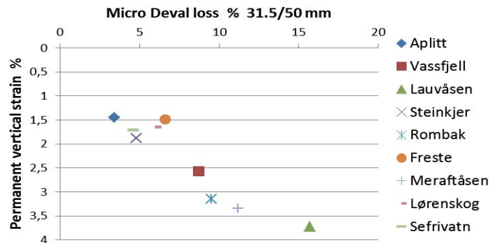
Figure 4.32 Permanent vertical strain from triaxial tests (dry) compared with micro-Deval results. Regression coefficient R^2 is 0.83. R^2 is 0.88 without Freste which can be an outlier (medium grained)
