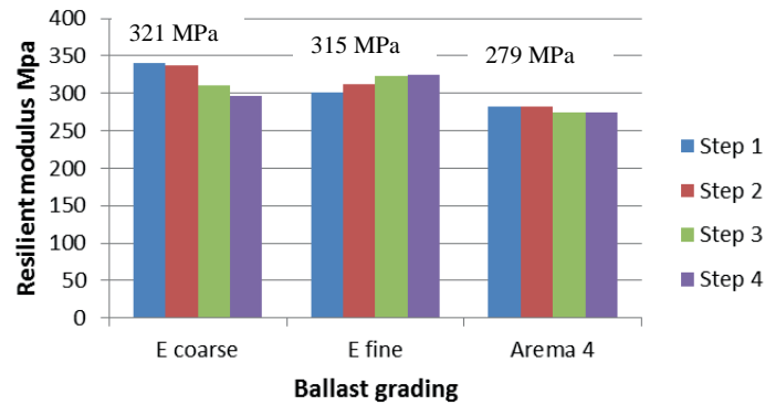
Figure 4.4 Variation of resilient modulus from cyclic triaxial testing with ballast grading. The rock type was Steinkjer meta-sandstone.
