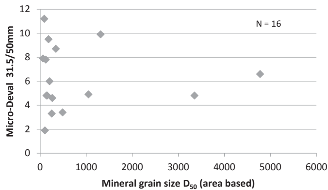
Figure 8: Mineral grain size D_{50} based on grain area plotted against micro-Deval (mechanical strength). Test results from alternative fraction Micro-Deval 10/14mm gave fairly the same correlation.
