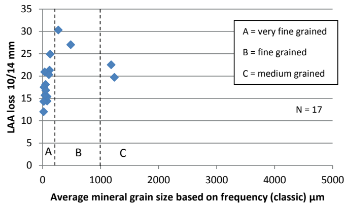
Figure 6: Average mineral grain size (arithmetic) based on grain frequency (classic calculation) plotted against LAA_{10-14 \text{ mm}} . Most samples were crystalline rocks and constituted of mainly hard minerals.
