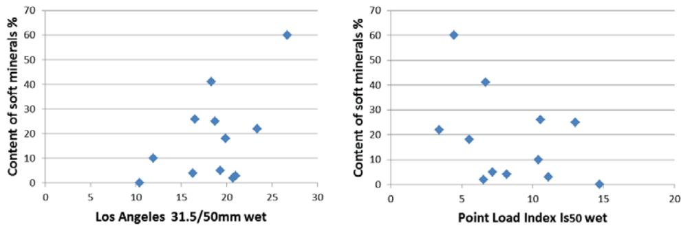
Figure 4.11 Relation between rocks' content of soft minerals and mechanical strength (wet state). Left: Los Angeles 31.5/50 mm wet. Right: Point Load Index Is_{50} wet.
