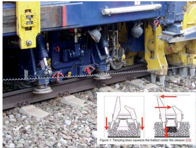
Figure 6.2 Maintenance of track alignment by tamping: 1) lifting track, 2) penetrating tines and 3) squeezing ballast (Selig and Waters 1994).
