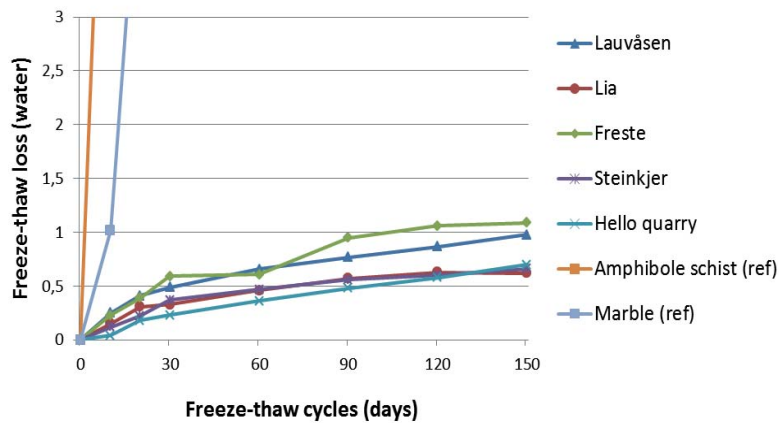
Figure 4.15 Example of long term recording of frost resistance of Norwegian rocks (water). Freeze-thaw loss in % of dry weight. Fraction 8/16 mm and 1 kg sample weight.
