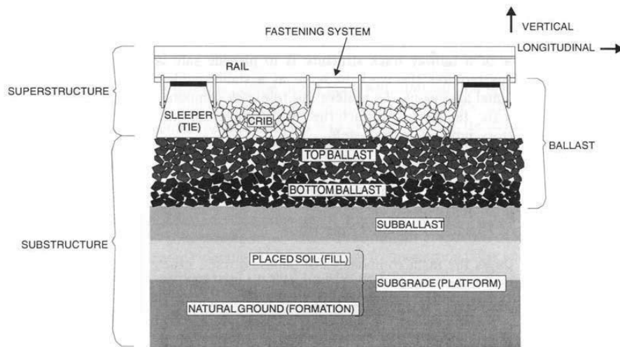
Figure 1.1. Track layout of a typical ballasted track- side view (Selig & Waters 1994).
