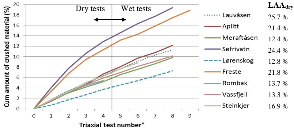
Figure 4.13 Cumulative amounts of crushed material 0/22.4 mm after 8 triaxial tests. Freste was tested 9 times. Test number 1 to 4 represents dry state, and number 5 to 8 represents wet state. Mica gneiss from Rombak was tested only under dry conditions. All rocks are fine to very fine grained except Freste.
