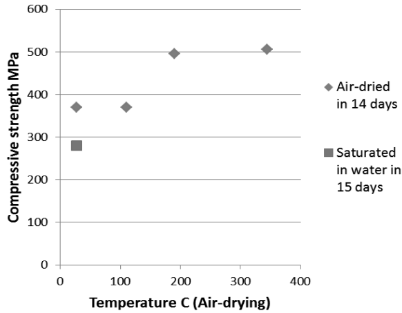
Figure 2.3 Compressive strength of rock cores (diabas) increases with increasing drying temperature ( 27, 110, 190, and 345 °C). Modified after Simpson and Fergus (1968).
