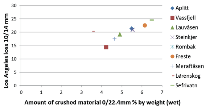
Figure 4.29 LAA values (10/14 mm dry) plotted against ballast breakage (0/22.4 mm) from triaxial tests performed in wet state (4 million loadings). R^2= 0.53 , without Lørenskog 0.97.
