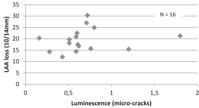
Figure 9: Luminescence against LAA 10/14mm loss (mechanical strength). Test results from alternative fraction LAA 31.5/50 mm gave fairly the same correlation.
