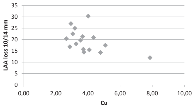
Figure 10: Correlation between slope of grading curve ( Cu = D_{60}/D_{10} ) and LAA 10/14 mm loss (mechanical strength)
