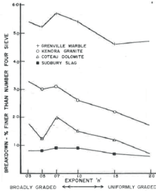
Figure 4.22 Variation in ballast breakage with gradation and with mechanical strength (Raymond 1977b). Number four sieve has 4.75 mm openings.
