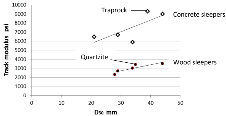
Figure 4.5 Variation in track modulus with ballast particle size. Regression coefficient R^2 for concrete sleepers is 0.55 and for wood sleepers 0.77. Test materials are different types of granite with two exceptions. 1 psi = 6.89 kPa. Modified after Bosserman 1981.
