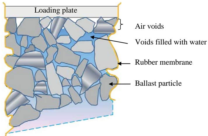
Figure 2.20 Upper section of a wet triaxial test specimen ready for loading, almost completely filled with water.
