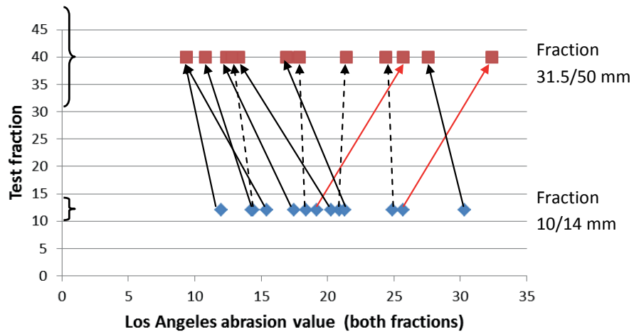
Figure 7.1 Los Angeles abrasion loss for a selection of rocks tested on fraction 10/14 mm and fraction 31.5/50 mm. Black lines marks decreasing values, dotted lines mark indifferent values and red lines mark increasing values when going from fraction 10/14 mm to fraction 31.5/50 mm
