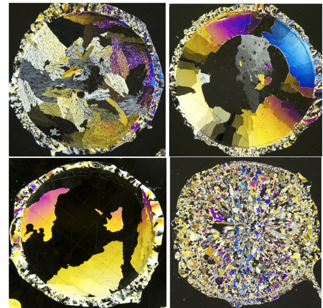
Thin Sections of Different Ice Qualities
