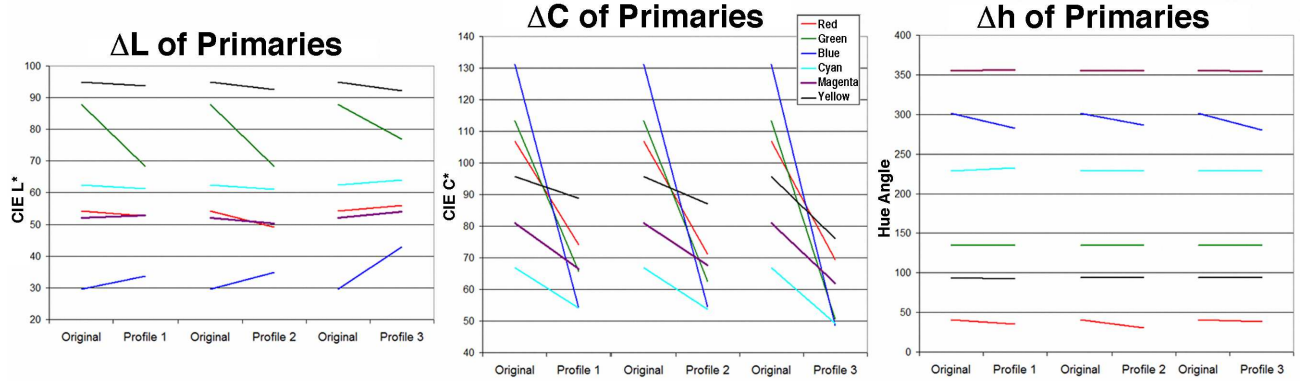
Figure 1. The 6 primaries: CIE \Delta LCh vectors are plotted. The lightness differences are plotted on the left, chroma is in the center and hue to the right. The vectors are similar between the profiles for most colors. In general, profile 3 has the largest compression of lightness and loss of chroma. All three profiles have the greatest change in chroma. There are slight hue shifts, in the counter-clockwise direction, for red (profiles 1 and 2) and blue (all) and in the clockwise direction for cyan (profile 1).
