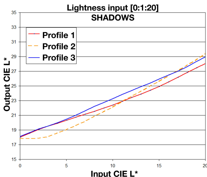
Figure 4. A plot comparing the curves of the low CIE L^* values of the reproductions. Profile 2, maps the very lowest values to the same point, and then has the most aggressive slope. Profile 1, has the most gradual incline, which will improve the shadow details at the expense of contrast.
