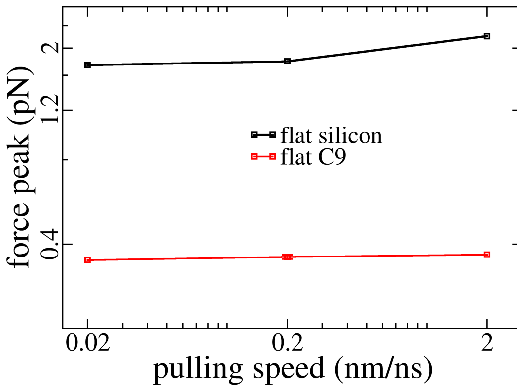
Supplementary Figure S4: Pulling-rate dependency of the highest force observed in the force profiles. The highest force observed in each force profiles were obtained from detaching water droplets from flat surfaces of silicon and C9. The data points at 0.2 nm/ns is the mean value from 5 independent simulations, with error bars showing standard deviations. Each data point at 2 and 0.02 nm/ns was obtained from 1 simulation.
