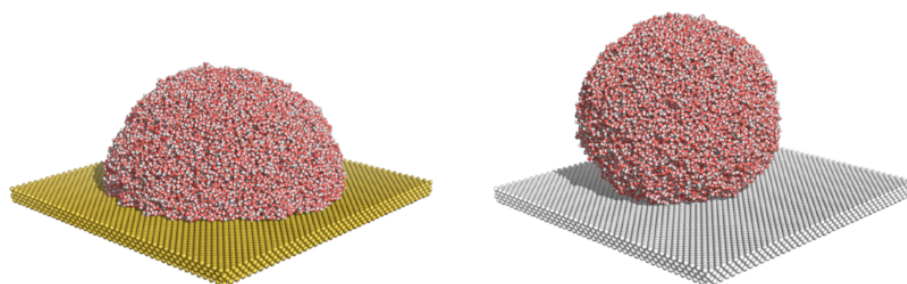
Supplementary Figure S10: Water droplets on flat silicon and C9 surfaces. Silicon atoms are colored in gold and C9 in grey.
