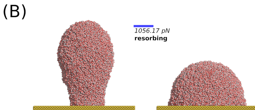
Supplementary Figure S11: Force-clamp MD simulations at different dewetting stages. System snapshots were first taken in the course of dewetting on flat silicon surface at 255 K. The pulling force on the water droplet in each system snapshot was maintained constant in these simulations. (A) Six snapshots were taken for these force-clamp MD simulations. Their corresponding positions in the simulation trajectory were marked in the dewetting force profile by color bars. The constant pulling force applied on the water droplets were given as legends on the left. The final water droplet morphologies, adhering, detaching or resorbing, were also given in the legends. (B) Water droplet resorbing, exemplified by the simulation with constant pulling force of 1056.17 pN. The initial and final snapshots of this simulation system were given on the left and right, respectively. It is clear that there are two forces resisting the droplet detachment, namely droplet shape deformation (increasing droplet surface area) and water-substrate adhesion (decreasing contact area). With the constant loading of the pulling force (force-probe MD simulation), there was an upper-bound of pulling force that over-power the two forces and led to water droplet detachment. In this study, this upper-bound force value was close to the highest force value found in the force profile. The droplet detachment event was not depended on the pulling distance because of the fluid property of the water molecules. The droplet can relax under constant force (force-clamp MD simulation), and allowed water molecules to move back to the hydrophilic Si substrate, which resulted in the whole droplet resorbing back to the substrate.
