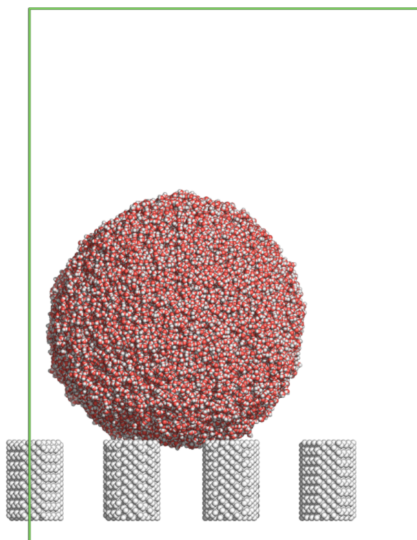
Supplementary Figure S5: Representative snapshot of the water droplet on 4 nm C9 nanopillars at the monostable CB wetting state.
