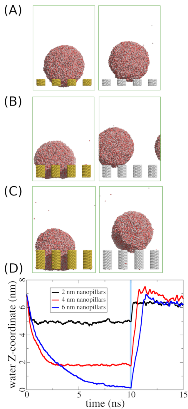
Supplementary Figure S6: Wetting of the water droplet on the silicon nanopillars and spontaneous transition to the monostable CB state on the C9 nanopillars. (A) the water droplet at the WZ state on silicon nanopillars of 2 nm (left), and at monostable CB state after spontaneous transition. (B) and (C) snapshots showing same wetting states in (A) for nanopillars with heights of 4 nm and 6 nm, respectively. (D) the Z-coordinates of the center of mass (COM) of the water droplets in wetting and spontaneous transition simulations on different nanopillars. The heights of the nanopillars in each simulation system were indicated as legends.
