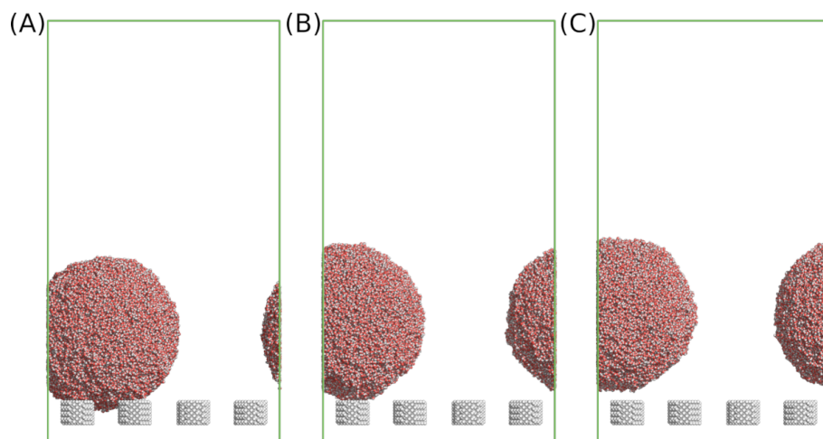
Supplementary Figure S9: Dewetting of a water droplet at monostable CB state. Snapshots of the simulation system at the beginning, middle and end of the dewetting process are shown in (A), (B) and (C), respectively.
