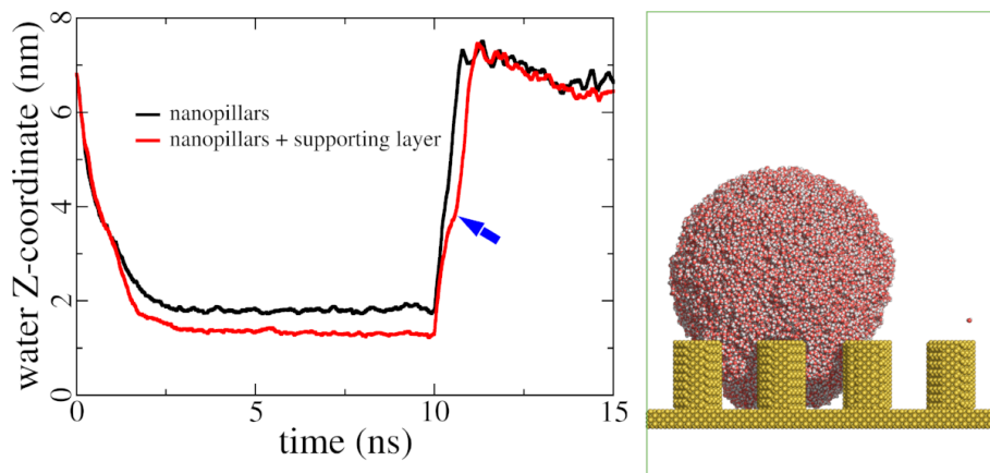
Supplementary Figure S7: Spontaneous transition from the WZ to the monostable CB state on nanopillars with and without underneath supporting layer. A supporting silicon atom layer with thickness of 1 nm was first added to the underneath of silicon nanopillars with heights of 4 nm, as the system snapshot shown on the right. The water droplet was let to adsorbed onto these nanopillars for 10 ns. The substrate atoms were then switched at 10 ns to be C9 for probing spontaneous wetting transition. Comparing to the nanopillars without a supporting atom layer, the water droplet adsorbed further onto the substrate and had a lower COM coordinate at the final adsorbed state. A supporting layer can slightly slow down the wetting transition process, as indicated by the blue arrow in the plot and the system snapshot shown on the right.
