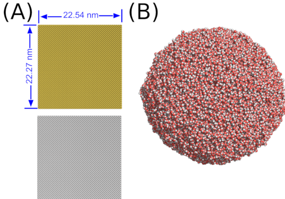
Supplementary Figure S1: Atomistic models of flat substrates and the water droplet. (A) top views of the flat silicon and the C9 substrates. Both substrates have the same thickness of 1 nm. The two substrates have the same surface area, as the dimension indicated in the figure. (B) the water droplet model consists of 50066 tip4p water models (200,132 atoms in total).
