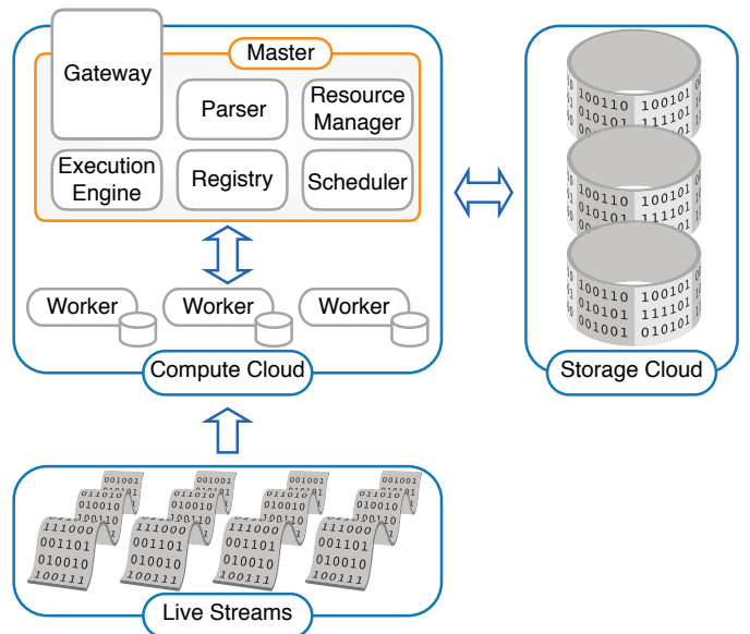
Figure 5: Distributed Stream Engine Architecture
