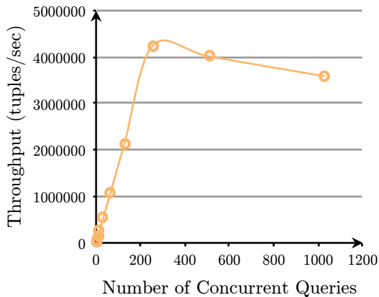
Figure 15: Effect of parallelism on live-stream queries
