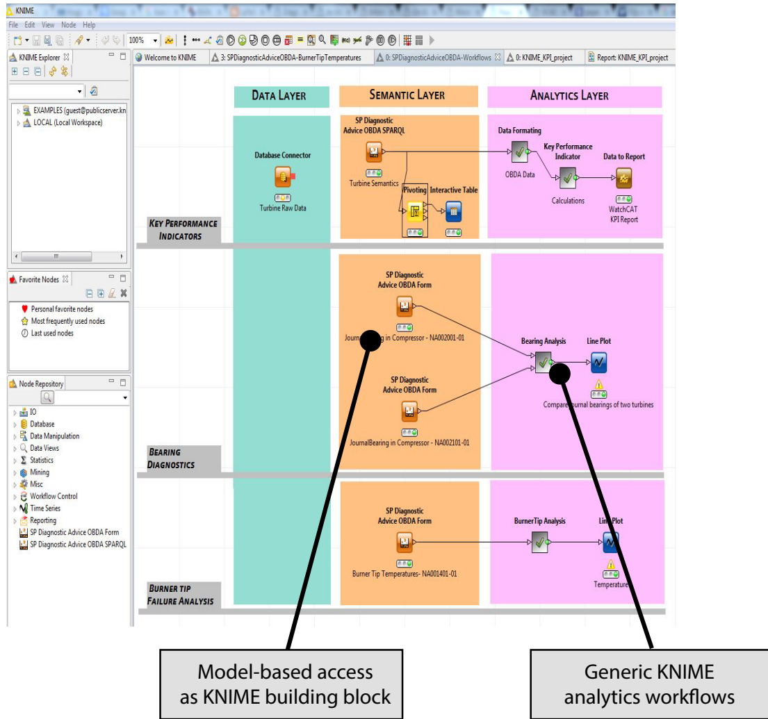
Figure 11: Optique integration with KNIME
