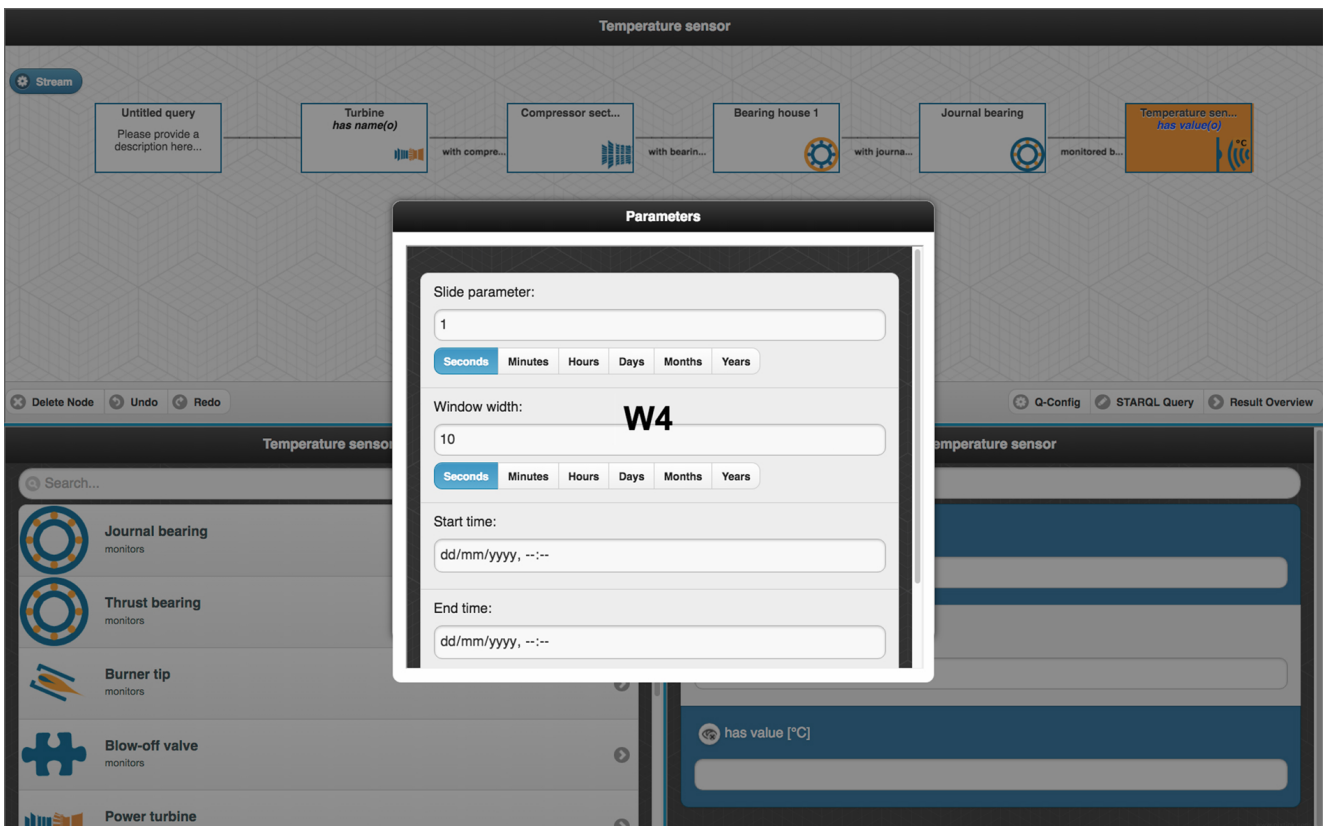
Figure 8: OPTIQUEVQS interface – parameter selection.
