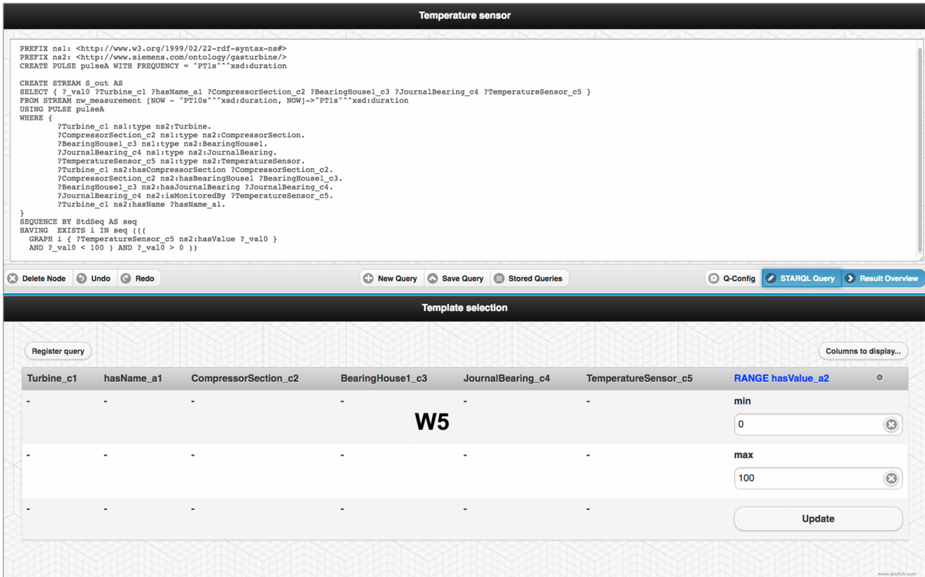
Figure 9: OPTIQUEVQS interface – template selection and the generated STARQL query.
