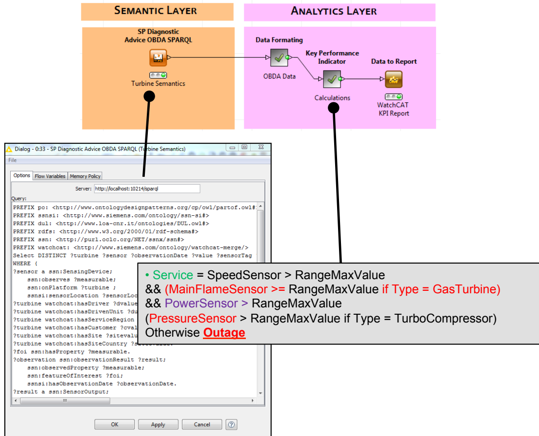
Figure 12: Optique integration with KNIME
