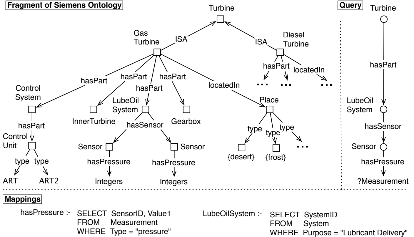
Figure 4: Simplified Siemens ontology and mappings, example query
