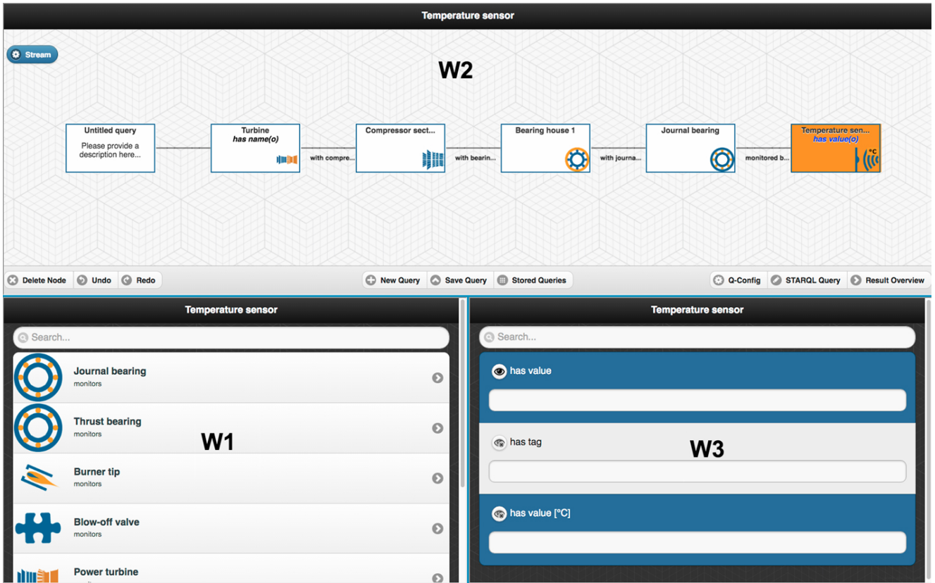
Figure 7: OPTIQUEVQS interface – dynamic properties are coloured in blue.
