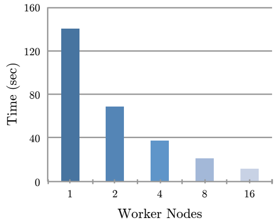
Figure 16: Effect of parallelism on hybrid queries
