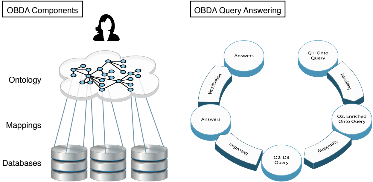
Figure 3: OBDA: components and a general idea of query processing
