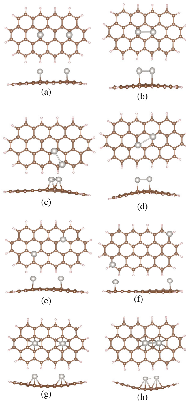
Fig. 4 Stable configurations for the Pt dimer (parallel adsorption) and two Pt atoms on C_{40}H_{16} molecule. Gray, brown and pink circles indicate Pt, C, and H atoms, respectively. a, b, c are bridge sites, d, e, f are top sites and g, h are hollow sites
