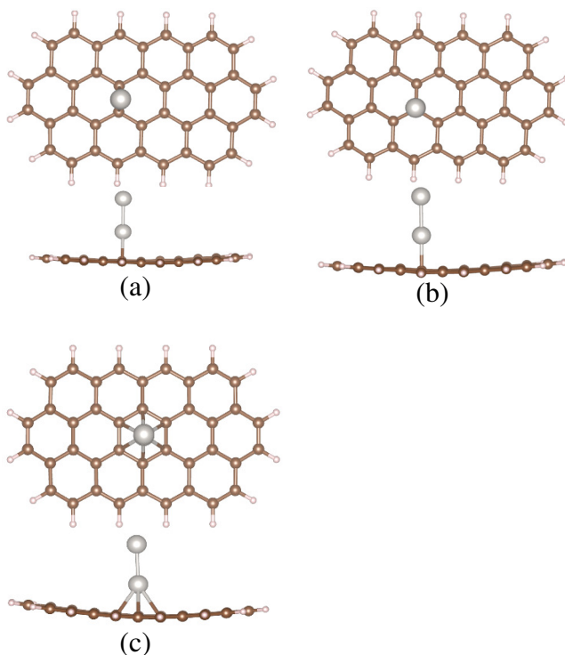
Fig. 5 Stable configurations for the Pt dimer (upright adsorption) on the C 40 H 16 molecule. Gray, brown and pink circles indicate Pt, C, and H atoms, respectively. a, b, c are bridge, top and hollow sites, respectively.
