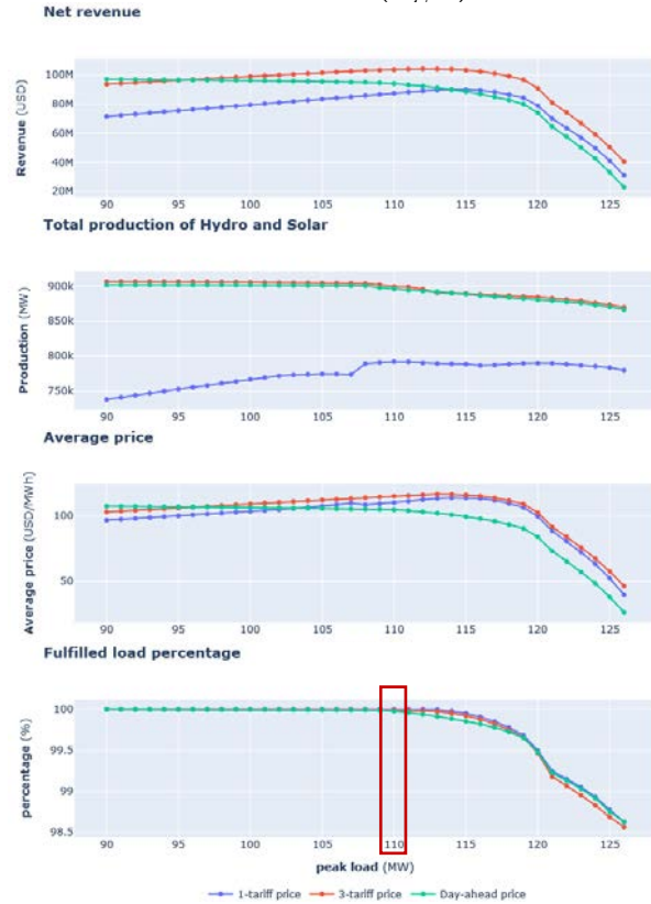
Fig. 8. Net revenue, total production, average price, and fulfilled load percentage with an increase of load obligation from 90 MW to 126 MW
