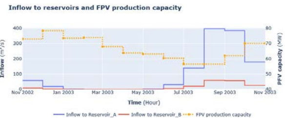
Fig. 7. Monthly inflow to reservoirs and average FPV production capacity
