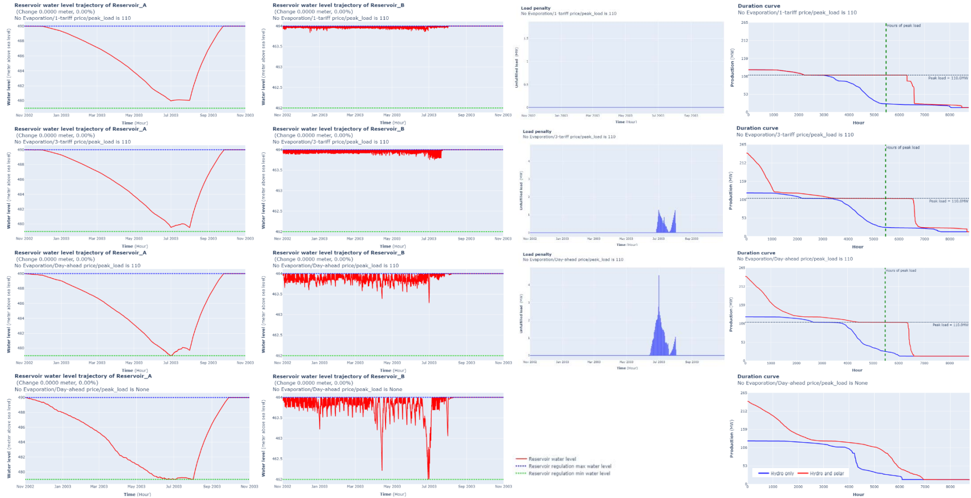
Fig. 10. Reservoir water level trajectories, load penalty, and production duration curves under three types of pricing regimes
