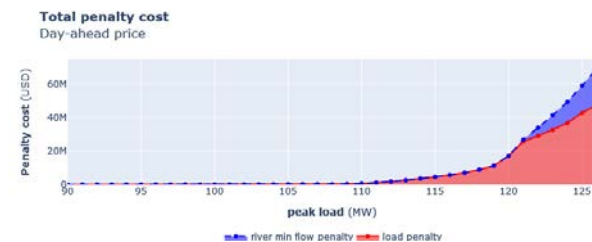
Fig. 9. Total penalty cost under day-ahead price with an increase of load obligation from 90 MW to 126 MW
