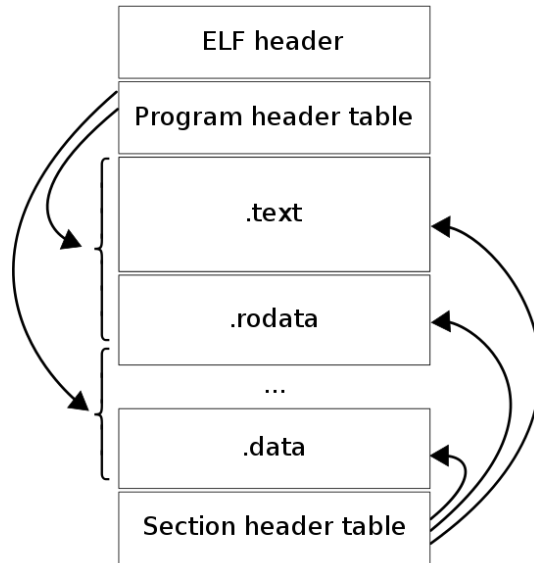
Figure 1: ELF file structure [6].
