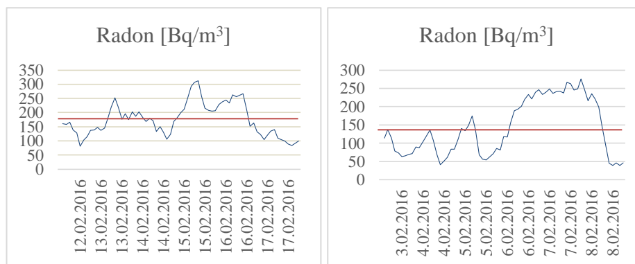
Figure 4. Time-dependent radon concentration (blue line) with mean value (red line): Neven (left) and Kolibri (right)
