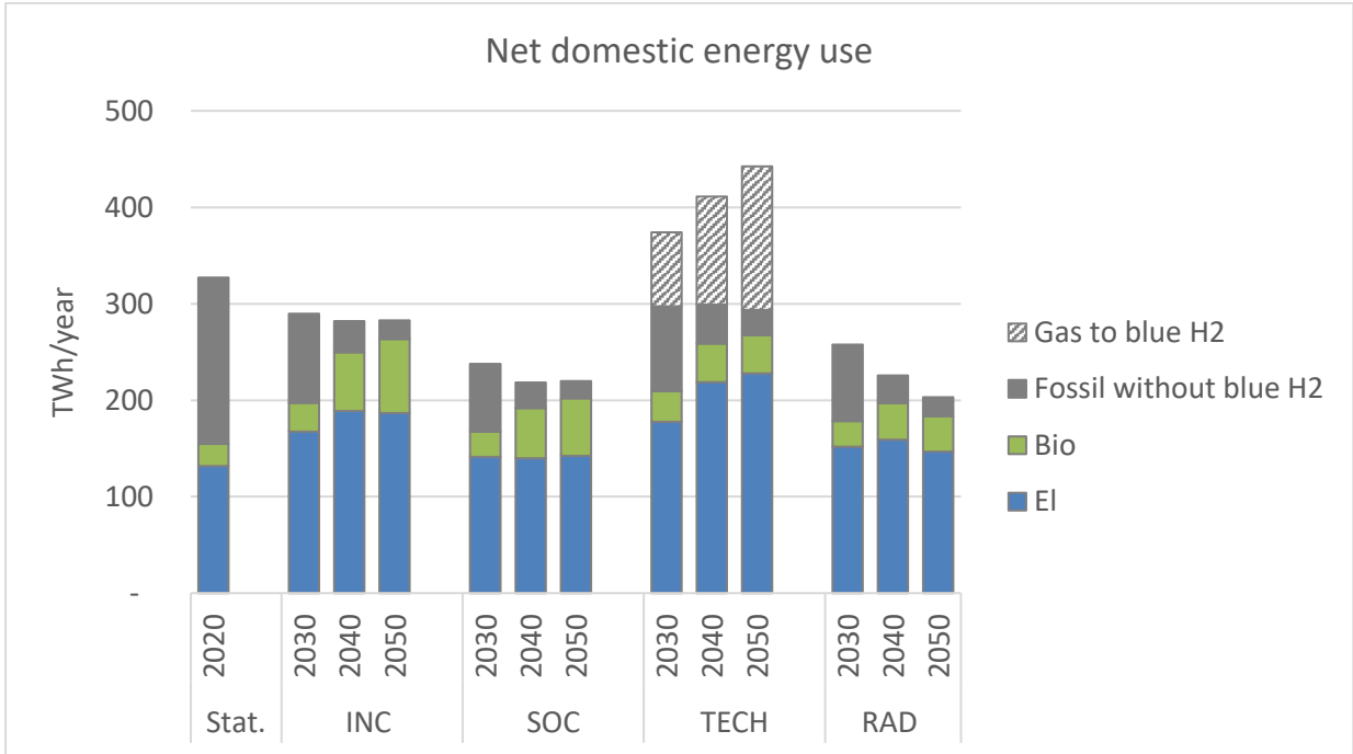
FIGURE 8: FINAL ENERGY USE BY ENERGY CARRIER (TWH/YEAR)
