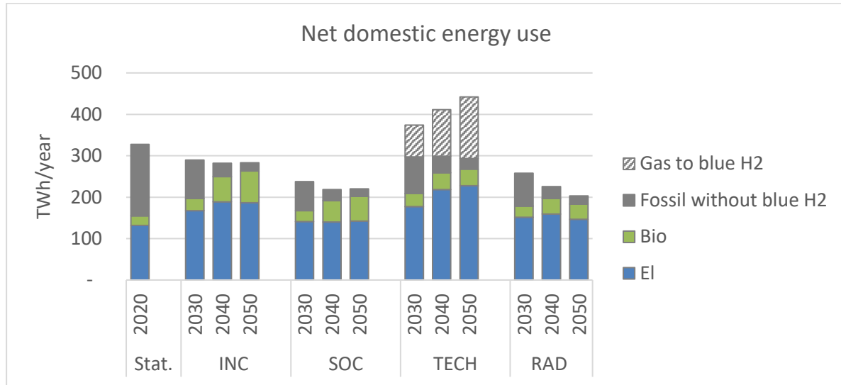
FIGURE III: FINAL ENERGY USE BY ENERGY CARRIER (TWH/YEAR)
