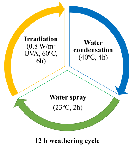
Fig. 3. Weathering cycle (1 cycle consists of 12 h).
