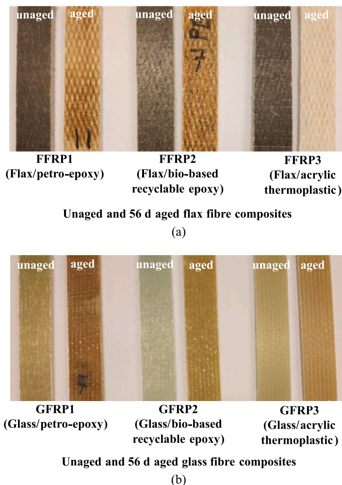
Fig. 8. Snapshots of test specimens after 56 d accelerated weathering: (a) unaged and 56 d aged flax fibre composites, and (b) unaged and 56 d aged glass fibre composites.
