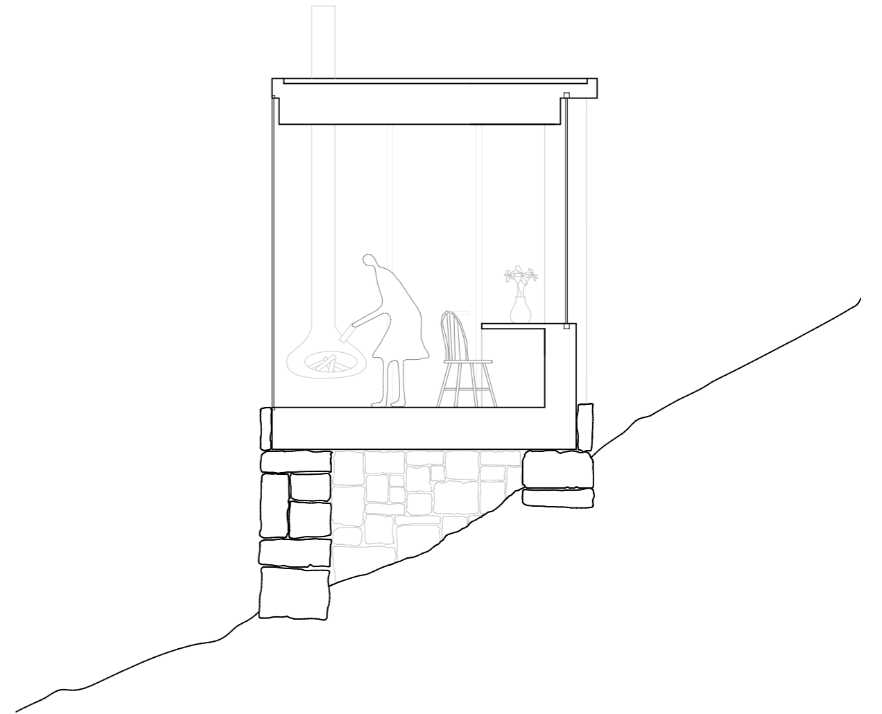
Snitt ss'
