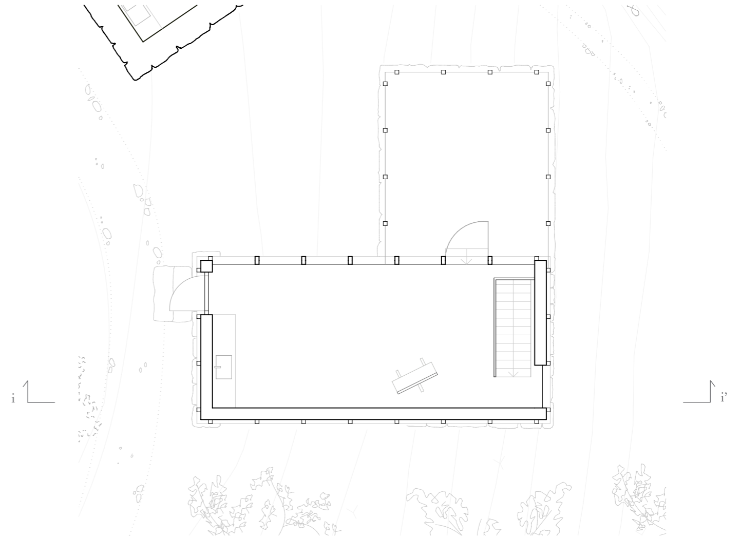
Plan 2. etg
