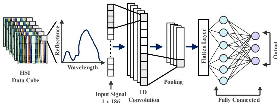
Figure 1: The architecture of 1D-CNN; typically comprises three fundamental layers: convolutional, pooling, and fully connected layer. Input from the HSI datacube (pixel value across wavelength) is fed to the convolutional layers, which apply a sliding window over given input data to perform feature extraction. The pooling layers reduce the size of the extracted features, and the fully connected layers classify the input based on the features obtained from the previous layers.
