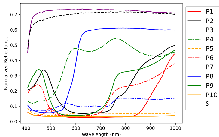
Figure D.1: Spectrum for ten pigments (P1 to P10) and substrate (S) measured at the flat surface by taking an average of 10 \times 10 pixels.
