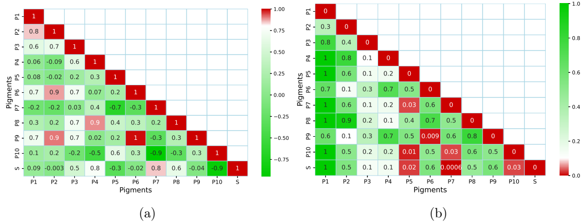
Figure 11: The matrices display the correlation and dissimilarity between the pigments; (a) Pearson’s correlation coefficient [83], a coefficient of 1 indicates a high correlation, while a value of zero represents no correlation; (b) SID calculated for dissimilarity, where a value of 0 implies a high degree of similarity between the spectra, while 1 indicates maximum dissimilarity.
