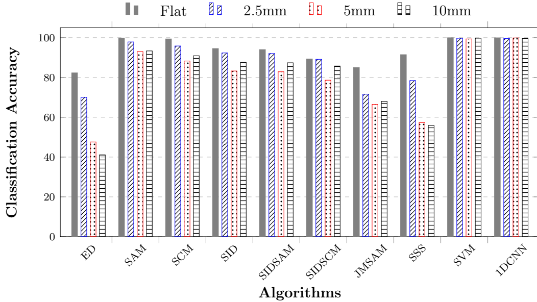
Figure E.8: Overall classification accuracy for four surface elevations (flat, 2.5mm, 5mm, and 10mm) obtained using average reference spectra; the averages were computed by considering a pixels values of a line drawn from right to left of the mockup for each pigment.
