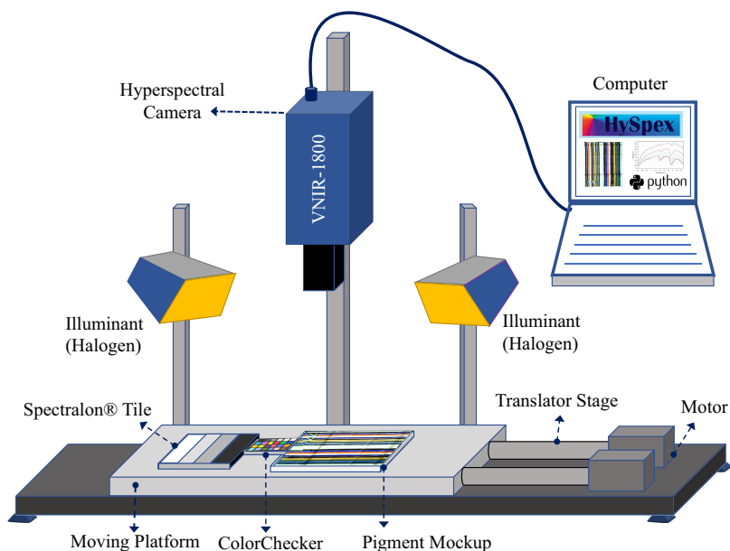
Figure 3: Schematic illustration of the HSI system used in the experiment. A 500 Watt halogen-based floodlight was used for illumination, and the illumination geometry was set to 45^{\circ} - 0^{\circ} - 45^{\circ} , where 0^{\circ} is the camera angle to normal.
