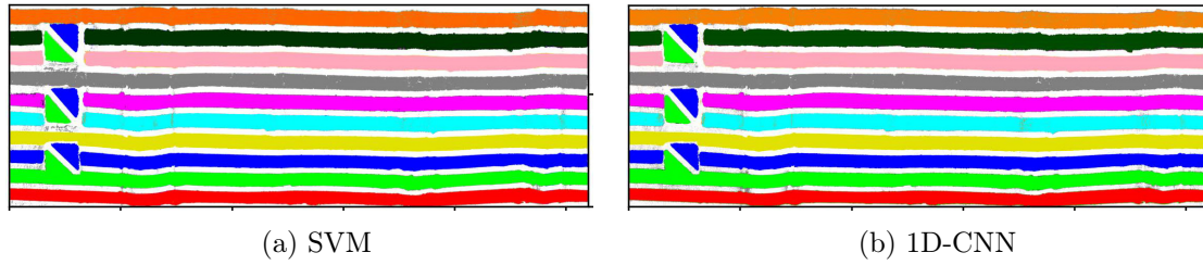
Figure F.1: The classification results for SVM and 1D-CNN using the averaged reference spectrum.
